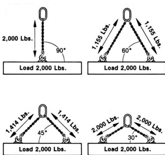
Fig. 1 — The load on each chain leg is increased as the lift angle decreases.
