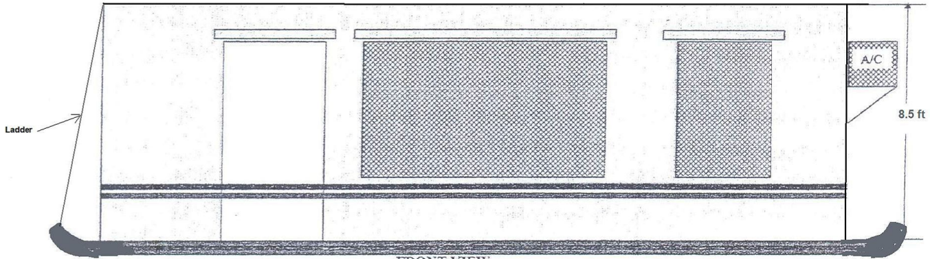
FRONT VIEW
