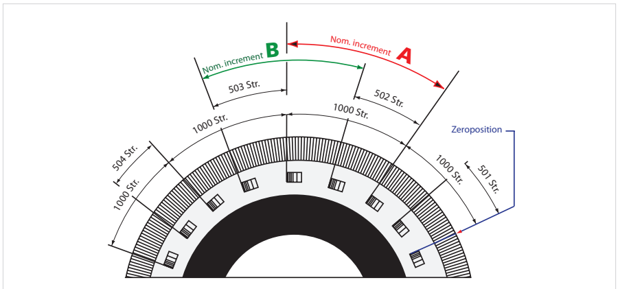
Figure 20 Circular graduations with increment-coded reference marks, rotary system
