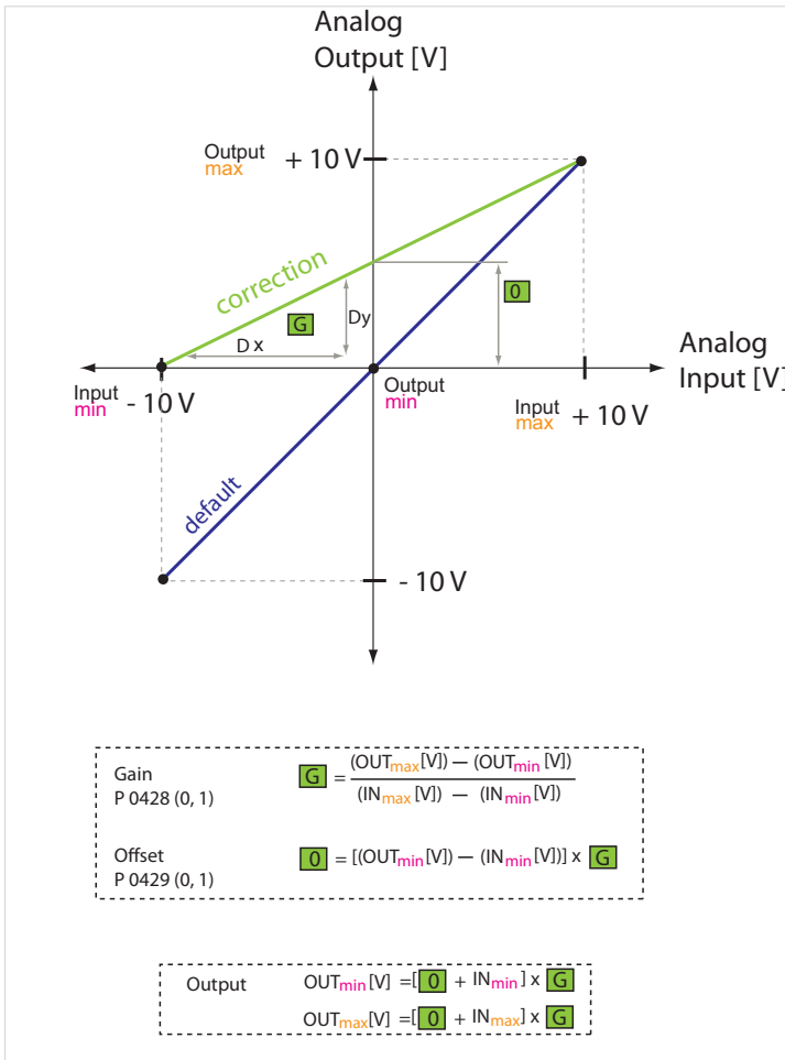
Figure 110 Weighting of analog inputs
