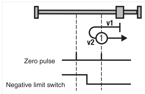
Figure 86 Type 1: Negative limit switch and zero pulseFigure pulse
