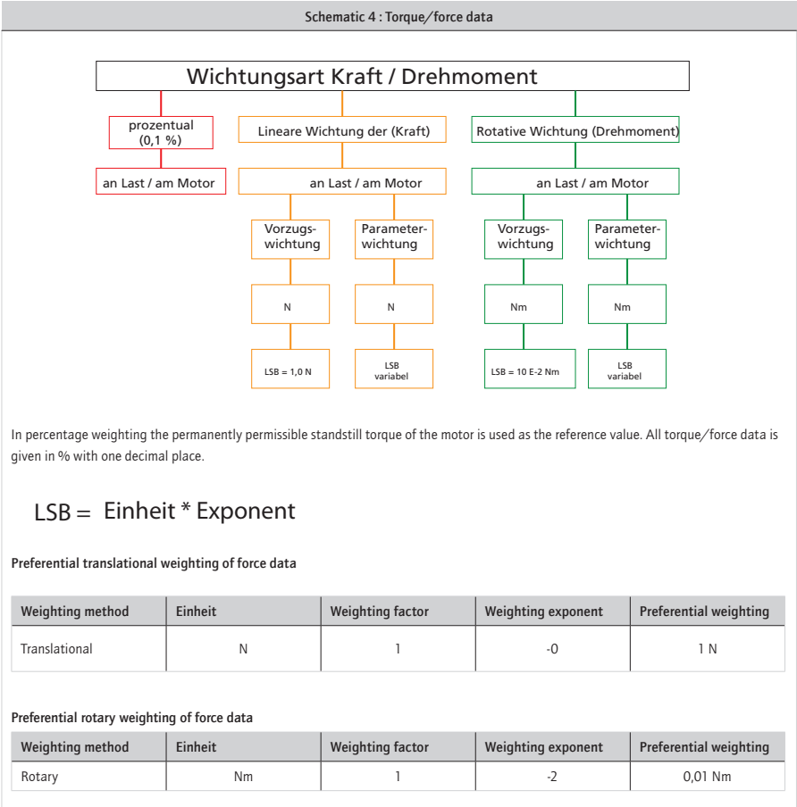
Figure 76 Weighting method for torque and force data
