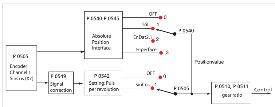
Figure 17 Encoder configuration based on example of channel 1
