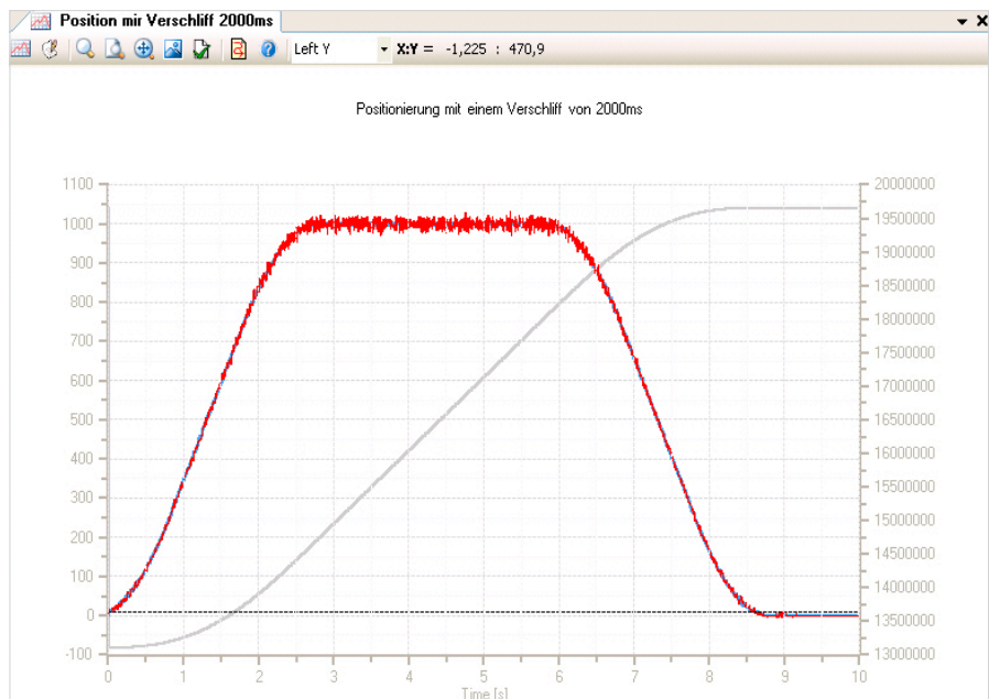
Figure 84 With smoothing of 2000 ms; Red = actual speed value; Grey = actual position value
