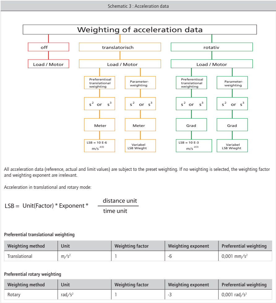
Figure 75 Weighting method for acceleration data
