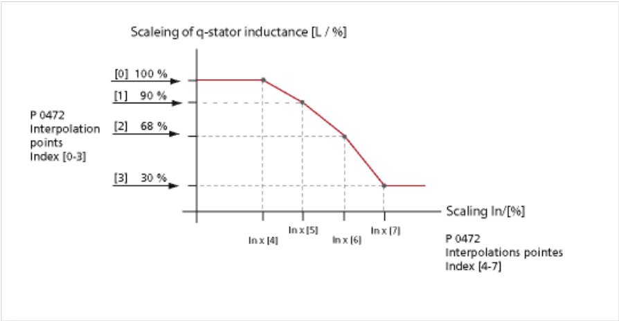
Figure 33 Example of current control adaptattion
