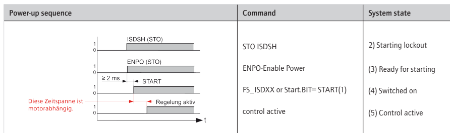
Figure 100 Power-up sequence for control
