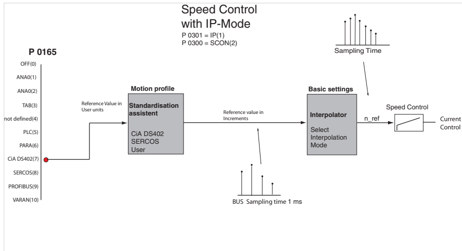
Figure 80 Speed control in IP mode
