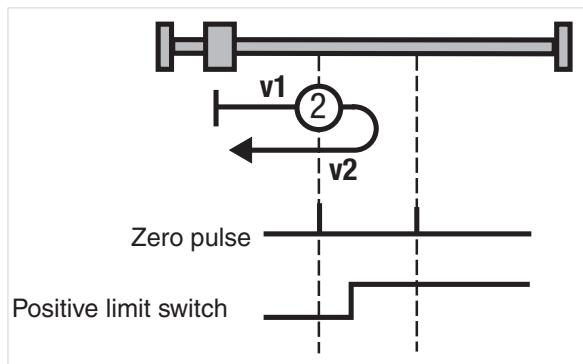
Figure 87 Type -2: Positive limit switch and zero pulse
