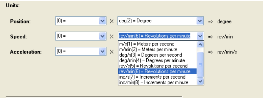
Figure 65 Scaling for position, speed, acceleration
