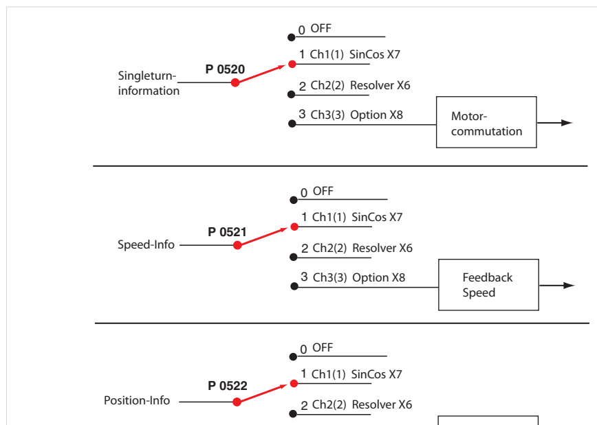
Figure 14 Interface configuration between encoder channels and control
