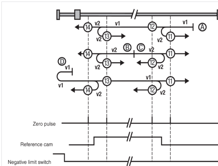
Figure 91 Type 11 to 14: Reference cam, zero pulse and negative limit switch
