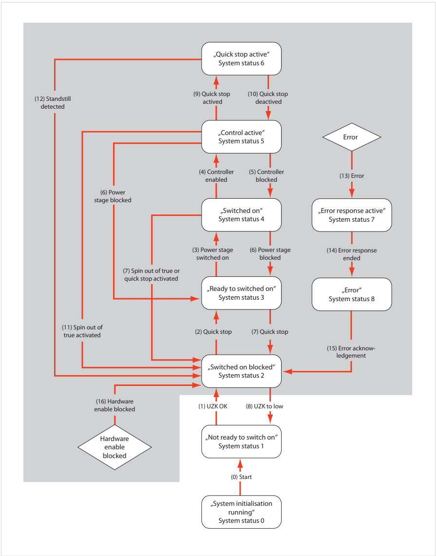
Figure 120 State machine of the drive controller
