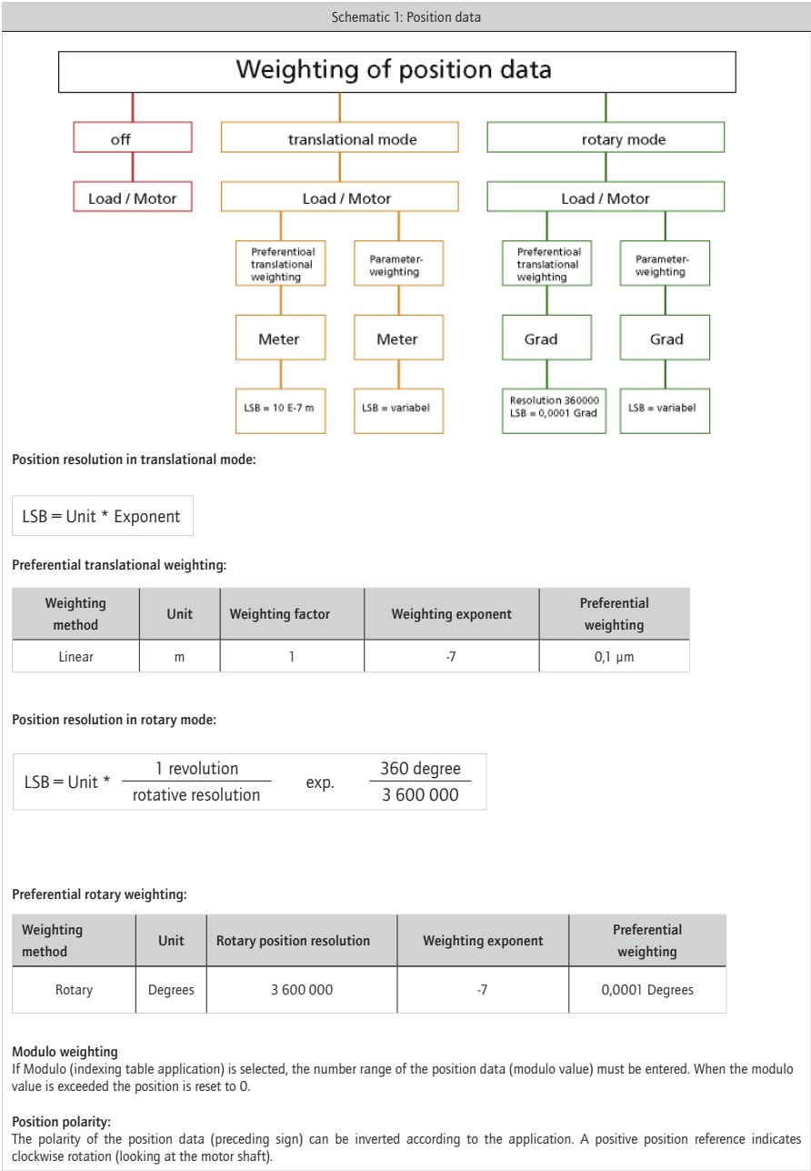
Figure 73 Position data weighting method
