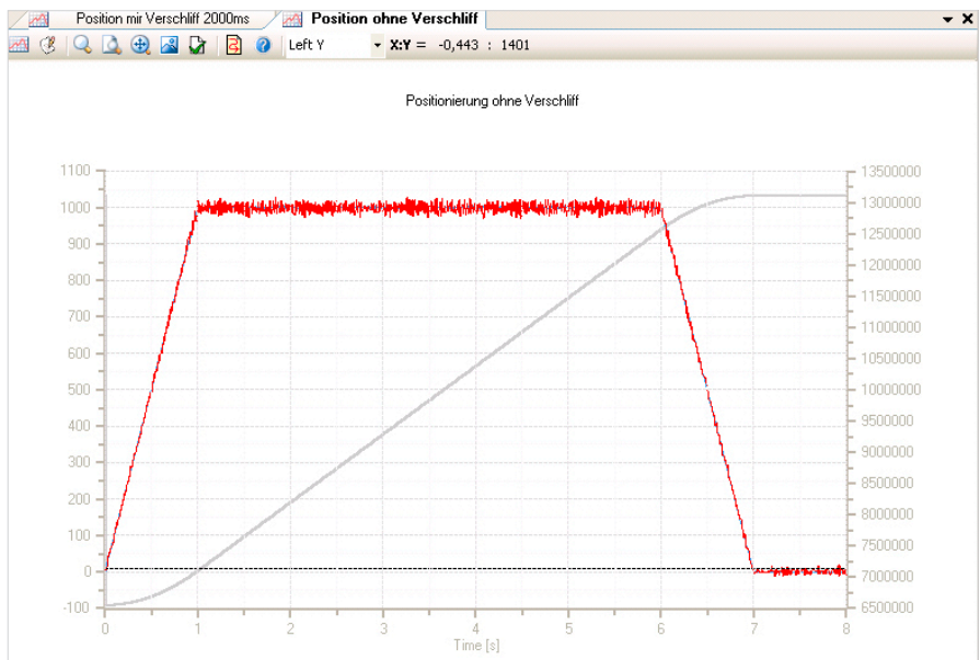
Figure 83 Without smoothing: Red = actual speed value; Grey = actual position
