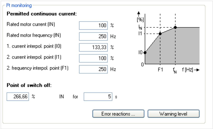
Figure 12 I 2 t protection PSM
