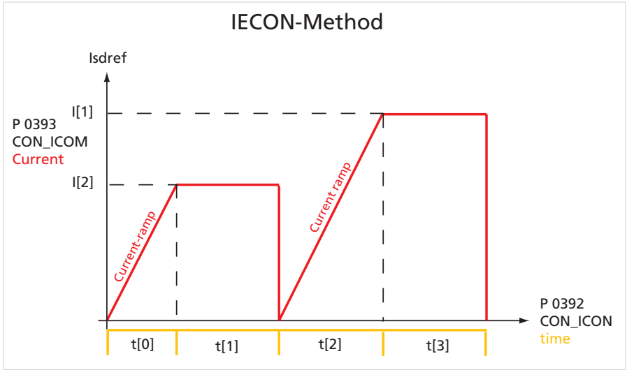
Figure 54 Schematic for the IENCC(1) and IECON(4) methods
