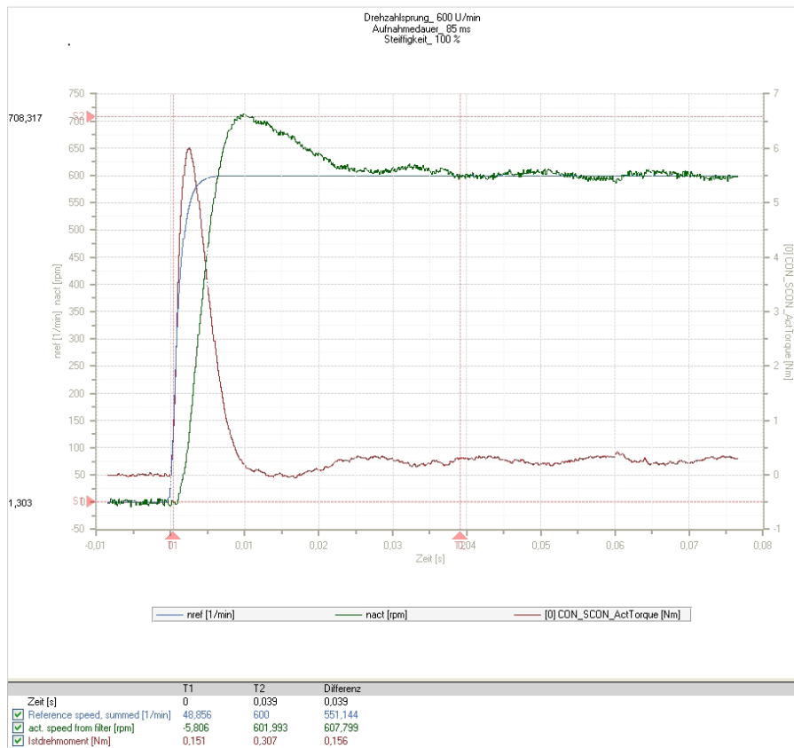
Figure 38 Speed step: 600 rpm
