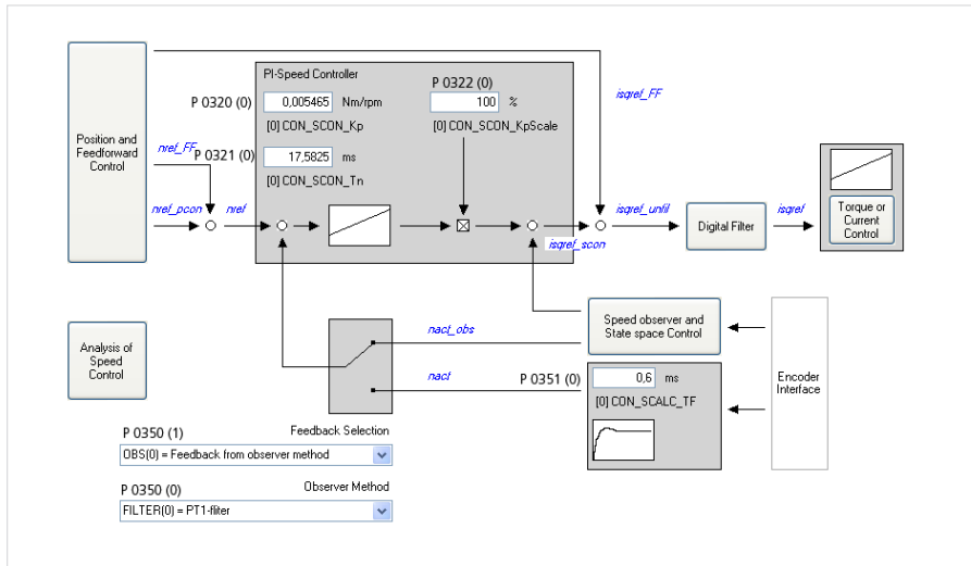
Figure 34 Speed controller screen
