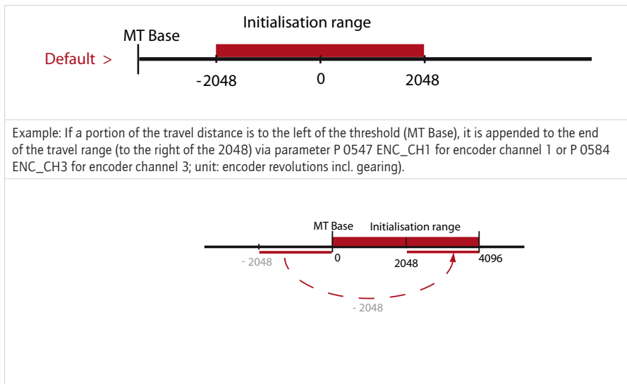
Figure 18 Overflow shift into the multitrans range
