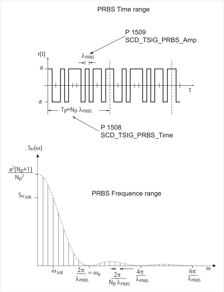
Figure 58 PRBS signal in time and frequency range
