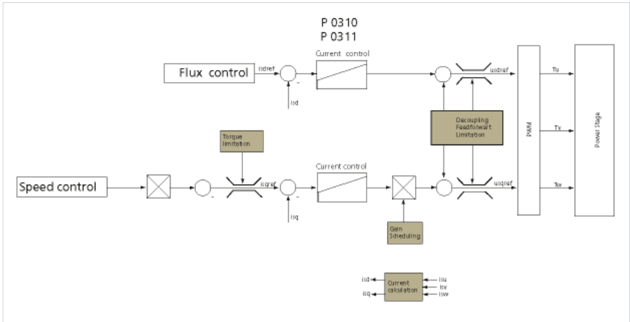
Figure 31 Block diagram of current and speed control
