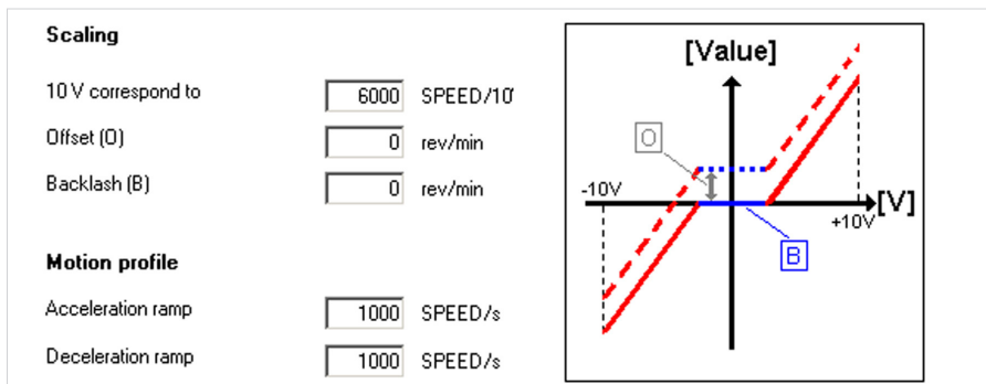
Figure 108 Options
