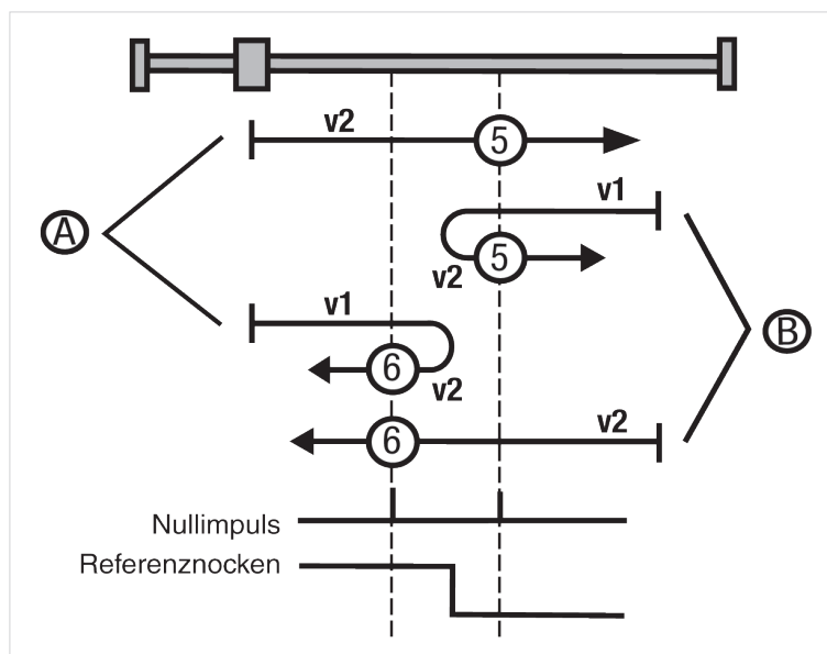
Figure 89 Type 5+6: Negative reference cam and zero pulse
