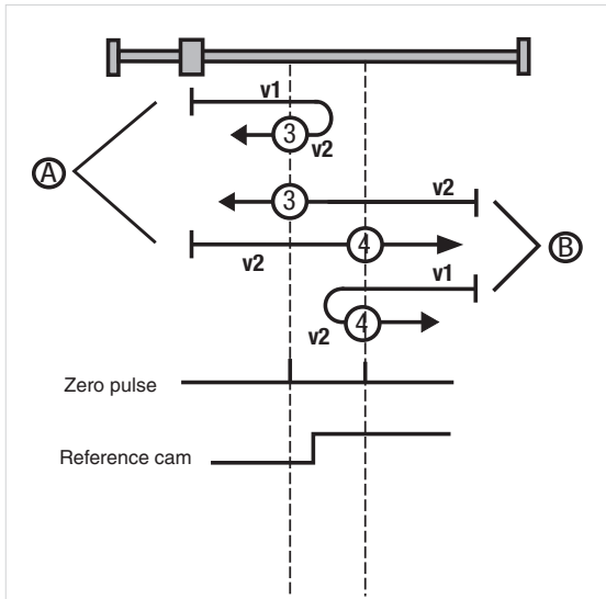
Figure 88 Type 3+4: Positive reference cam and zero pulse
