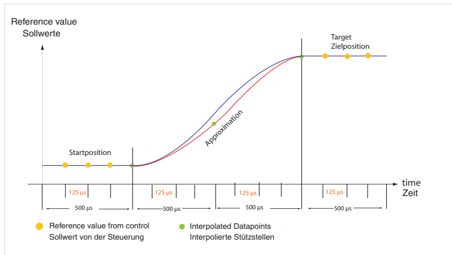
Figure 123 Cubic Spline Approximation: P 0305=125 \mu\text{s} cycle
