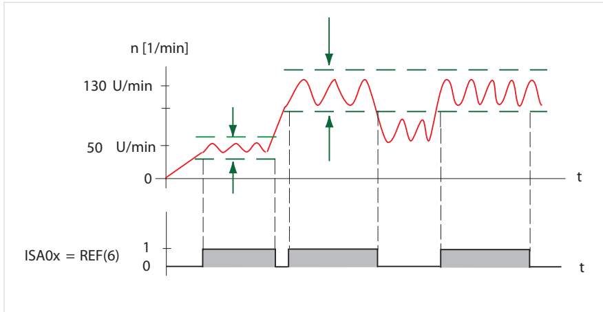
Figure 103 REF setting: "Reference reached" window for speed control via analog input
