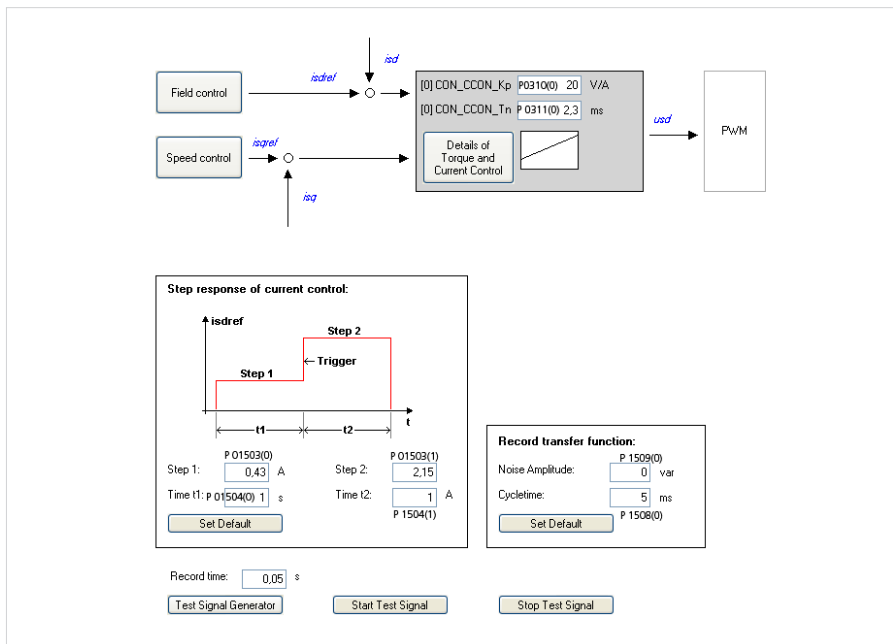
Figure 28 Screen for the current control loop
