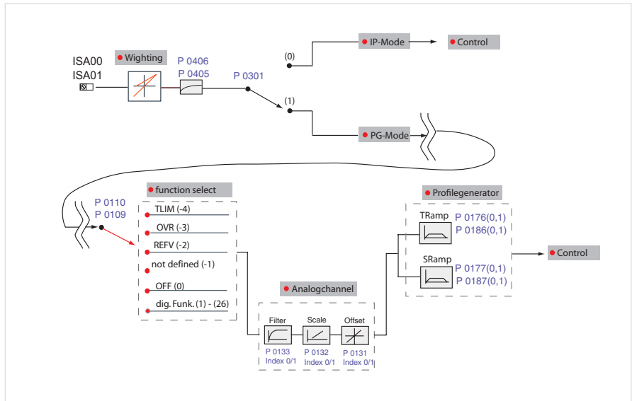
Figure 106 References via analog input (analog channel ISA00 and ISA01)
