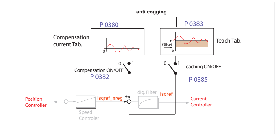
Figure 30 Schematic for detent torque compensation
