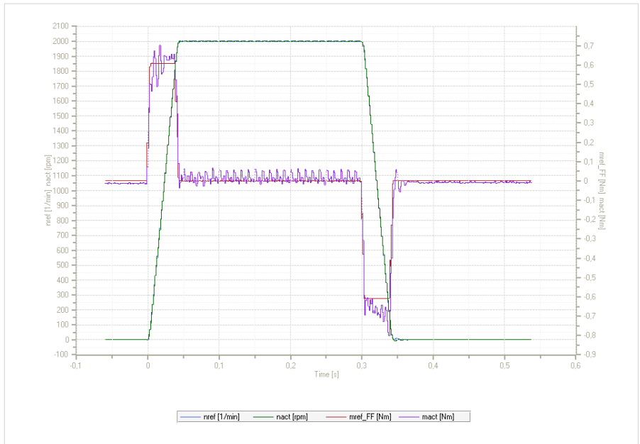
Figure 51 Graph of feedforward torque reference and actual torque value
