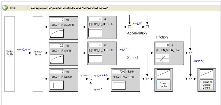
Figure 45 Position controller setup screen
