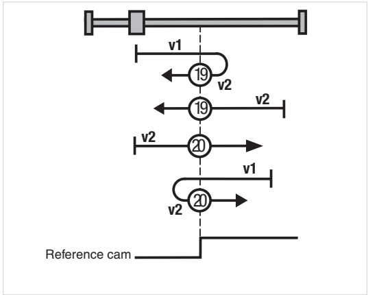
Figure 92 Type 17 to 30: Reference cam
