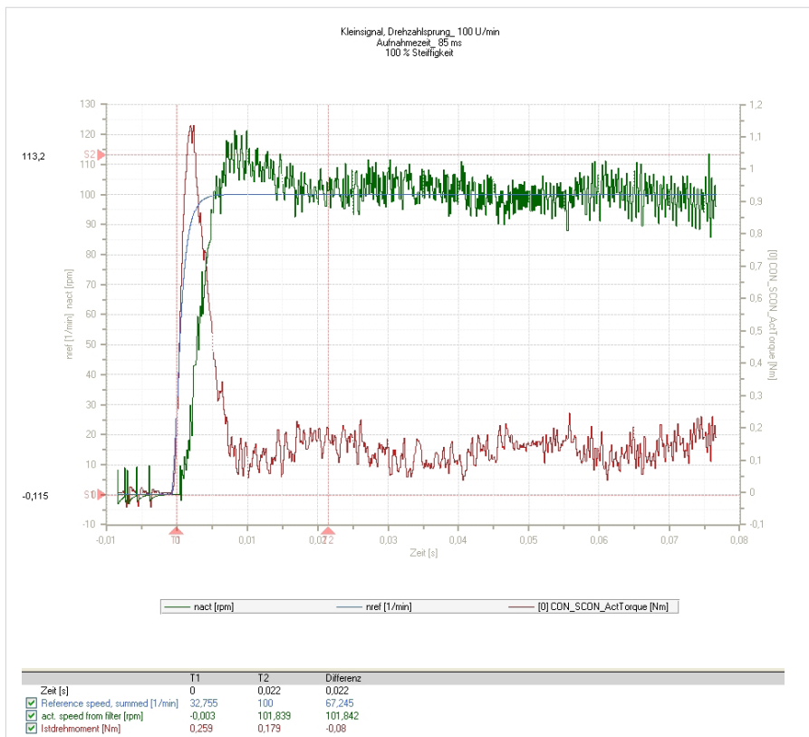
Figure 37 Small signal response: Speed step 100 rpm
