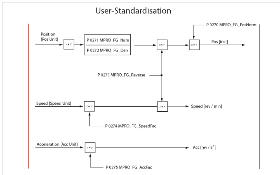
Figure 77 Schematic of user scaling
