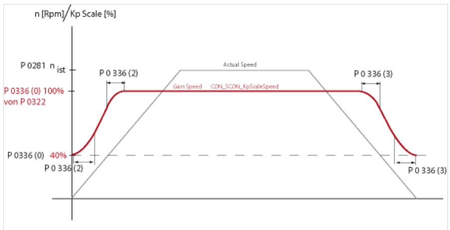
Figure 39 Speed controller gain reduction
