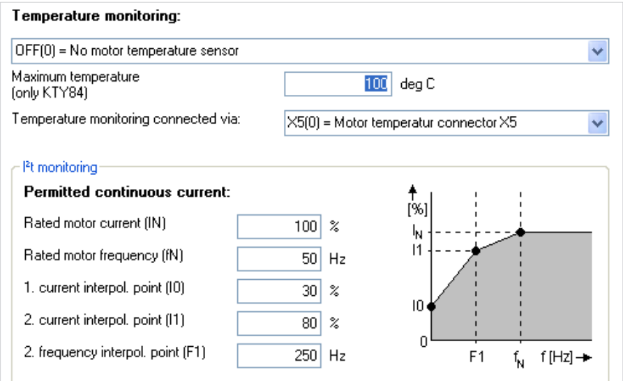
Figure 10 I²xt protection ASM
