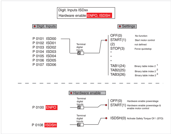
Figure 97 Function selector
