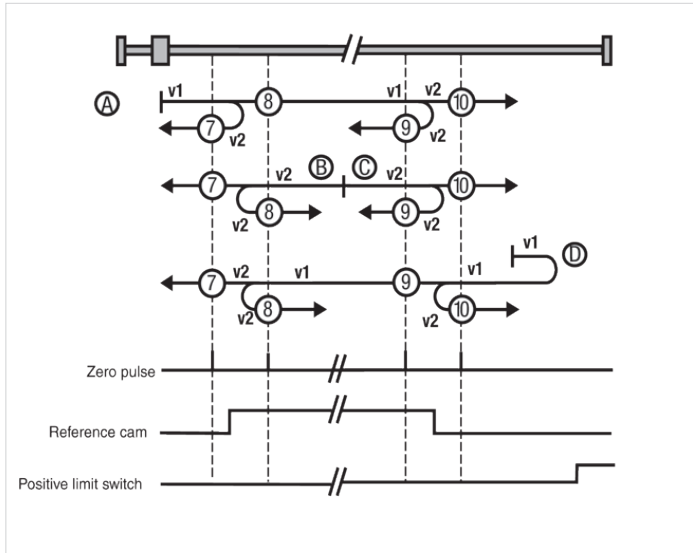
Figure 90 Type 7 to 10: Reference cam, zero pulse and positive limit switch
