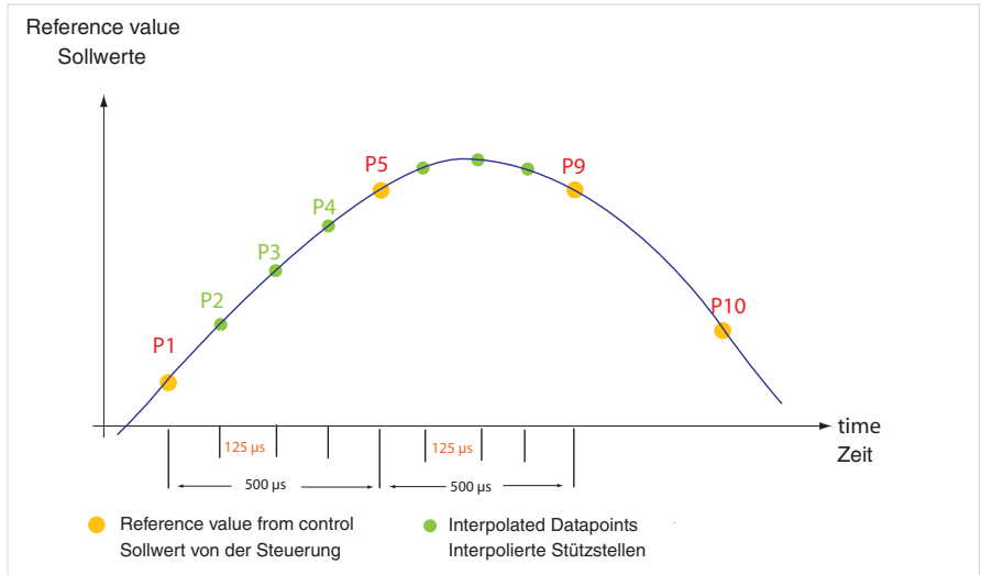
Figure 122 Cubic Spline interpolation; P 0305=125 \mu\text{s} cycle
