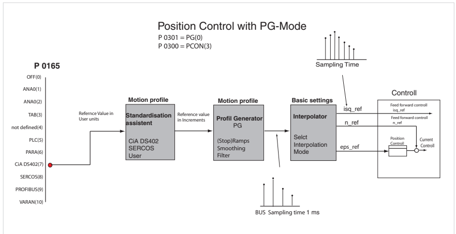
Figure 81 Configuration of position control in PG mode
