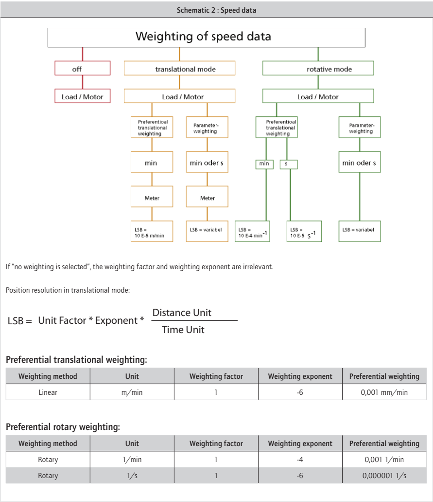
Figure 74 Weighting method for speed data
