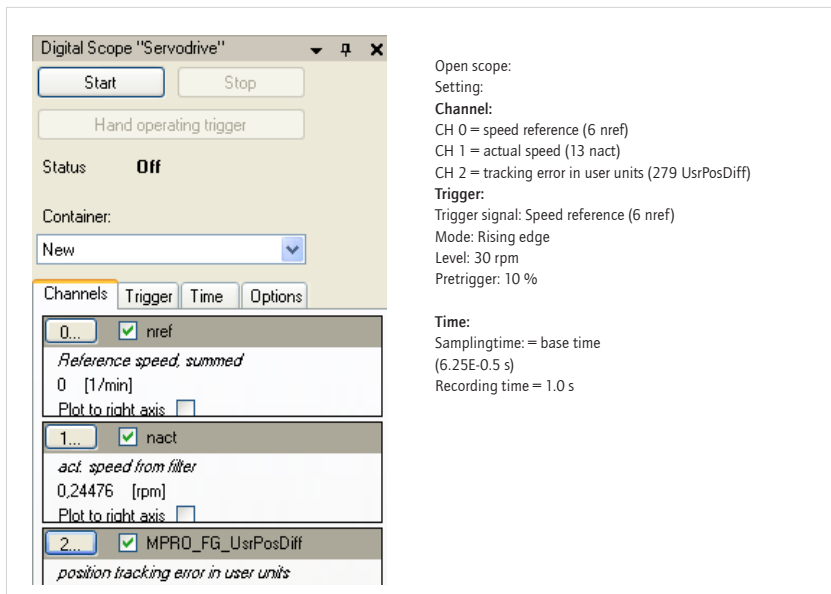
Figure 47 Oscilloscope settings.
