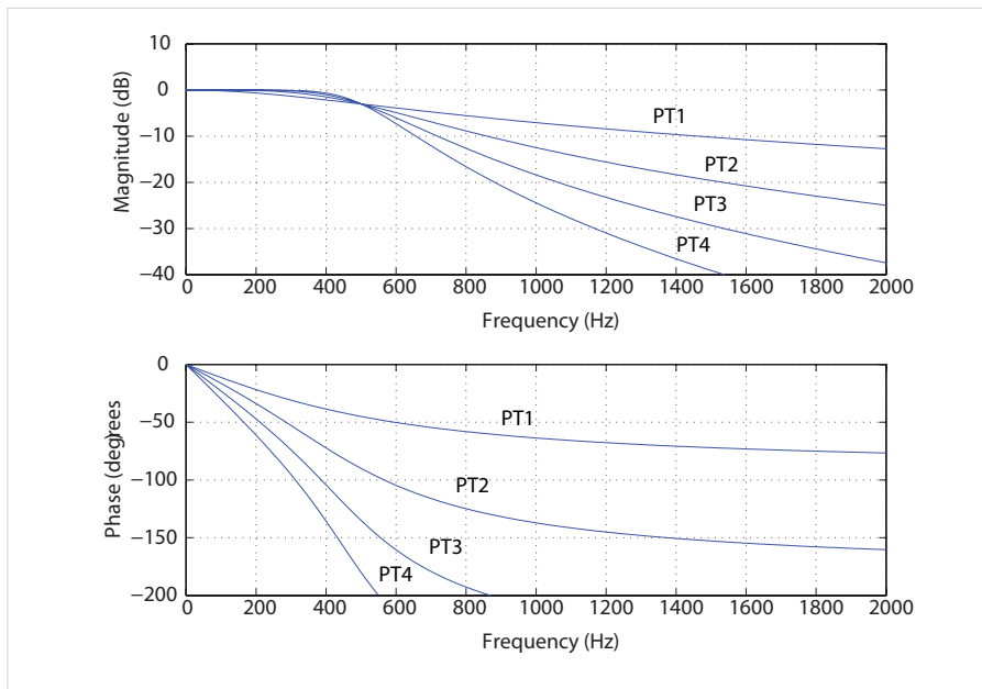
Figure 41 Frequency responses of PT1, PT2, PT3, PT4 filters
