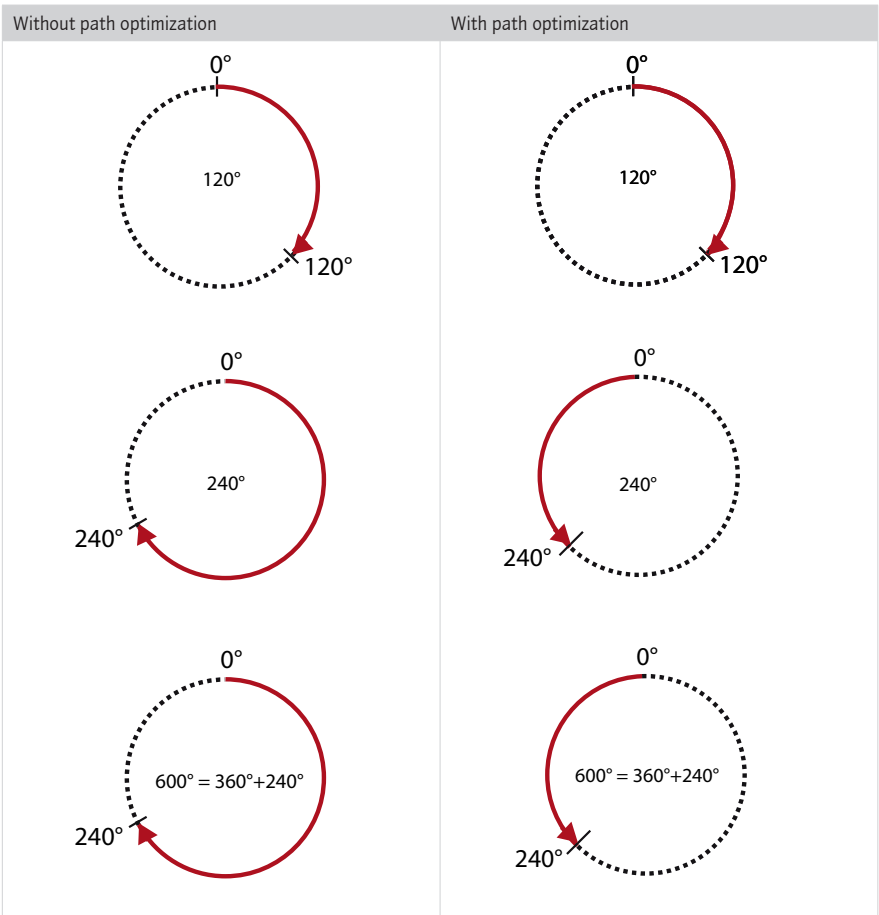
Figure 71 Path optimization
