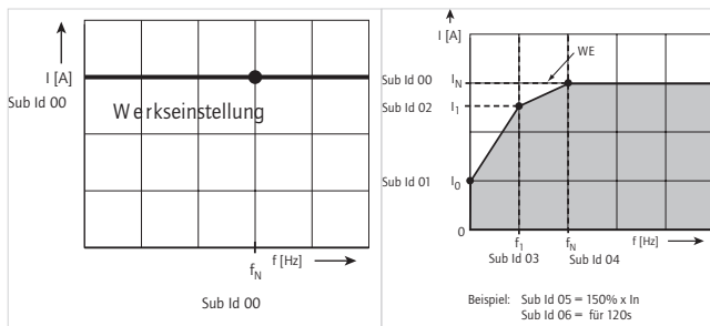
Figure 11 Figure left: Constant characteristic/ Figure right: Characteristic with interpolation points
