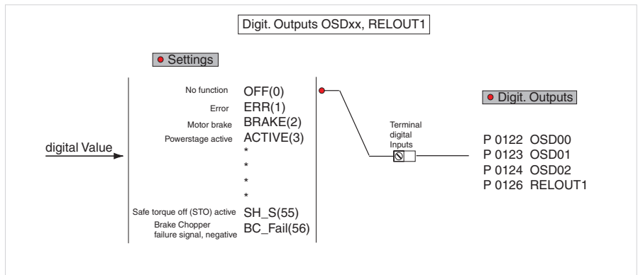
Figure 101 Function block for adaptation of the digital outputs
