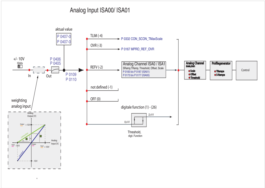
Figure 109 Analog inputs function block, PG/IP switching, Analog channel and Weighting
