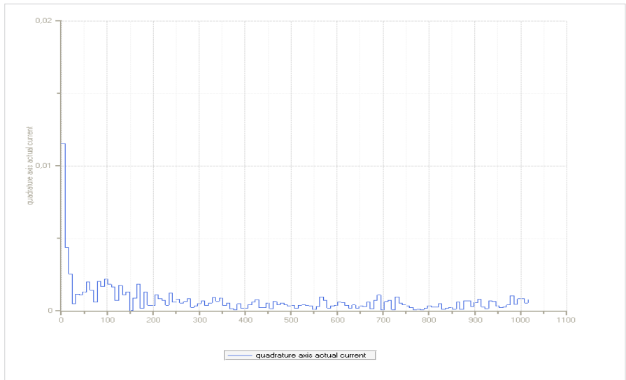
Figure 44 Motor shaft under current at standstill with activated notch filter (width f = 40\text{ Hz} , mid-frequency f = 420\text{ Hz} )
