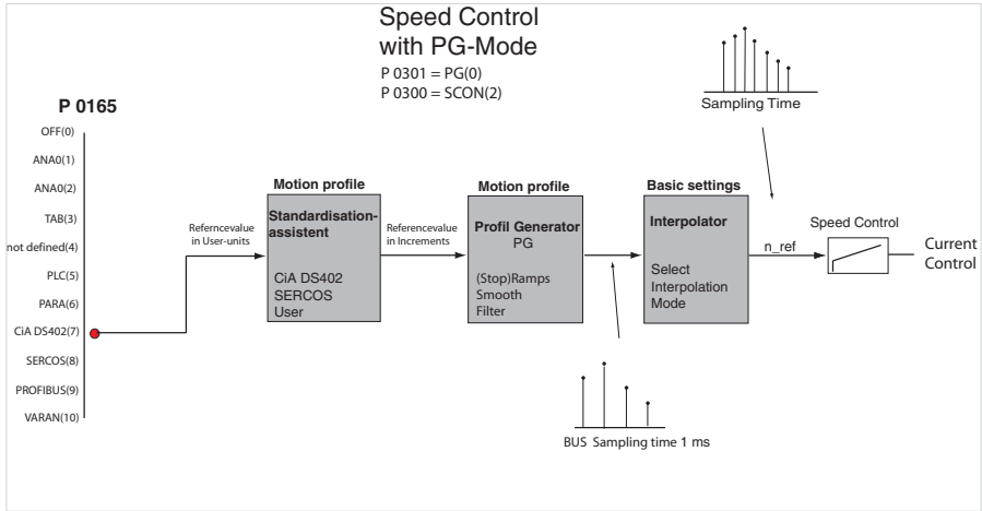
Figure 79 Speed control in PG mode
