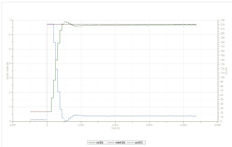
Figure 29 Step up to rated current
