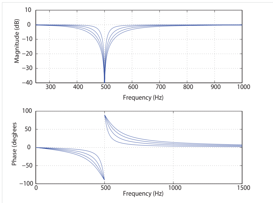
Figure 42 Notch filter: Blocking frequency 500 Hz and bandwidths 25, 50, 75 and 100 Hz
