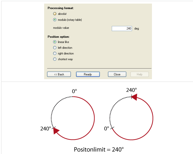
Figure 68 Defining the position range
