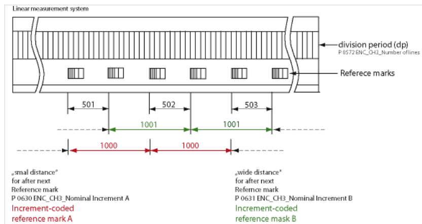
Figure 21 Schematic view of a linear scale with increment-coded reference marks
