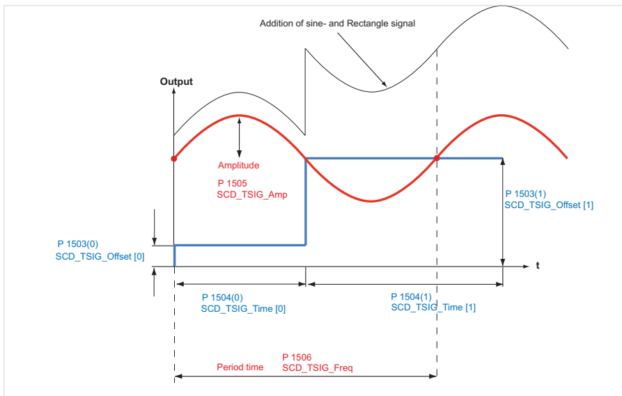
Figure 57 Addition of sine- and rectangle signal
