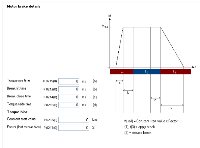
Figure 104 Brake output
