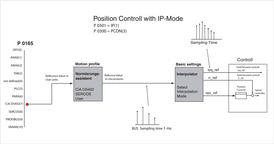
Figure 82 Position control in IP mode
