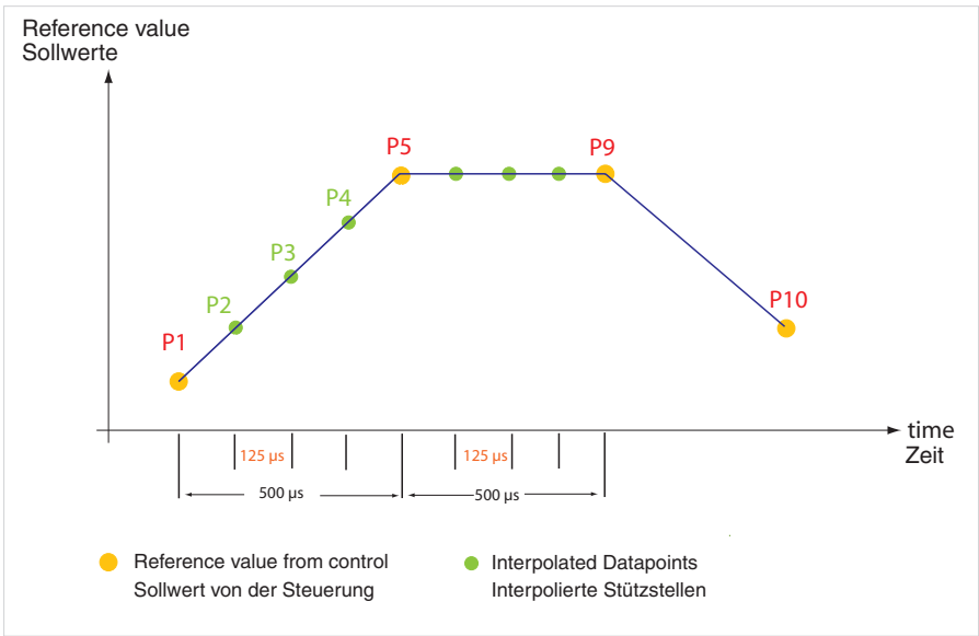
Figure 121 Linear interpolation
