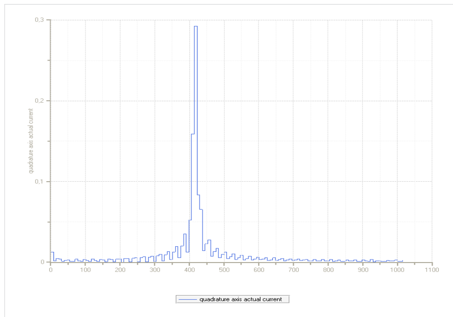
Figure 43 Oscillation of a motor shaft under current at standstill without filter
