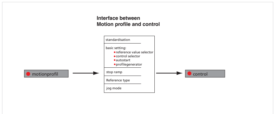
Figure 62 Reference interface
