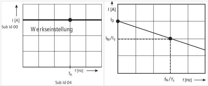
Figure 13 Characteristic of PSM
