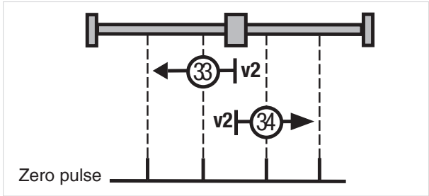
Figure 93 Type 33 + 34: Zero pulse
