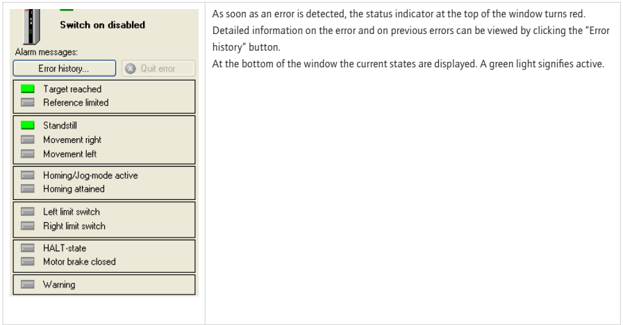
Figure 118 Drive status-Fenster
