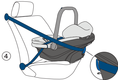
Picture 3+4: Pull the cars diagonal seat belt over the head protection (3) of First Class 0+ and attach it into the blue clip on the back of the car seat.
