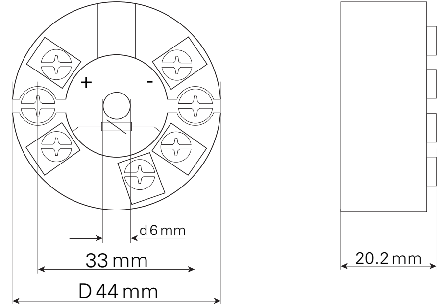
Figure 1-5 Mechanical Specifications
