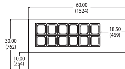
VUR-60-12 TOP VIEW
