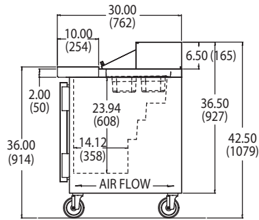
VUR-60-8, VUR-60-12, VUR-60-16 SIDE VIEW
