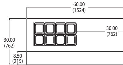
VUR-60-8 TOP VIEW
