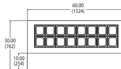
VUR-60-16 TOP VIEW
