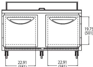
VUR-60-16 FRONT VIEW
