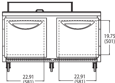
VUR-60-12 FRONT VIEW
