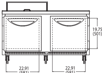
VUR-60-8 FRONT VIEW
