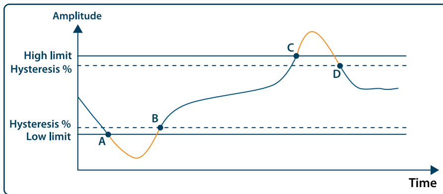
Figure 3-4 Alarm Example
