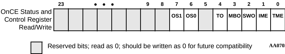
Figure 11-5 OnCE Status and Control Register (OSCR)
