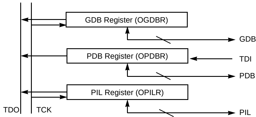
Figure 11-9 OnCE Pipeline Information and GDB Registers
