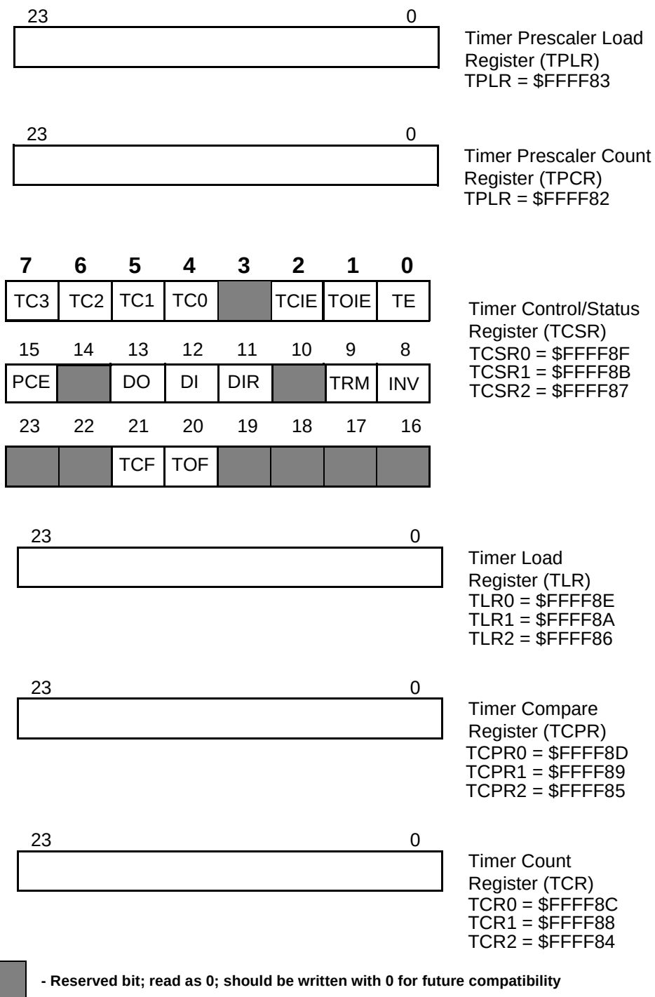
Figure 9-3 Timer Module Programmer's Model
