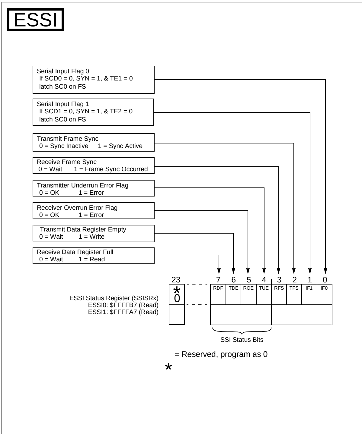
Figure E-13 ESSI Status Register (SSISR)
