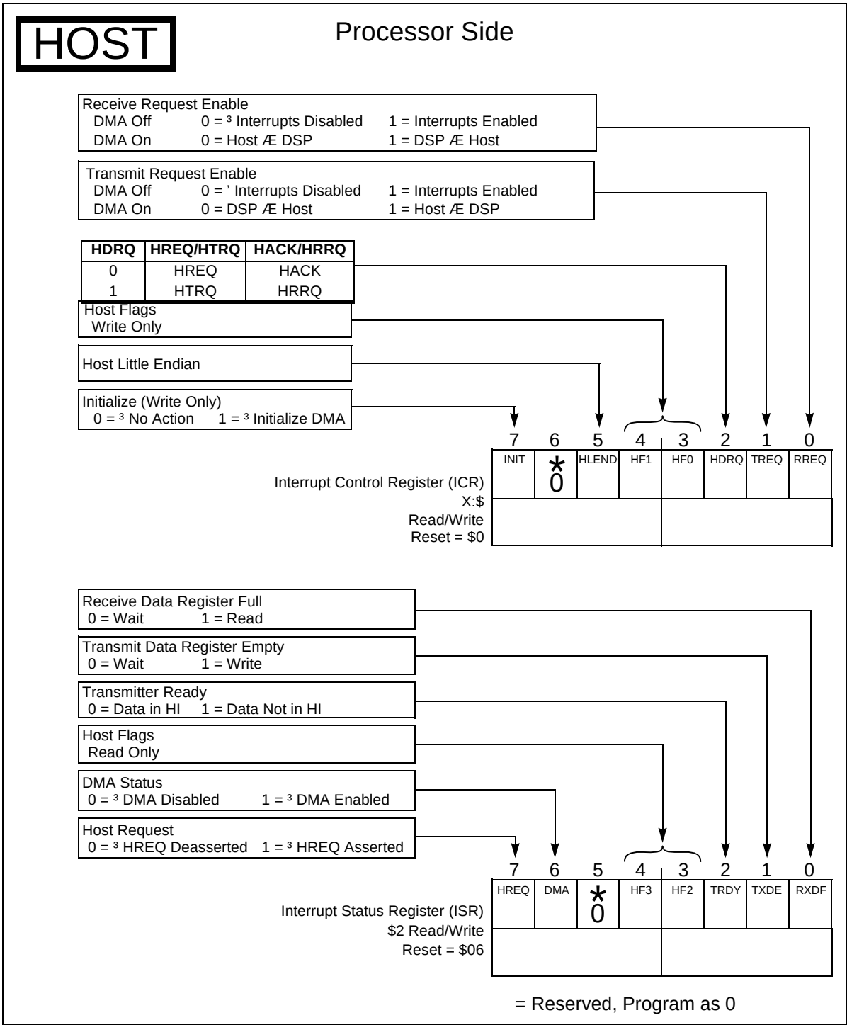
Figure E-8 Interrupt Control and Interrupt Status Registers
