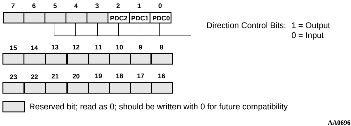
Figure 8-9 Port E Direction Register (PRRE)
