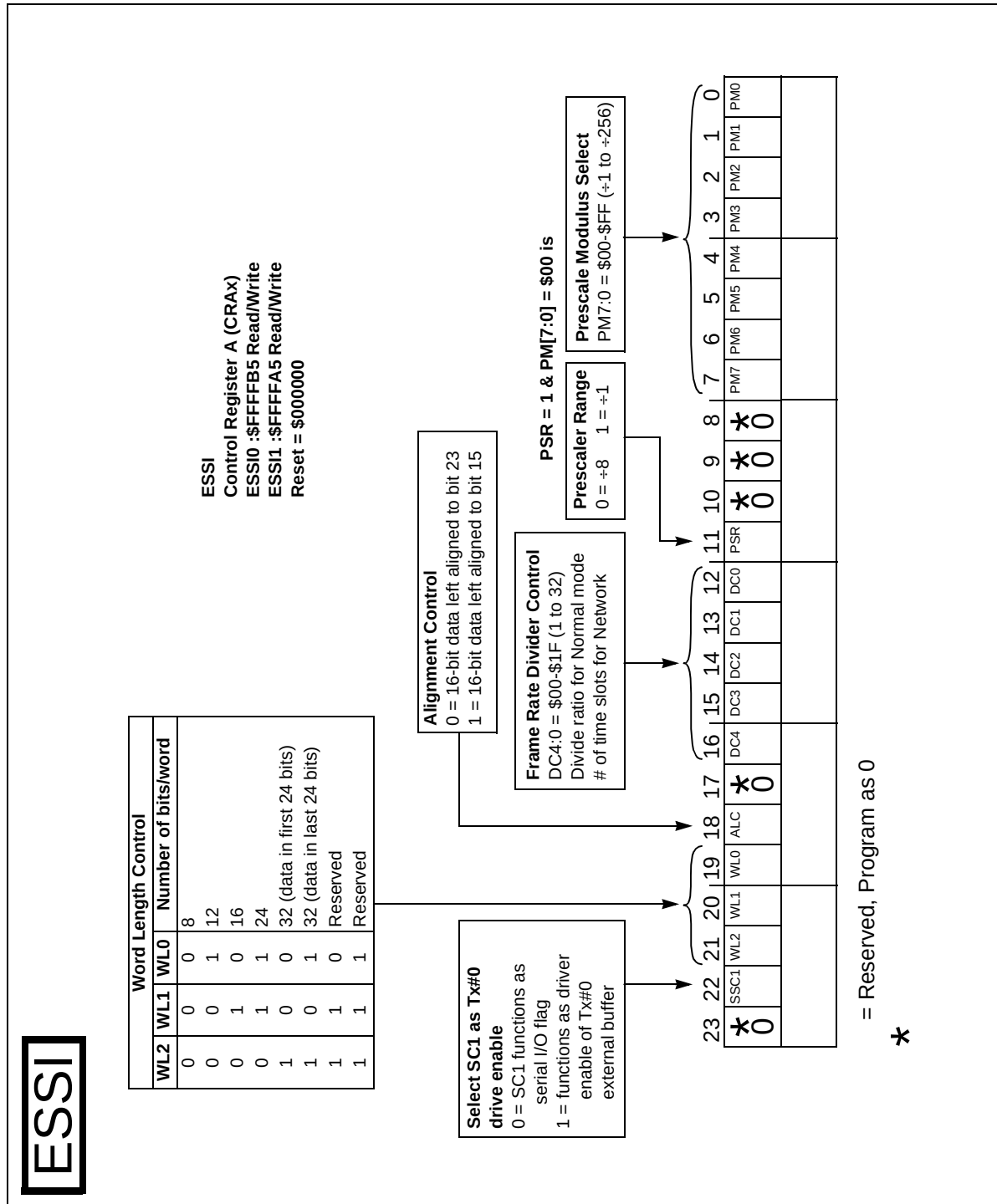
Figure E-11 ESSI Control Register A (CRA)
