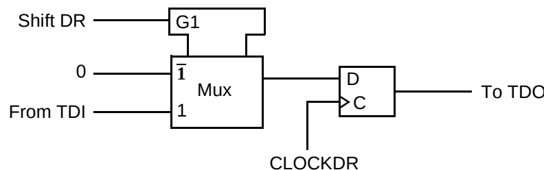
Figure 12-5 BYPASS Register
