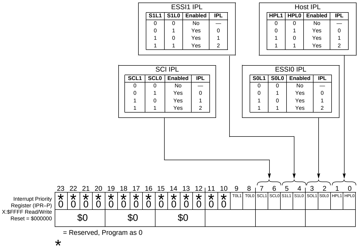
Figure E-3 Interrupt Priority Register – Peripherals (IPR-P)
