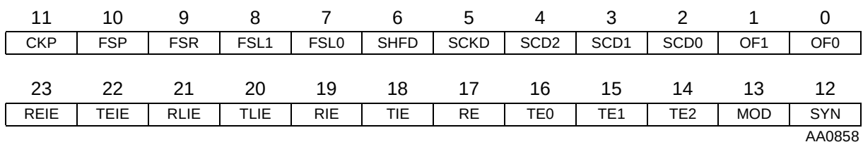
Figure 7-3 ESSI Control Register B (CRB) (ESSI0 X:$FFFFB6, ESSI1 X:$FFFA6)
