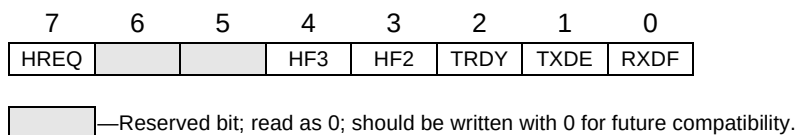
Figure 6-14 Interface Status Register
