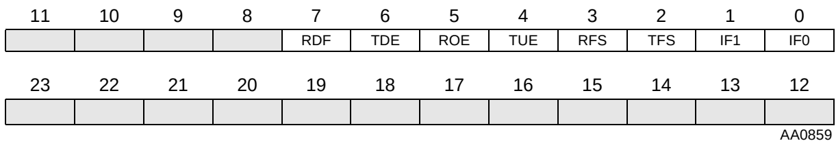
Figure 7-4 ESSI Status Register (SSISR) (ESSI0 X:$FFFFB7, ESSI1 X:$FFFA7)
