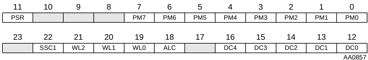
Figure 7-2 ESSI Control Register A (CRA) (ESSI0 X:$FFFFB5, ESSI1 X:$FFFA5)
