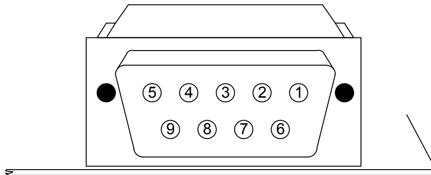
Figure 3-1: EDOSK Serial Port Pin Numbering
