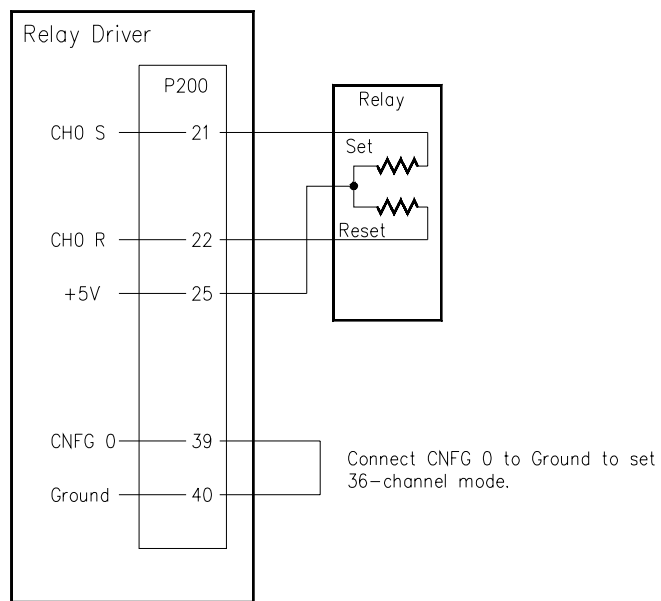
Figure 3-2. Example: Closing a Channel (36-Channel Mode)
