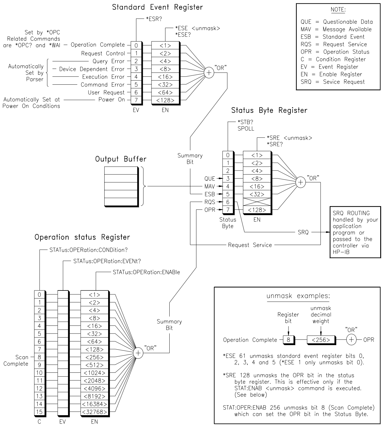
Figure 5-1. Relay Driver Module Status System Register Diagram
