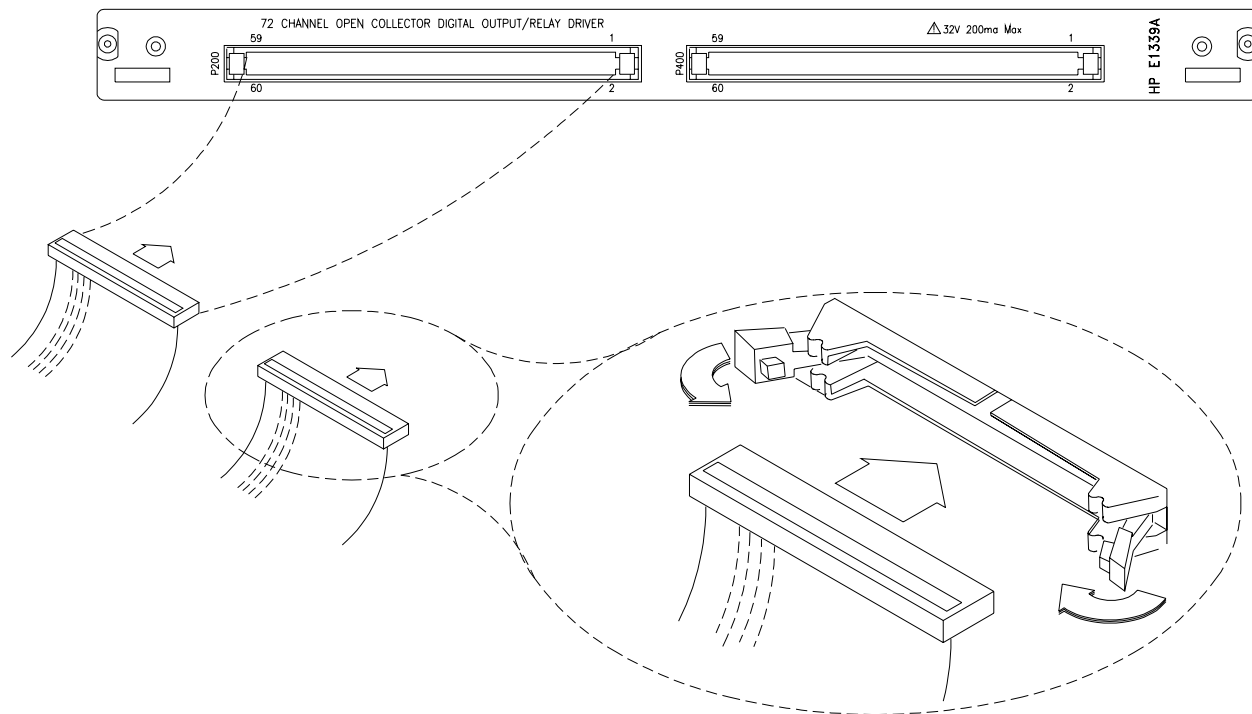
Figure 2-1. Connecting User Inputs
