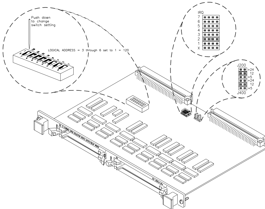
Figure 2-2. Switch/Jumper Locations
