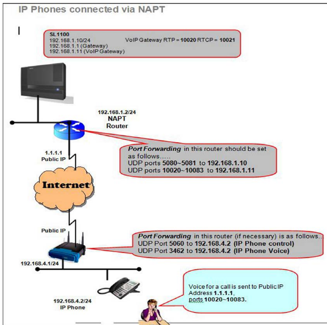
Figure 9-36 NATP Configuration Example
