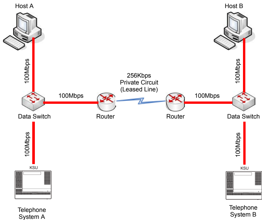
Figure 6-4 Voice and Data Network Implementation
