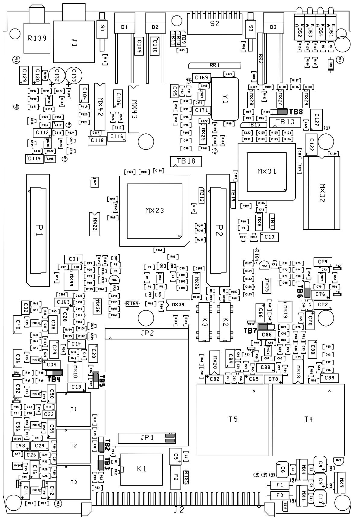
Figure 6: Audio board configuration
