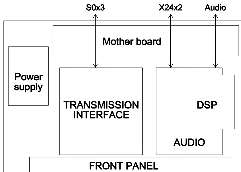
Figure 4: Internal architecture of the HIFISCOOP 3 5ASystem
