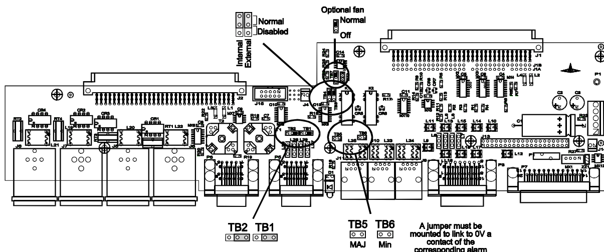
Figure 5: Motherboard configuration
