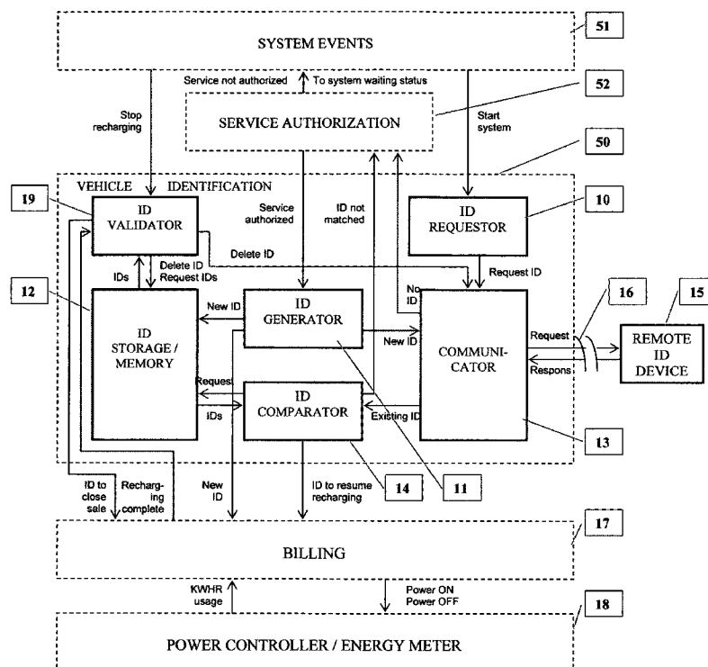
Vehicle Identification System Functional Diagram
