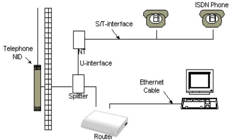
Figure 2-4.3 Router Connected through a ISDN Splitter
