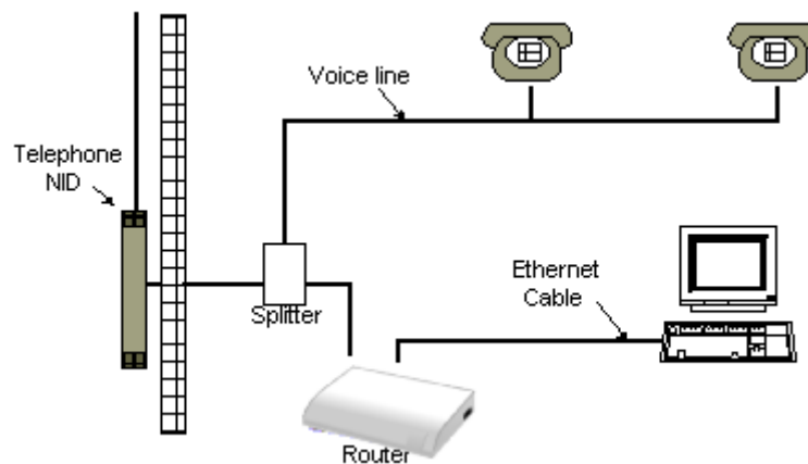
Figure 2-4.1 Router Connected through a POTS Splitter
