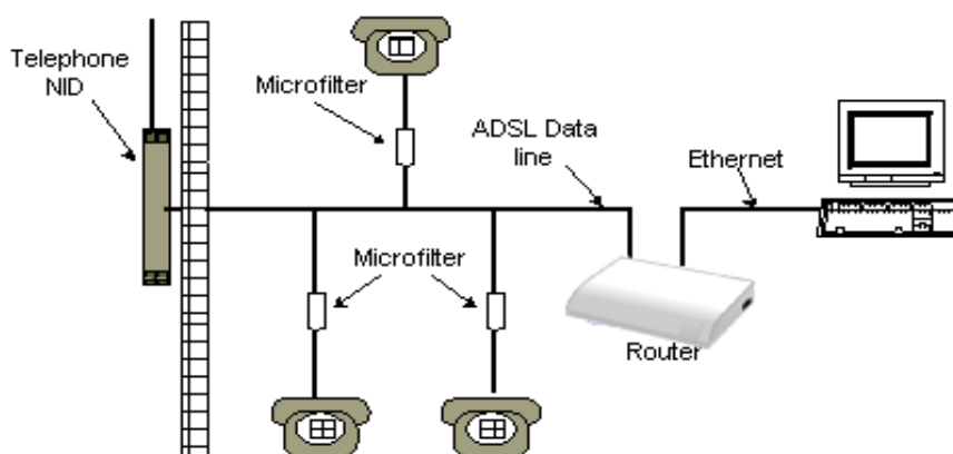
Figure 2-4.2 Router Connected through several micro-filters
