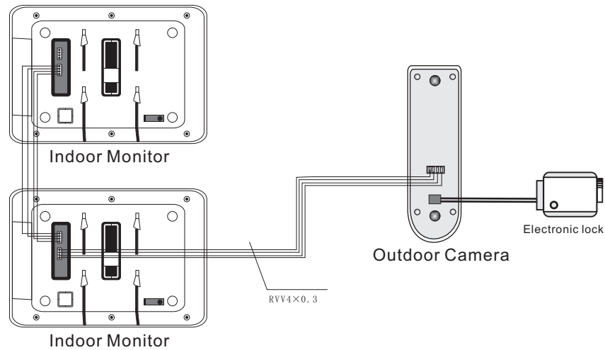
"Two Cam. to one Mon." wiring diagram (Pic. 4)
