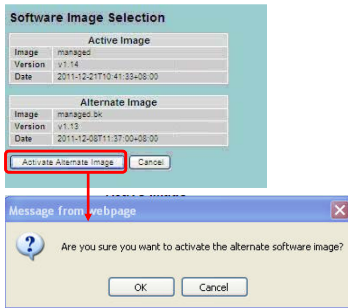
Figure 5-2.2: The Firmware Selection
