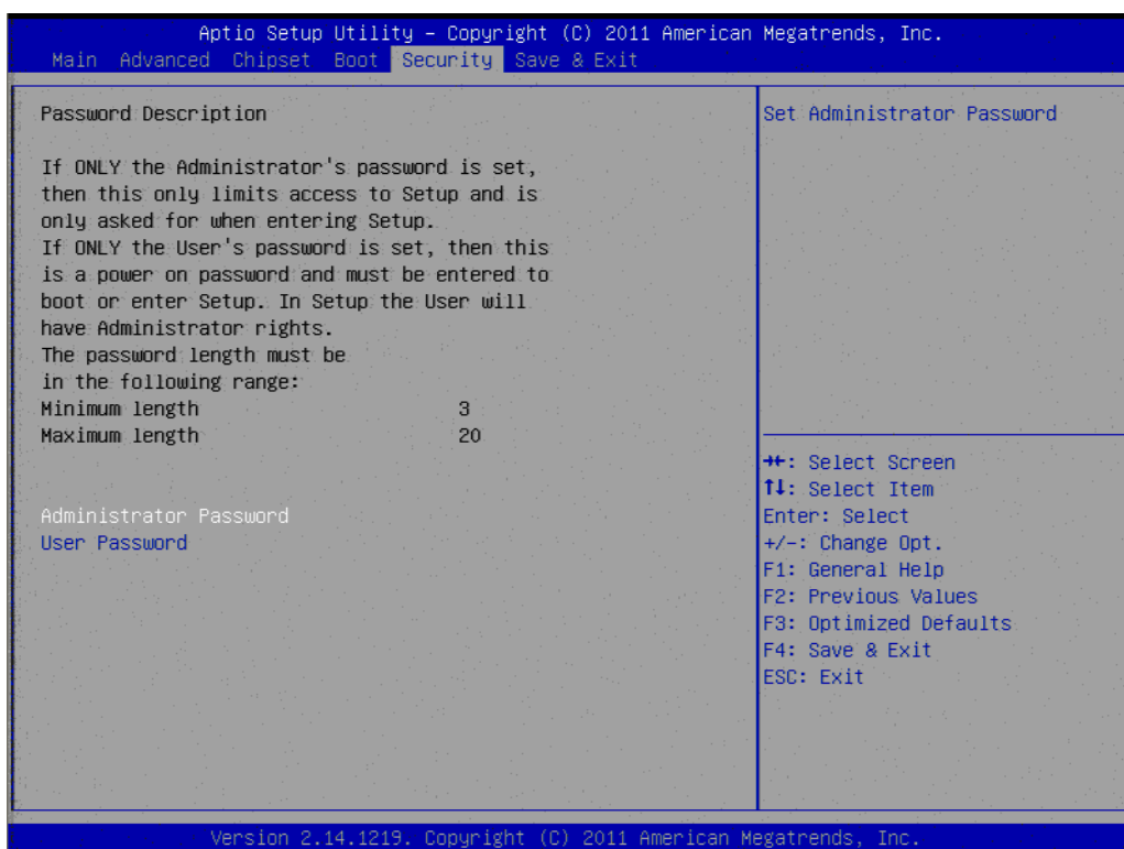
Figure 3.17 Security Setup
