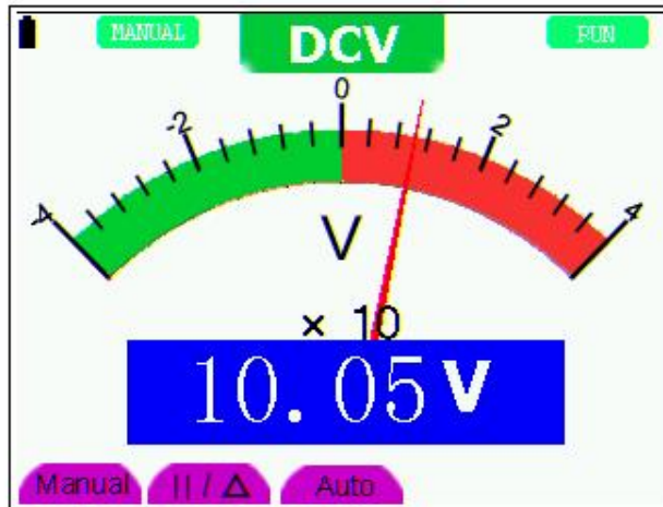
figure 33: Automatic/Manual Range Adjustment
