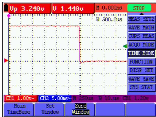
figure 48: Window Setting
