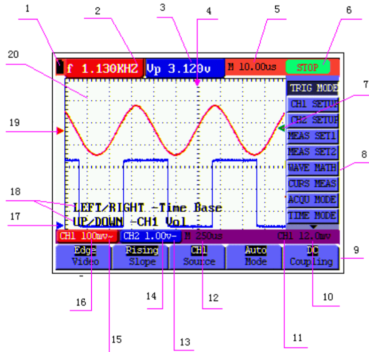
figure 4: Oscilloscope Operation Window
