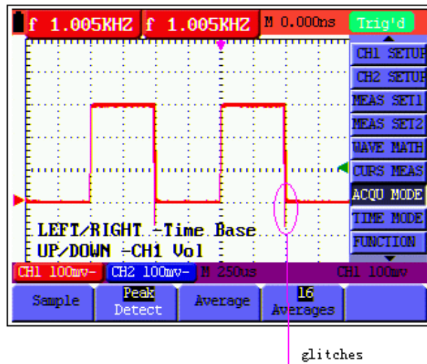
figure 16: Peak Detection
