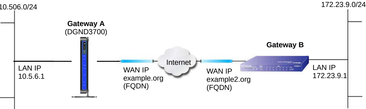
Figure 63. VPNC example, network interface addressing
