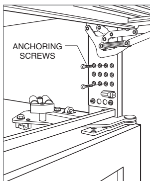
Top anchoring.
