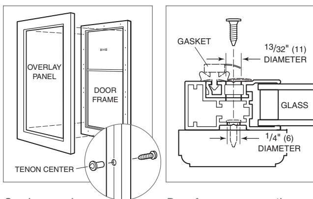
Overlay panel.
