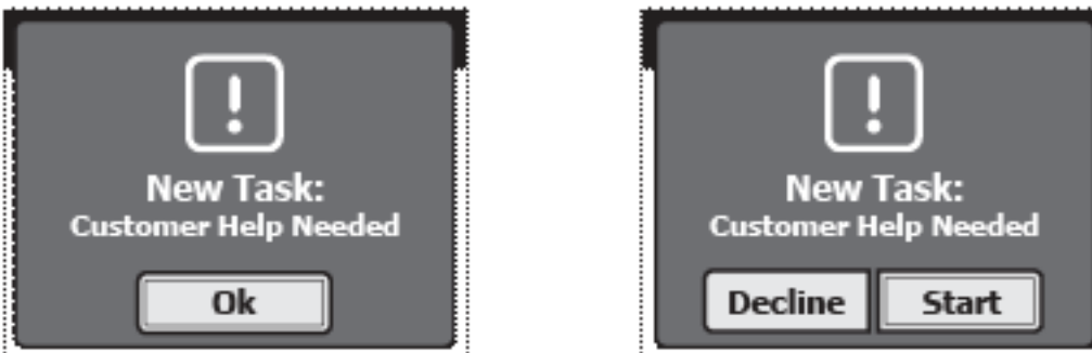
Figure 3-4 Notification Options
