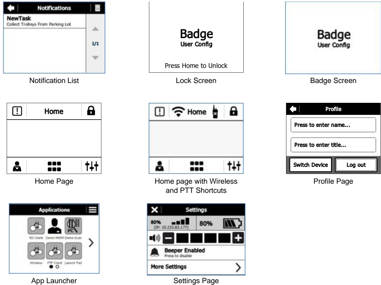
Figure 1-3 System Applications
