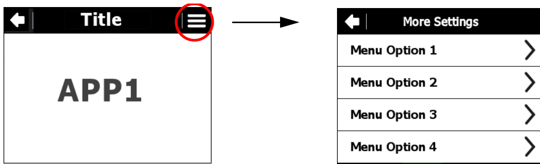
Figure 3-13 Options Menu
