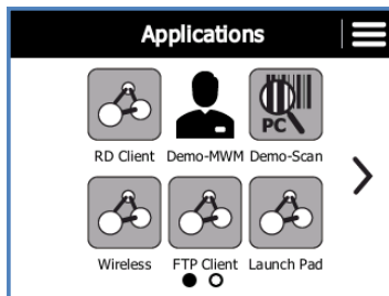
Figure 2-1 Applications Screen
