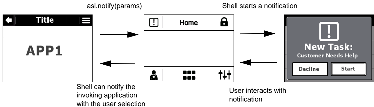
Figure 3-3 Notifications
