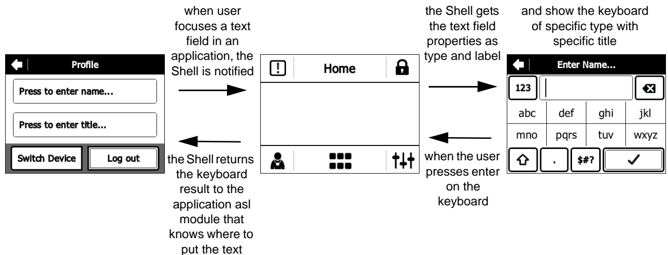
Figure 3-5 Keyboards
