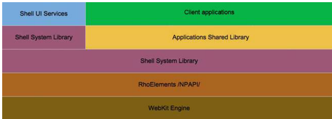
Figure 1-4 Structure Diagram
