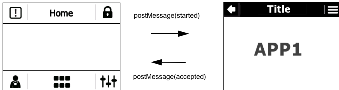
Figure 3-18 Message Handshake
