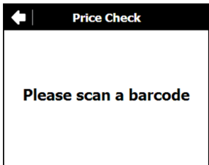
Figure 3-14 Without Options
