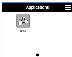
Figure 1-6 Applauncher
