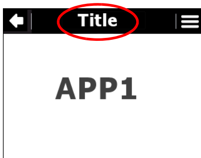
Figure 3-12 Title Label
