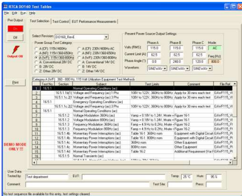
Figure 2-1: 160 Option Test Selection Screen.
