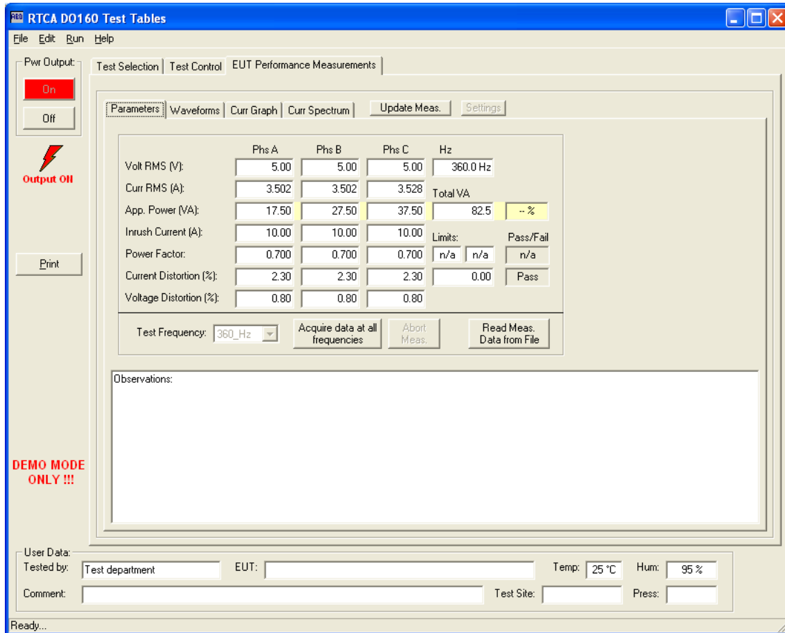
Figure 2-3: 160 Option EUT Measurement Data Screen.
