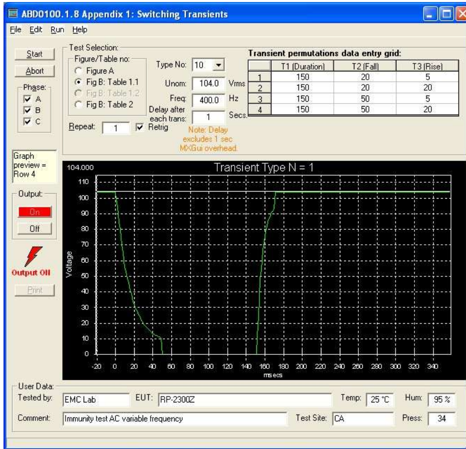
Figure 7-1: ABD0100.1.8 Switching Transient Control Window
