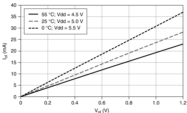
Figure 7. DIO (PFI <0..15>/P1/P2): I_{OI} versus V_{OI}
