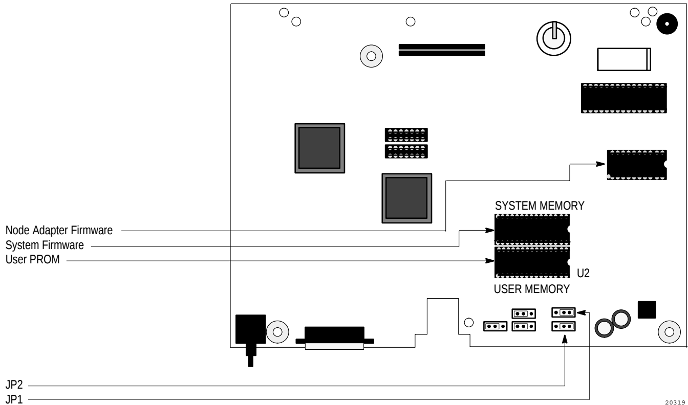
Figure 2 PanelView Series D or E Logic Board, with Jumpers JP1 and JP2 in the EPROM/EEPROM Position
