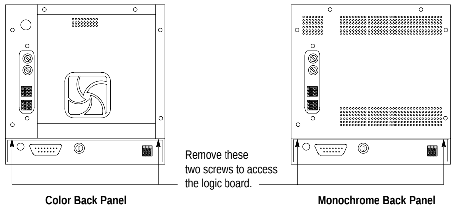
Figure 1 Opening the Series D or E PanelView Terminal
