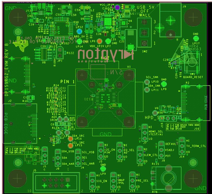
Figure 16. Layer 5 (GND)
