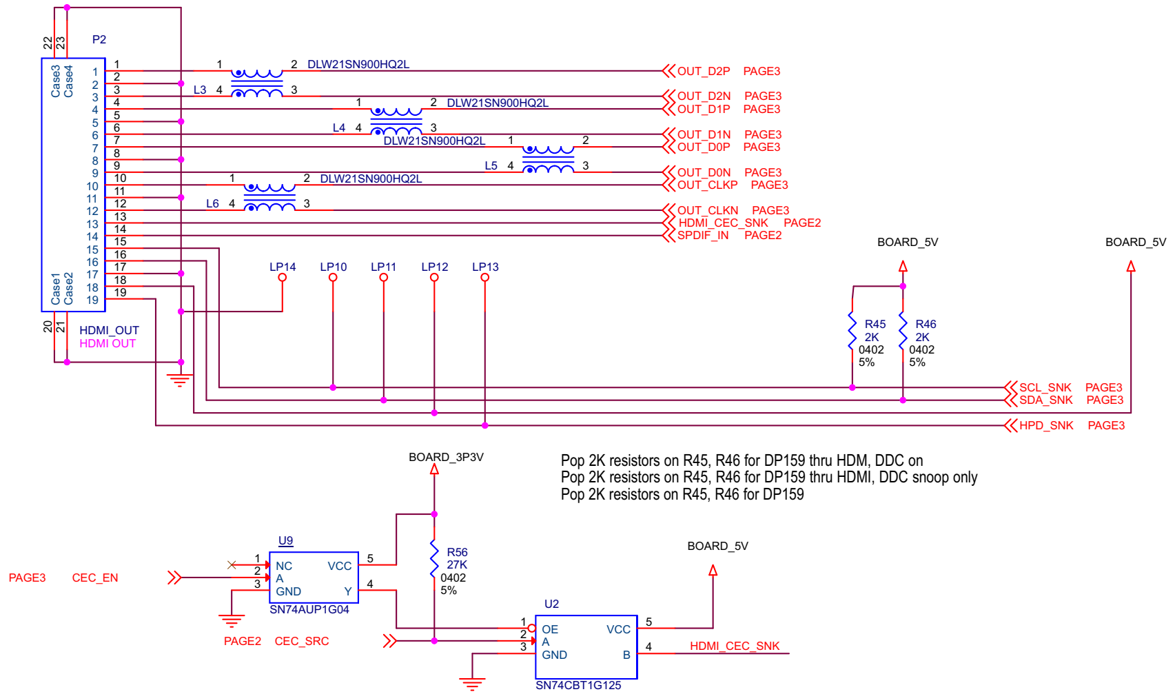
Figure 7. HDMI TX Connector
