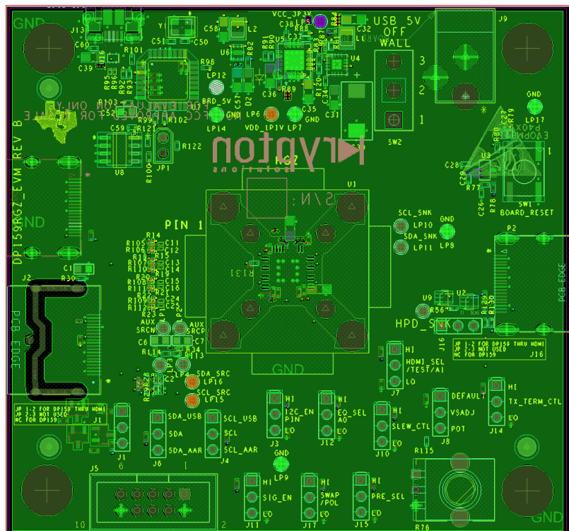
Figure 13. Layer 2 (GND)
