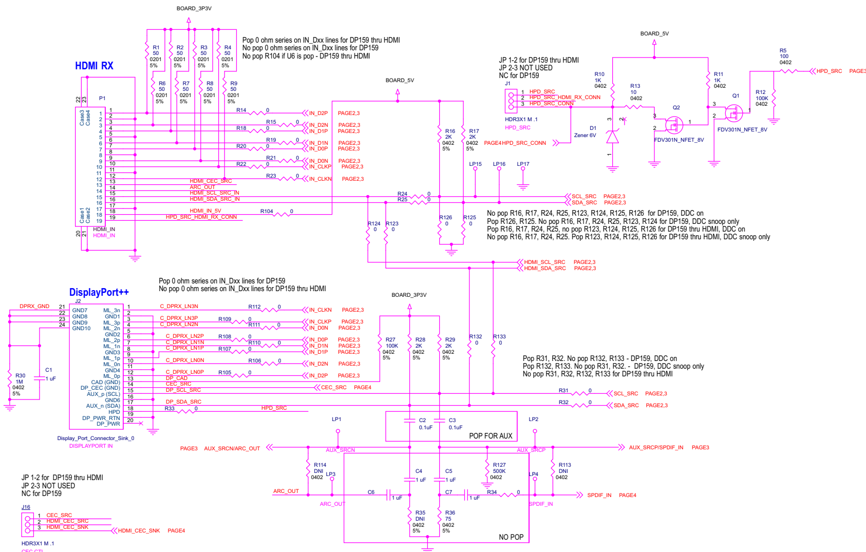
Figure 5. HDMI Input Connectors
