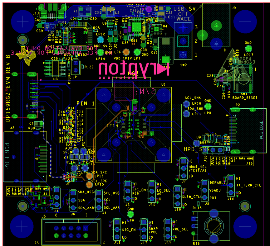
Figure 17. Layer 6 (Bottom)
