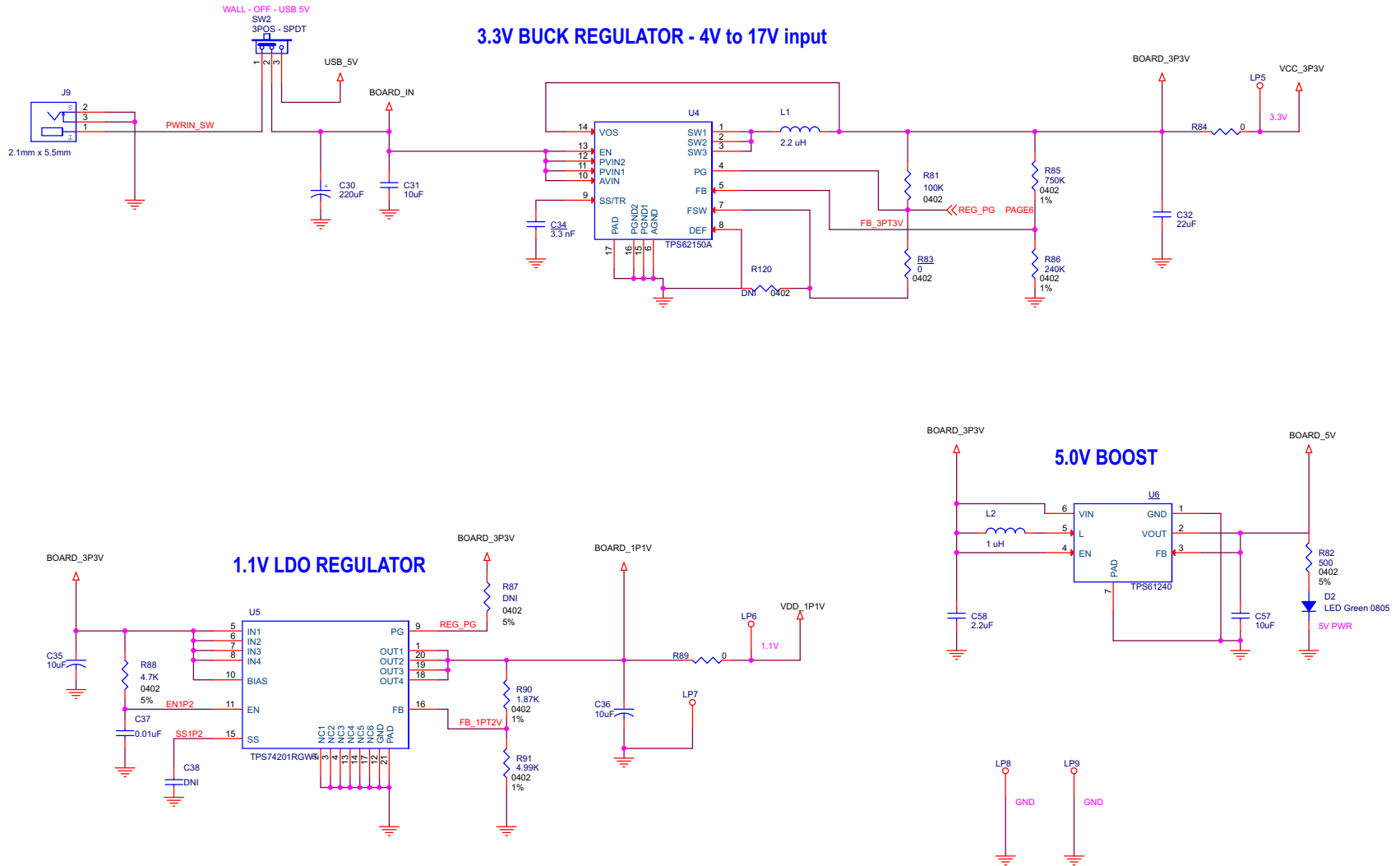
Figure 10. 1.1- and 3.3-V Regulators
