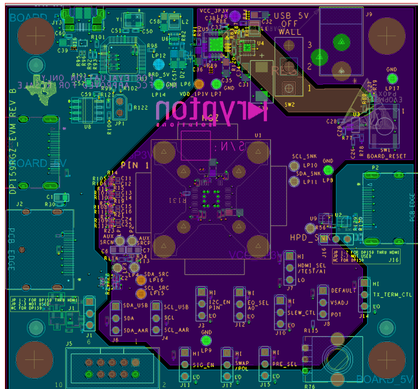
Figure 15. Layer 4 (Power)
