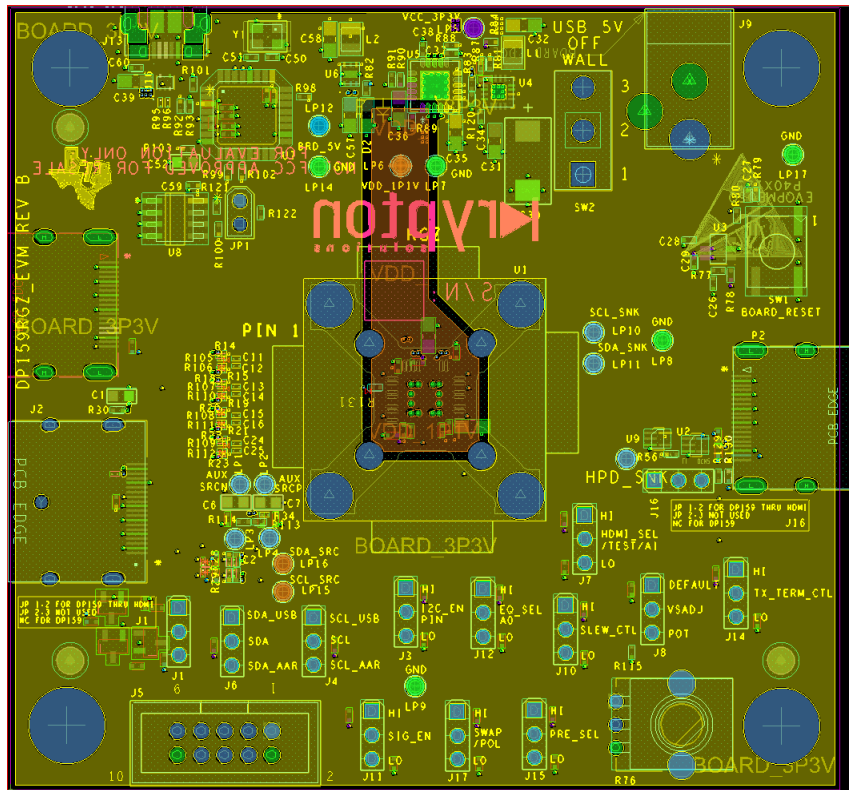
Figure 14. Layer 3 (Power)
