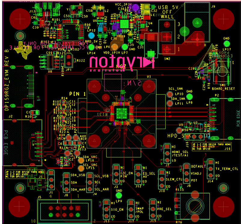
Figure 12. Layer 1 (Top)
