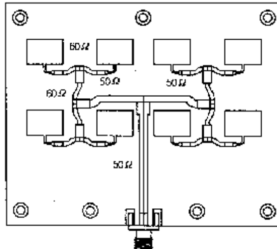
Figure 11-1 Microstrip Patch Array
