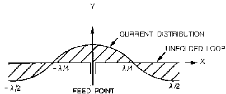
Figure 5-2 Current Distribution of Loop Antenna of Length 1\lambda
