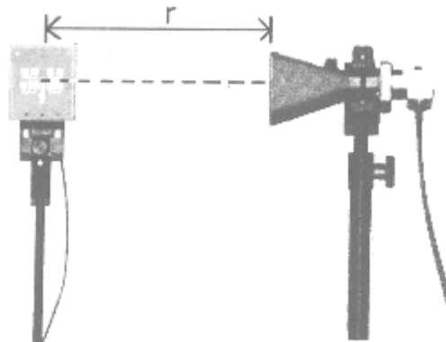
Figure 11-4 Distance between Antennas r
