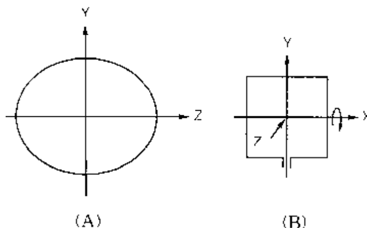
Figure 5-6(A) H-Plane Radial Pattern of Full-Wave Loop Antenna
