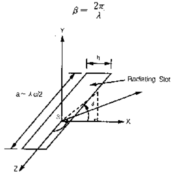
Figure 10-5 Type for Calculation of E -, H - Plane Radial Pattern
