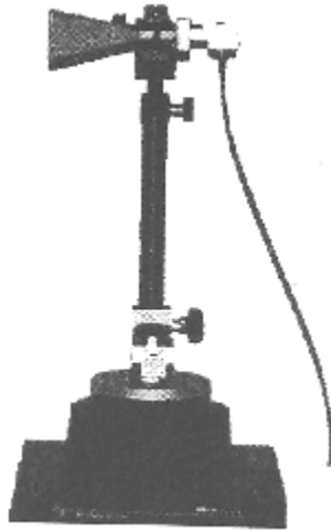
FIGURE 12-9 Horizontal Polarization Transmitting Antenna
