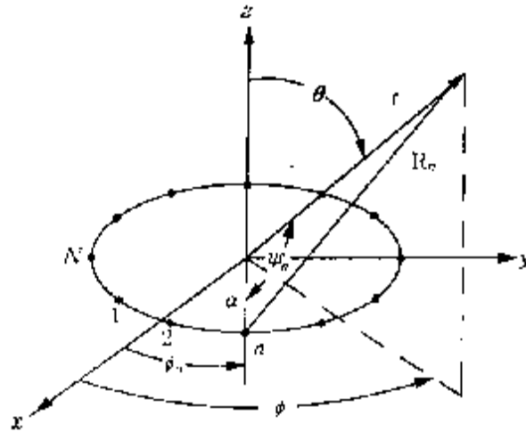
FIGURE 12-3 N-Circle Arranging Structure
