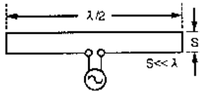
Figure 2-1 \lambda/2 Folded Dipole
