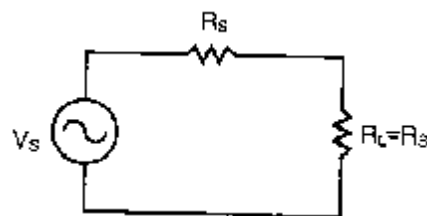
Figure 2-5 Impedance Matching between a power and load for the maximum power transmitting
