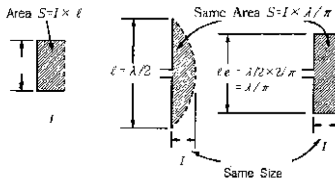
(A) Infinitesimal Antenna (B) \lambda/2 Dipole (C) \lambda/2 Dipole Effective Wave
