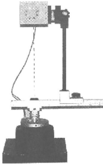
Figure 12-12 Installation of circle arranging antenna
