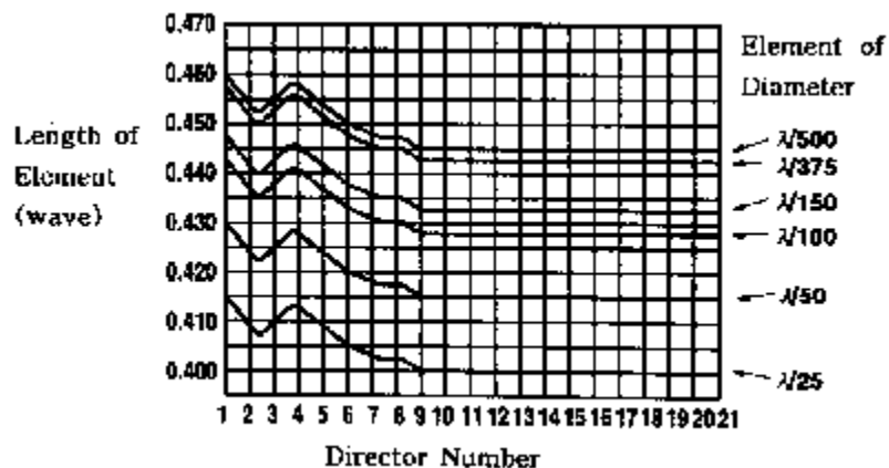
Figure 6-5 Method taking each Director
