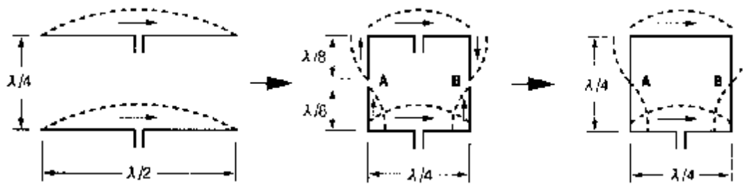
(A) \lambda/4 Spacing Step Dipole (B) \lambda/8 Fold and Bend of Both Side (C) 1 Wave Loop
