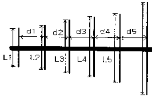
Figure 6-10 Yagi Antenna
