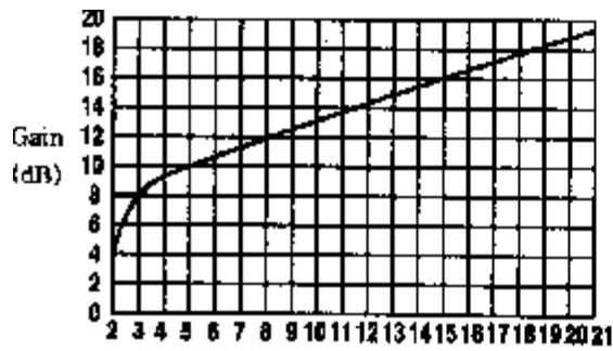
Element Number Figure 6-3 Relation between Element Number and Gain.
