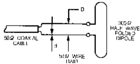
Figure 2-8 Folded Dipole Without Balun
