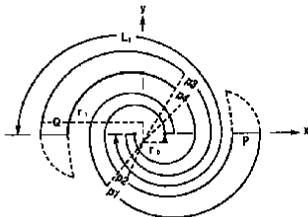
Figure 7-1 2Arm Equiangular Spiral Antenna
