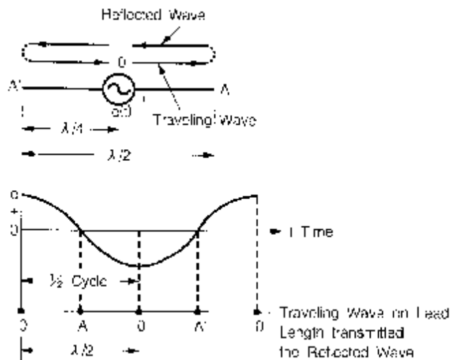
Figure 1-2 The reason that the electric wave of wave 3 resonate to lead \lambda/2
