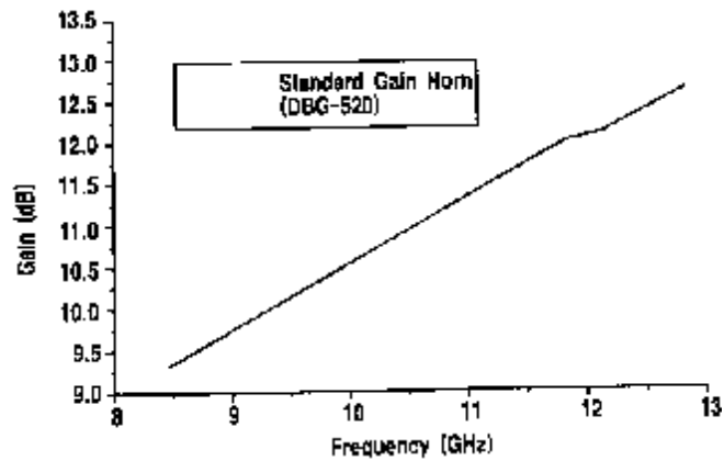
FIGURE 12-7 Standard Gain Horn Antenna (DGB-520)
