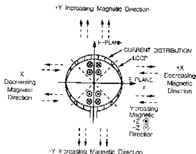
Figure 5-3 Current Distribution of Circle Loop Antenna
