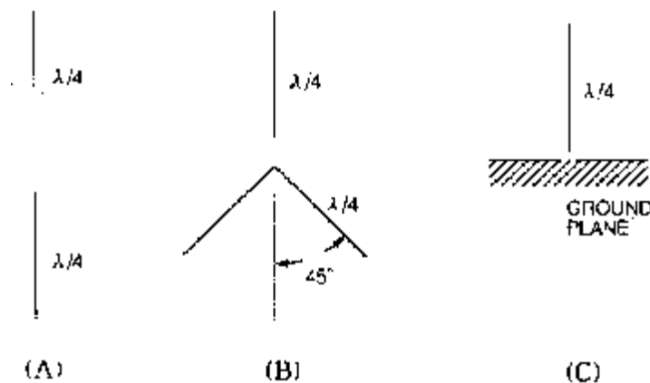
Figure 4-9 (A) Half Wave Dipole (B) Drooping Antenna (C) \lambda/4 Ground Antenna
