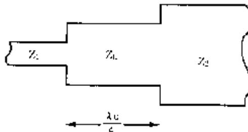
Figure 10-7 \lambda/4 of Impedance Z_L for matching impedance Z_1 , Z_2
