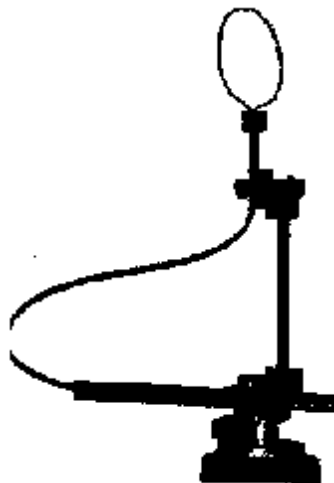
Figure 5-12 Setting of Even Polarization Receiving Antenna
