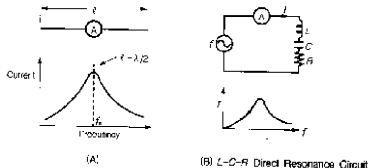
Figure 1-1 Antenna and Resonance Circuit
