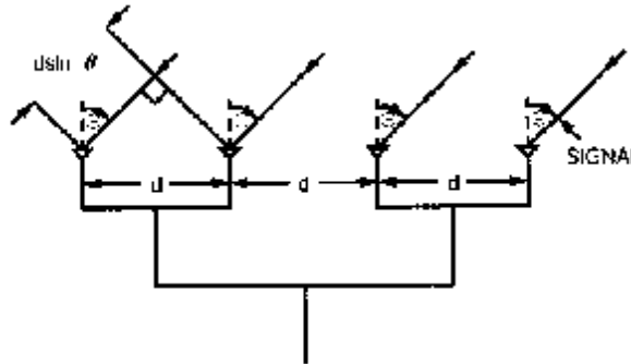
Figure 12-1 4-Element Linear Array
