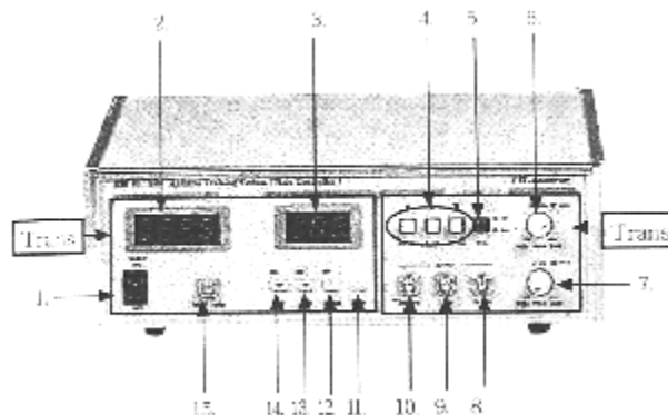
Figure 1-2 Main Controller
