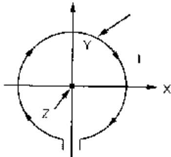
Figure 5-1 Current in Infinitesimal Loop Antenna
