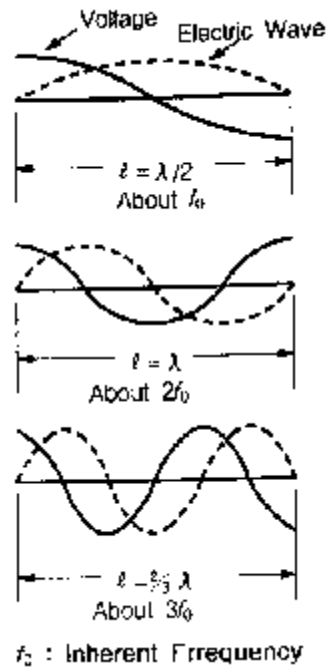
Figure 1-4 High Frequency Excitations of Harmonics
