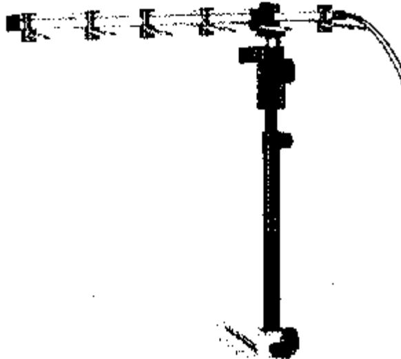
Figure 7-3 Even Polarization Transmitting Antenna
