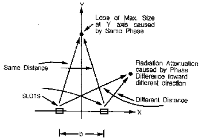
Figure 10-4 Analysis of E-Plane Far-Field in Square Patch
