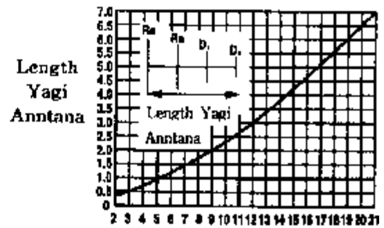
Yagi Element Number Figure 6-4 Relation between Length of Antenna and Element Number
