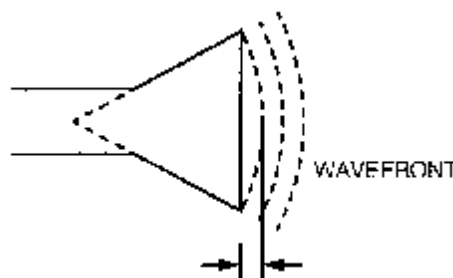
Figure 9-2 Phase Error by Wave Front of Horn Antenna (A)
