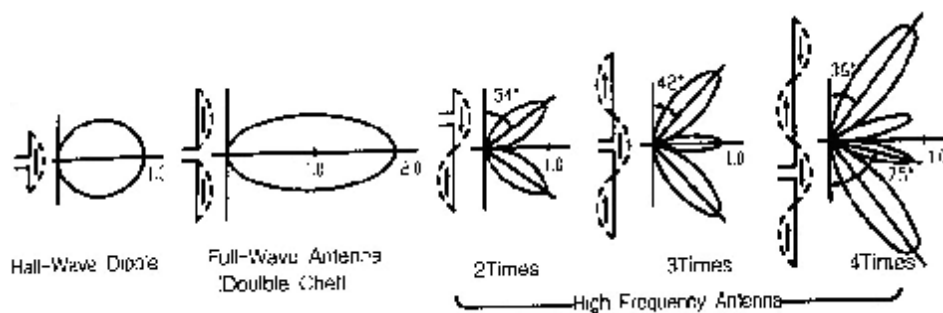
Figure 1-10 Directivity of Half-Wave, Full-Wave and Harmonics
