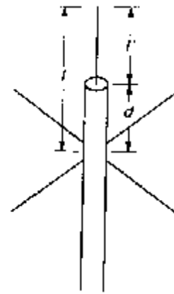
Figure 4-7 Place the Vertical Radial in a Coax
