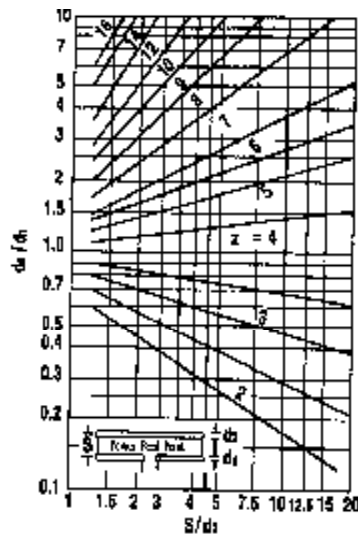
Figure 2-3 Impedance Change of 2Line Type Folded Dipole
