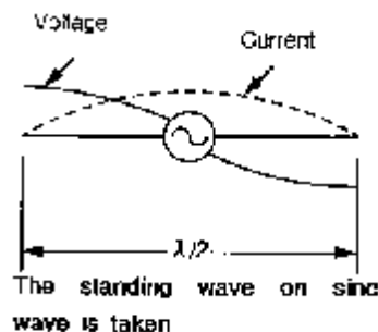
Figure 1-3 Voltage Current Distribution on both end open \lambda/2 lead
