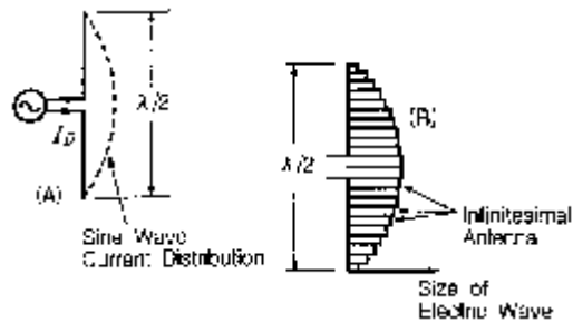
Figure 1-7 (A) Center Feed Half Wave Doublet
