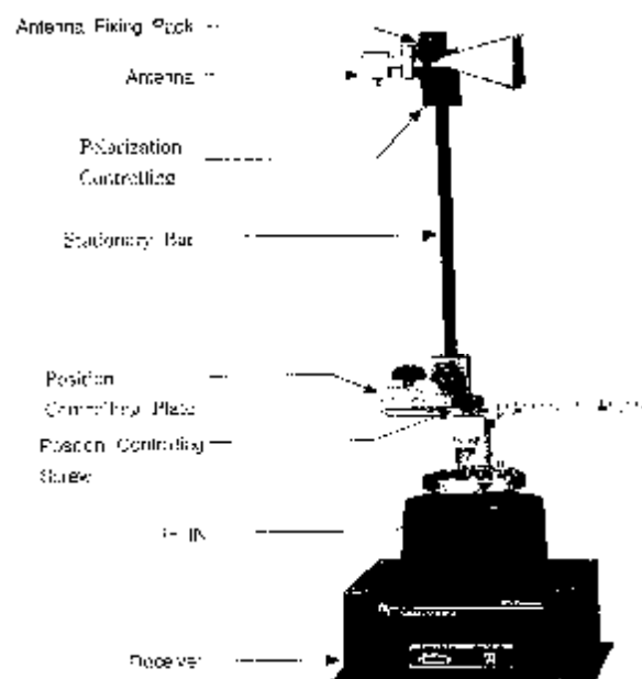
Figure 1-4 Receiver
