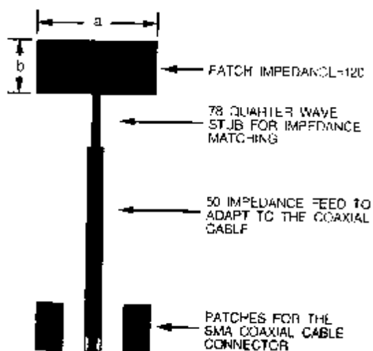
Figure 10-8 Single Patch Antenna (Unit: mm)
