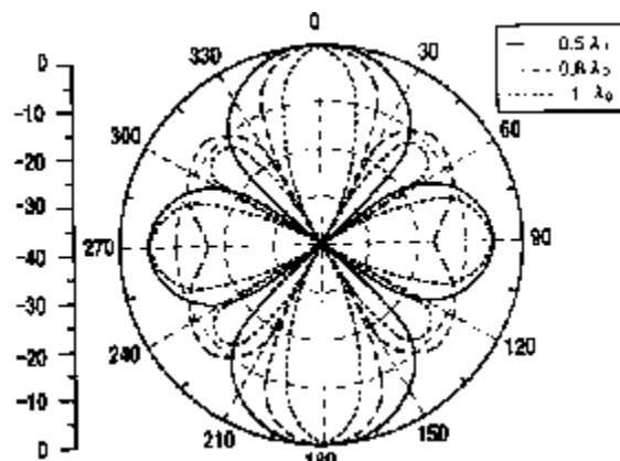
FIGURE 12-4 Radiation Pattern Change of Circle Arranging Antenna According to the Isolated Distance Change (Y-z plane)
