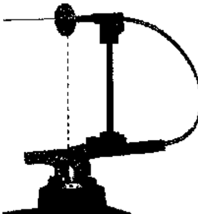
Figure 3-9 Setting of Even Polarization Receiving Antenna
