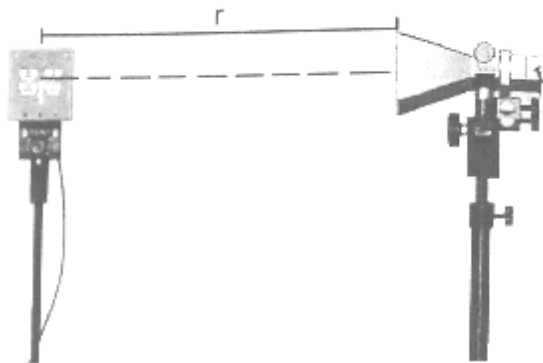
Figure 11-6 Vertical and Horn Antenna
