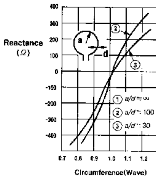
Figure 5-10 Input Impedance of 1 Wave Circle Loop
