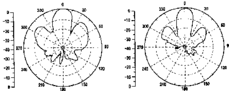
FIGURE 12-8 Radiation Pattern of Circle Arranging Antenna(8-element)
