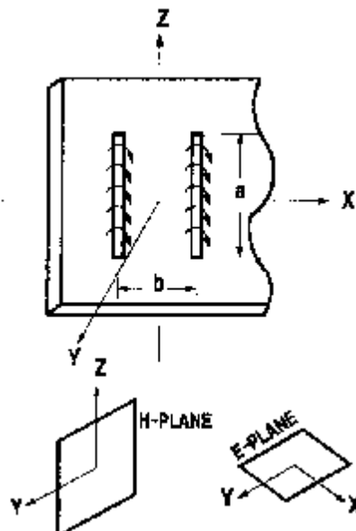
Figure 10-3 Two Parallel Slot in Waveguide
