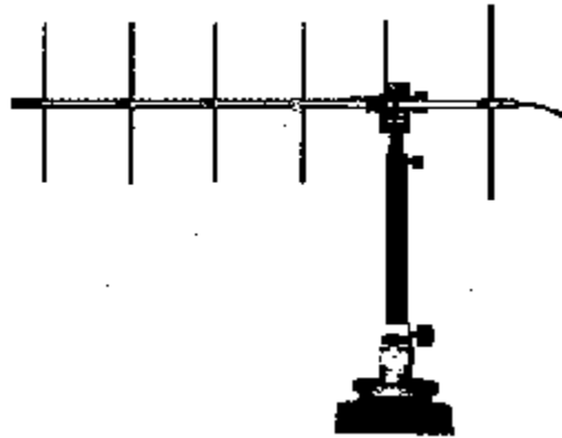
Figure 6-12 Setting of Vertical Polarization Transmitting Antenna
