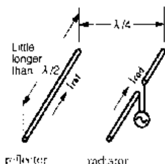
(A) 2 Element Yagi
