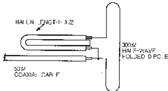
Figure 2-9 Folded Dipole with Balun
