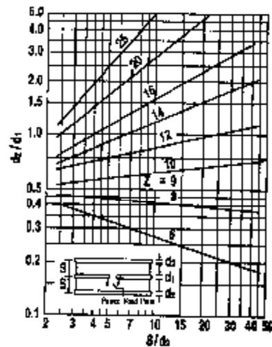
Figure 2-4 Impedance Change of 3Line Type Folded Dipole
