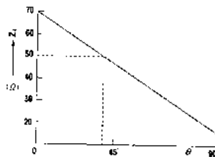
Figure 4-5 Angle \theta and Impedance of Vertical Element
