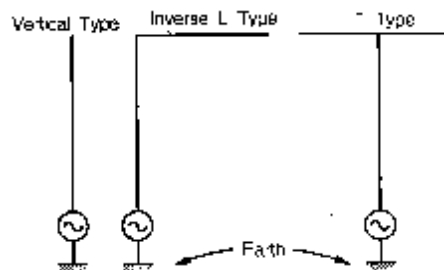
Figure 3-1 Representative Ground Antenna
