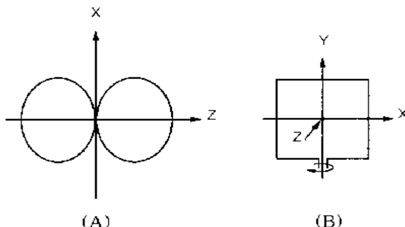
Figure 5-5 (A) E-Plane Radial Pattern of Full-Wave Loop Antenna
