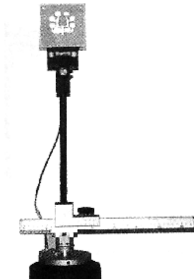
Figure 12-10 Installation of Horizontal Polarization Receiving Antenna
