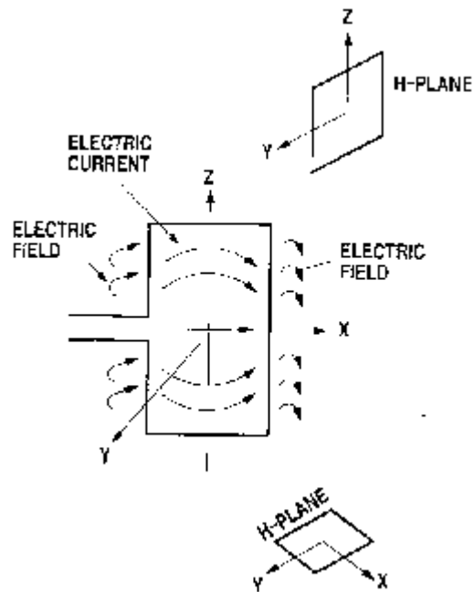
Figure 10-2 Current Distribution and Main Type of Field
