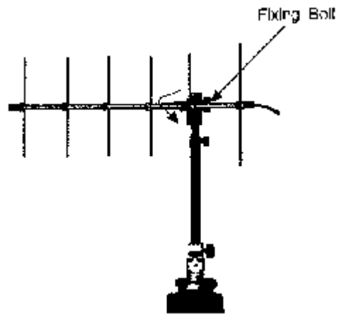
Figure 1-15 Setting of a Even Polarization Transmitting Antenna
