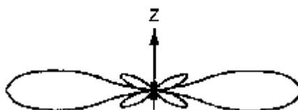
Figure 8-3 Radial Pattern of Pencil Beam
