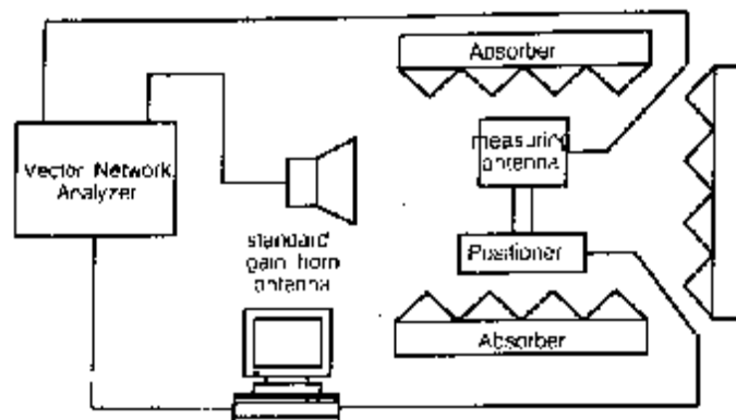
FIGURE 12-6 Antenna Measuring System
