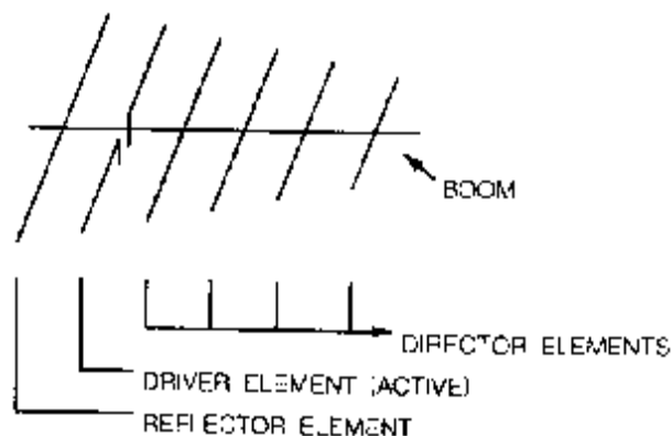
Figure 6-6 6 Antenna Element Yagi Antenna
