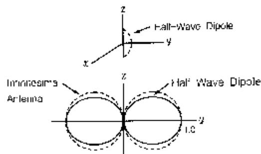
Figure 1-8 Field Directivity of Half-Wave Dipole(side y \wedge z )
