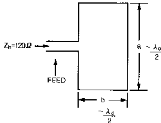
Figure 10-1 Basic Square Microstrip Antenna
