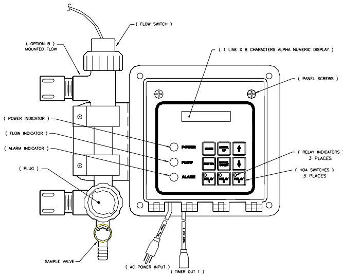
FIGURE 15 MCT110 Front Panel
