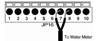
FIGURE 10 Art for water meter connection
