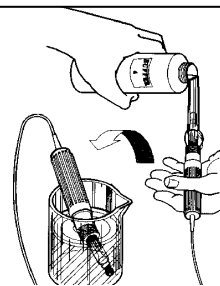
FIGURE 24 Adding pH buffer solution to probe in a clean container for calibration.
