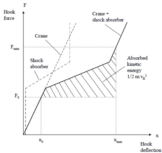
Figure A.1 - Effect of shock absorbers
