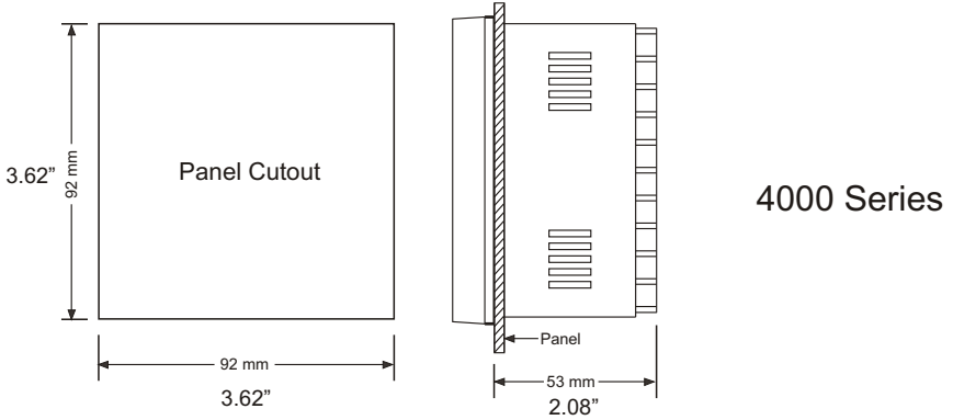
Figure 2.1 Mounting Dimensions
