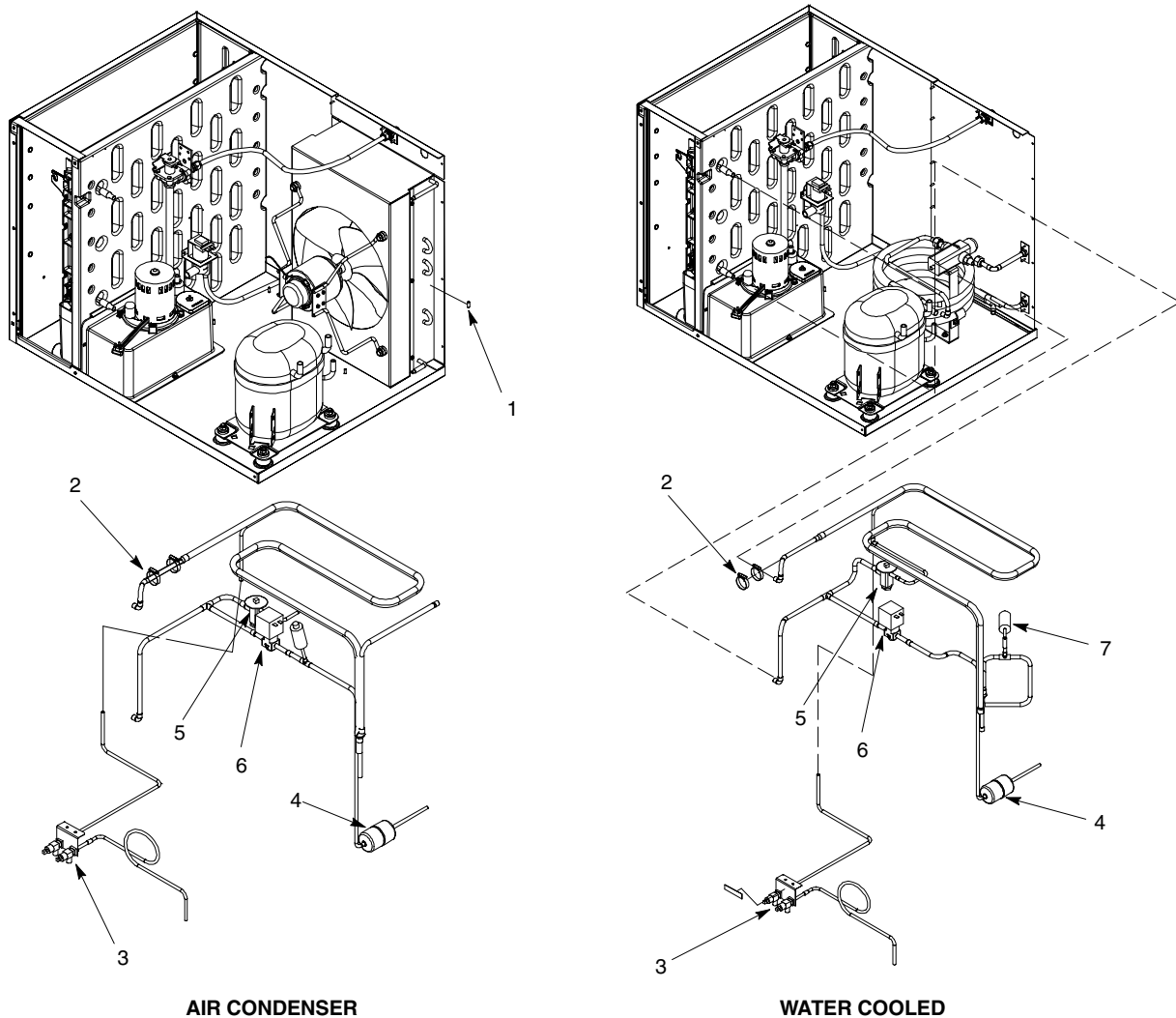
FIGURE 3. REFRIGERATION ASSEMBLY
