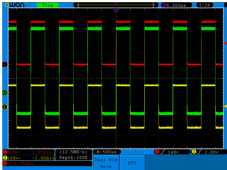
Fig. 5-7 Waveform resulted from CH1 +CH2 Mathematical Manipulation User Manual of Smart Digital Storage Oscilloscope
