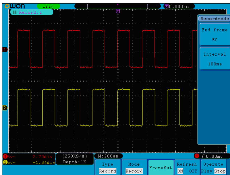
Fig.5-36 Wave Record
