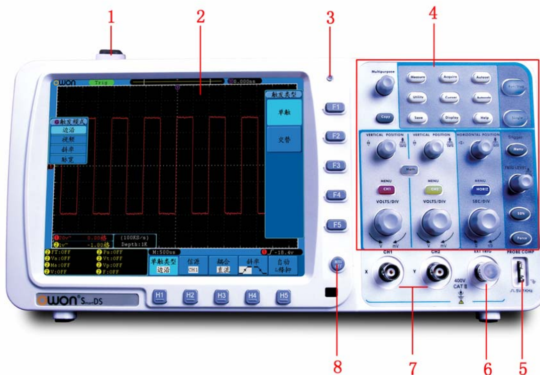
Fig. 4-1 Front panel
