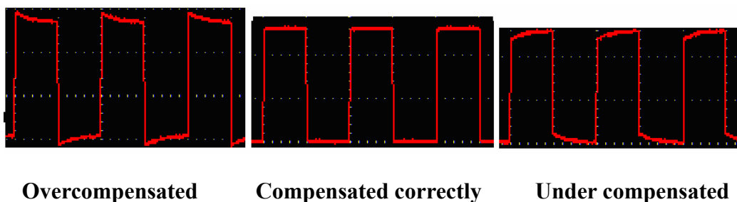
Fig. 4-8 Displayed Waveforms of the Probe Compensation
