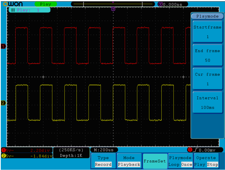
Fig. 5-37 Wave Playback
