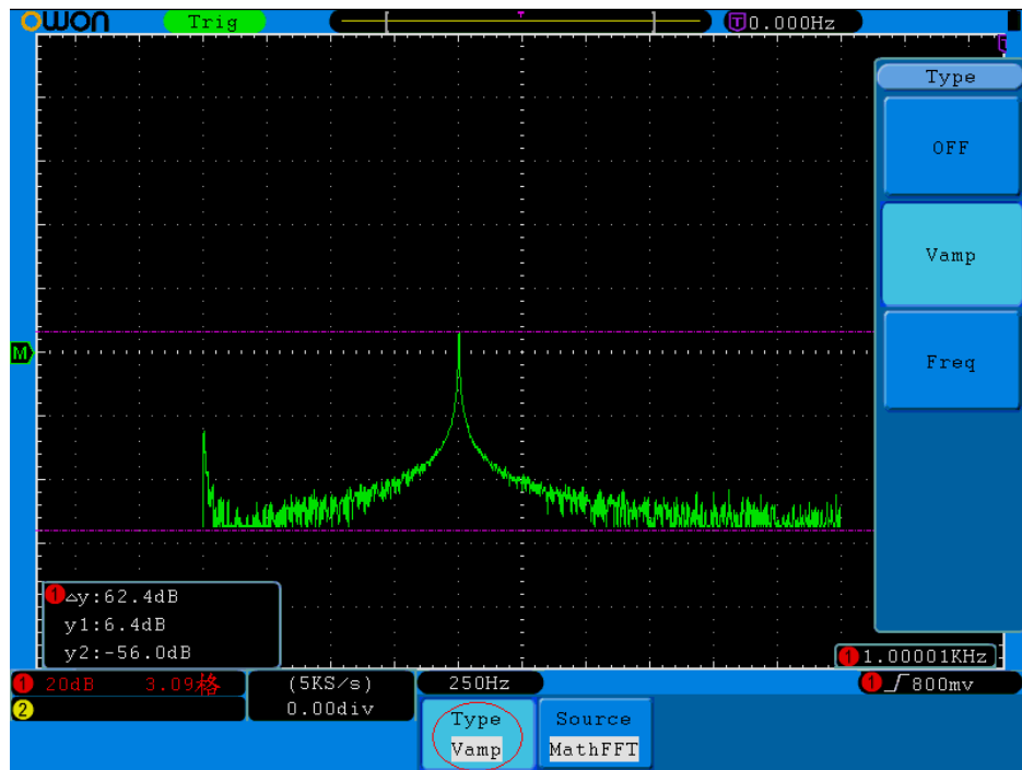
Fig.5-54 wave of Vamp cursor measurement
