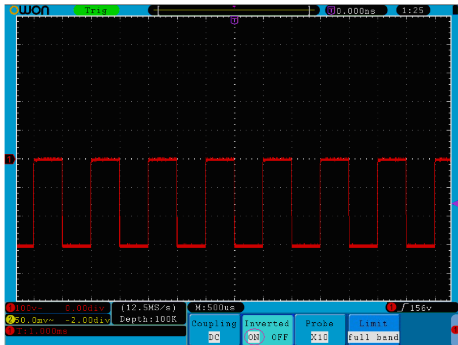
Fig. 5-5 Waveform Inverted
