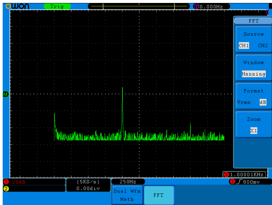
Fig.5-11 Hanning window
