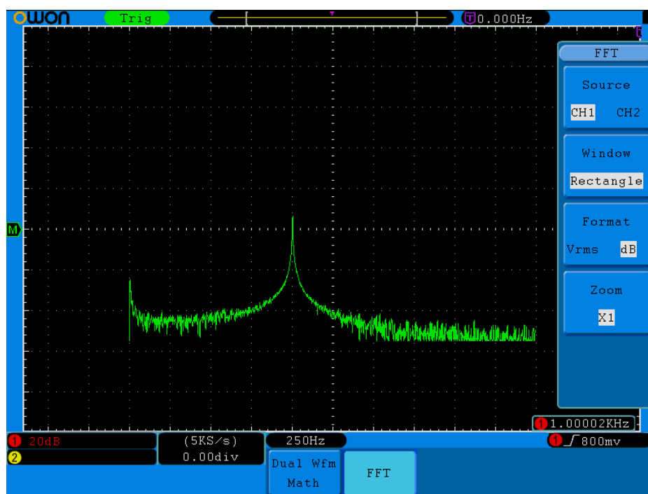
Fig.5-10. Rectangle window
