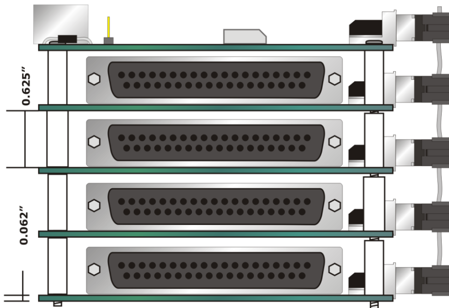
Figure 9-13: USB-AIOxx-128A Mechanical Drawing
