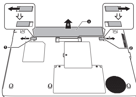
Figure 4-10 Releasing the battery pack (R940)
