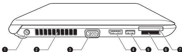
Figure 3-2 The left side of the computer (R950)
