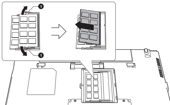
Figure 4-14 Removing the memory module (R940)
