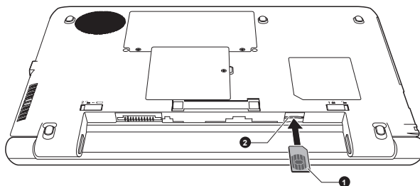
Figure 4-7 Installing the SIM Card (R940)
