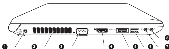
Figure 3-8 The left side of the computer (R940)
