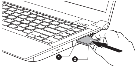
Figure 4-17 Inserting the ExpressCard (R940)
