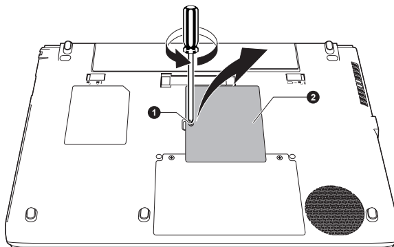
Figure 4-11 Removing the memory module cover (R940)
