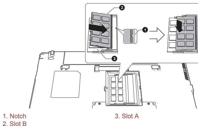
Figure 4-12 Seating the memory module (R940)
