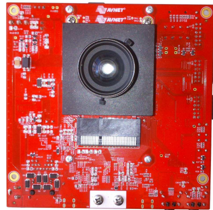
Figure 10: The PYTHON-1300 Camera Module Plugged In the Carrier Card
