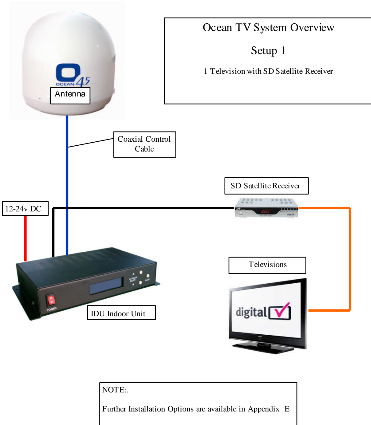
Figure 1 –1 System Diagram
