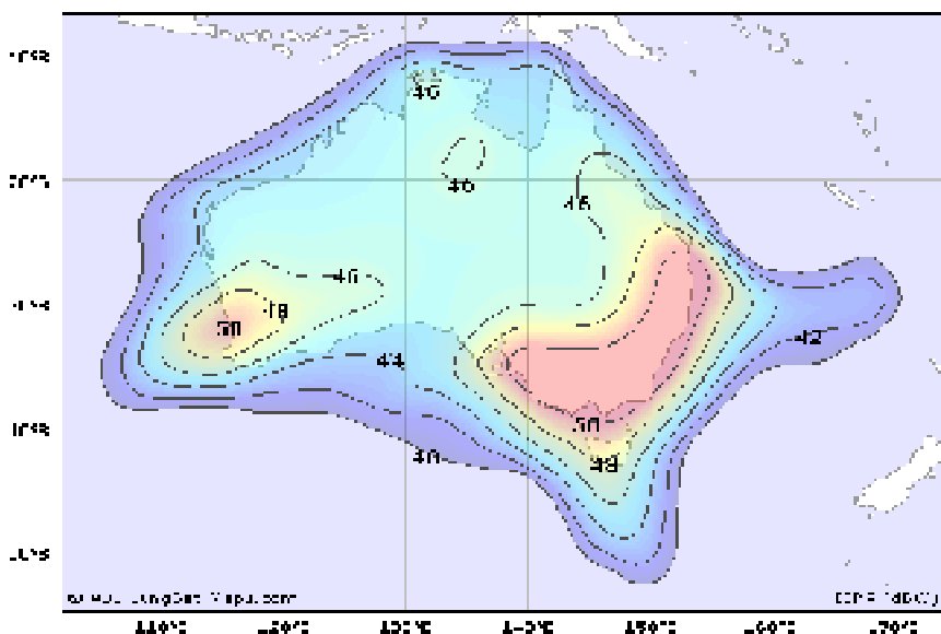
Foxtel - Austar - Aurora - VAST Optus C1 Satellite Coverage Area O37M Requires 50dBW O45M Requires 48-49dBW
