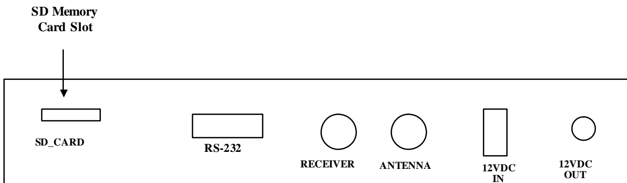
Figure C-3 The back of the IDU
