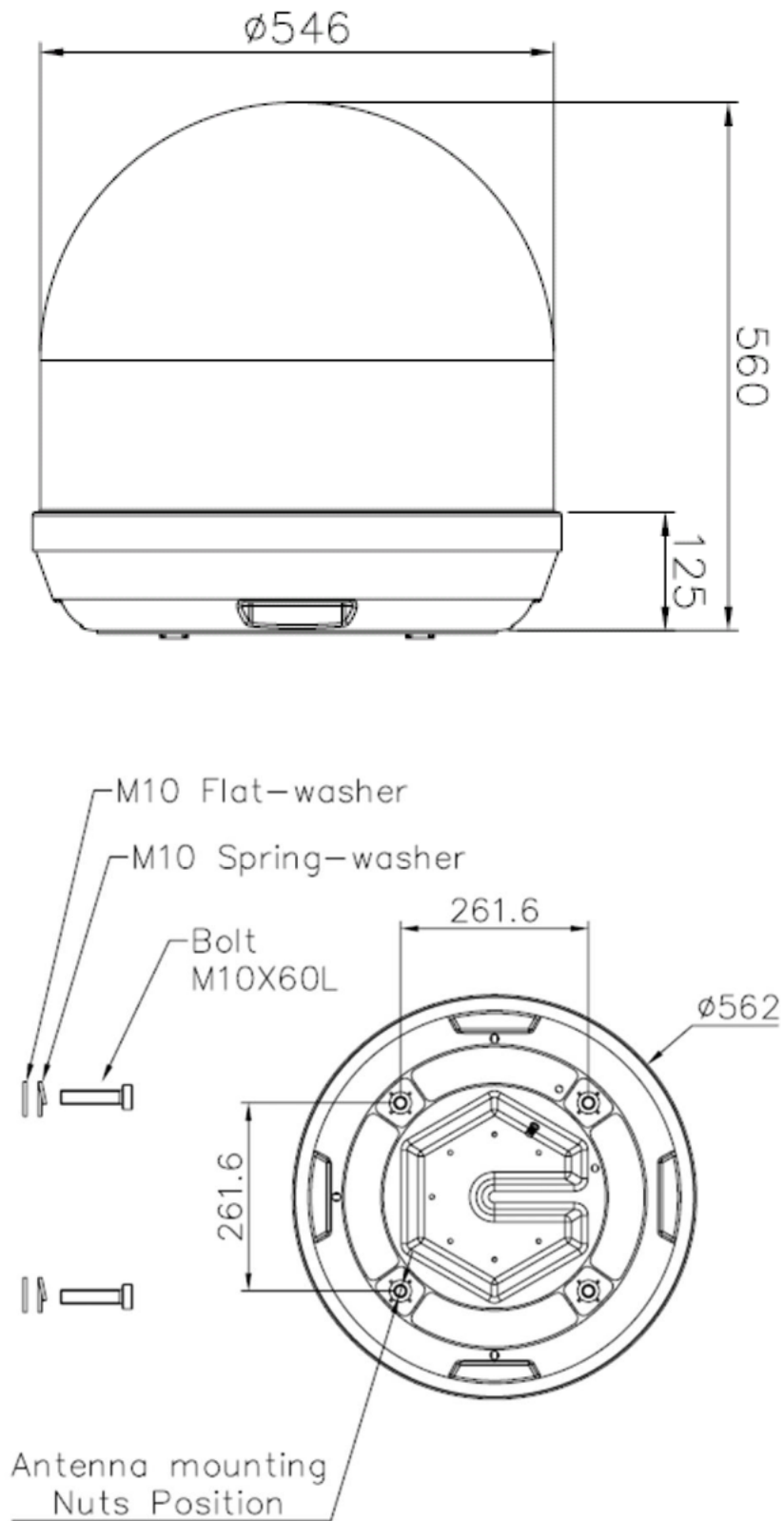
Figure 1-1 O45M Drawing
