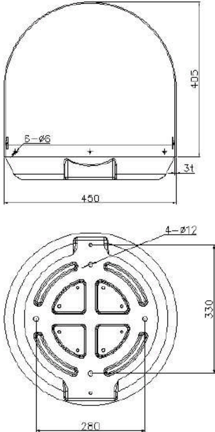
Figure 1-1 O37 Drawing
