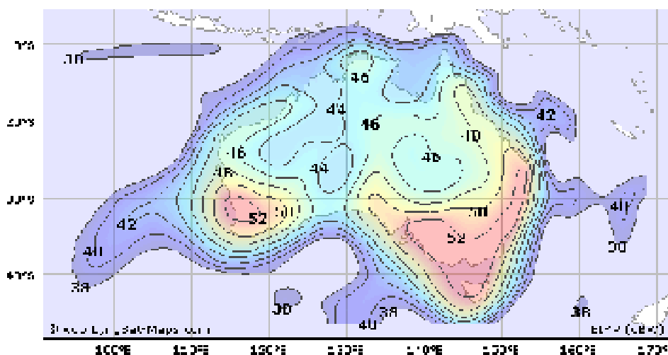
Foxtel - Austar - Aurora Optus D3 Satellite Coverage Area O37M Requires 50dBW O45M Requires 48-49dBW
