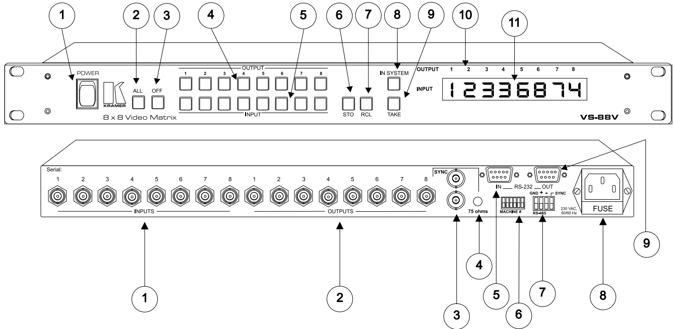
Figure 2: VS-88V Front/Rear Panel Features
