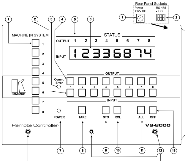
Figure 5: VS-8000 Top/Rear Panel Features
