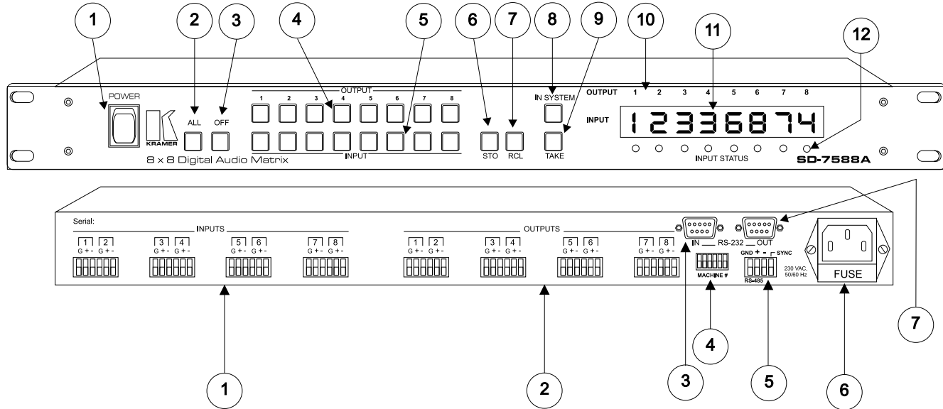
Figure 3: SD-7588A Front/Rear Panel Features
