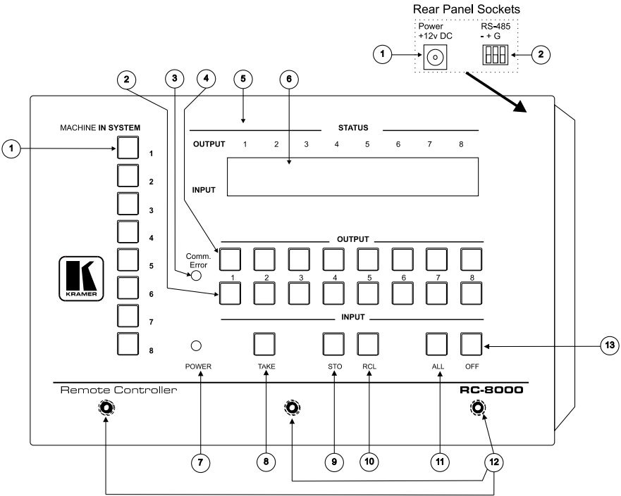
Figure A1: RC-8000 Top/Rear Panel Features
