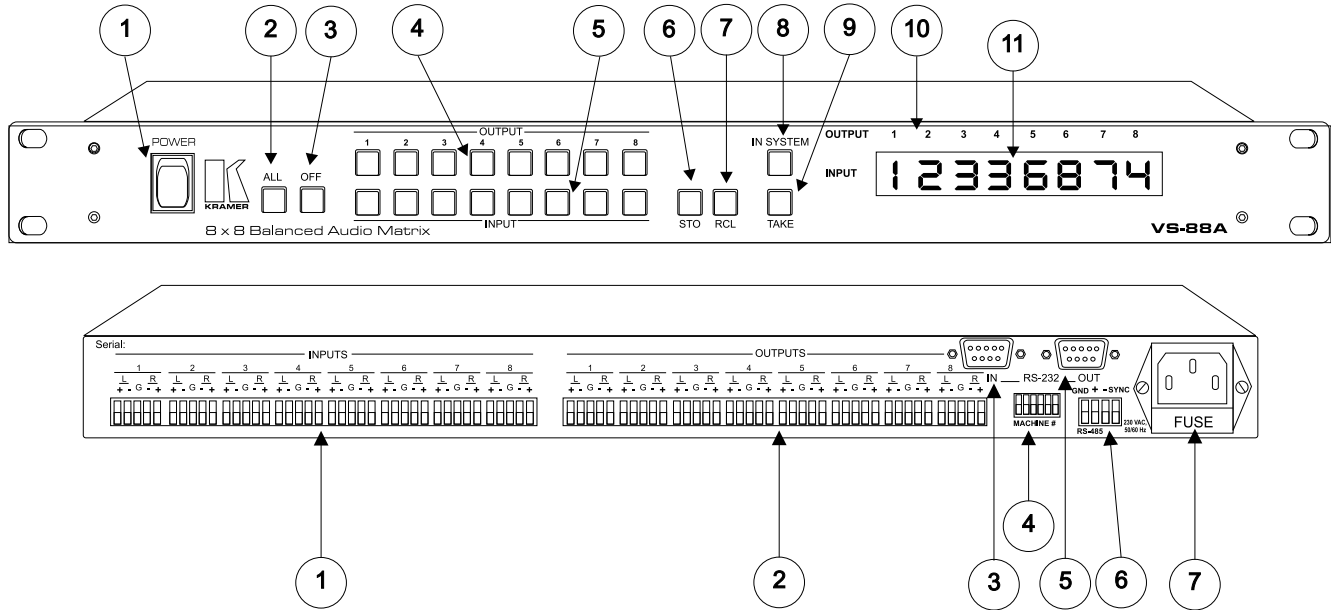
Figure 1: VS-88A Front/Rear Panel Features
