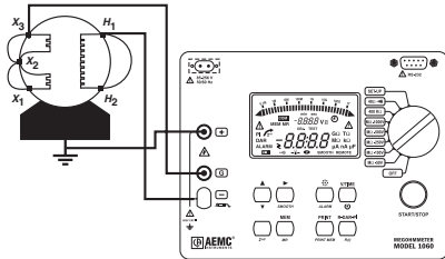
d. High voltage winding to ground
