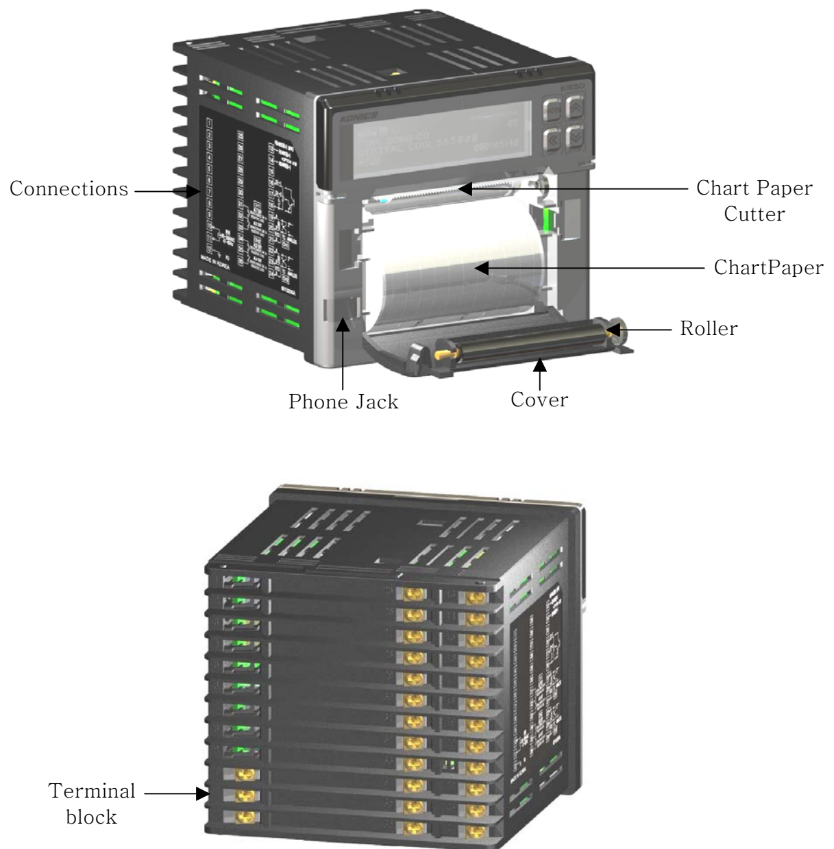
[ Figure 5-1 Each part name ]
