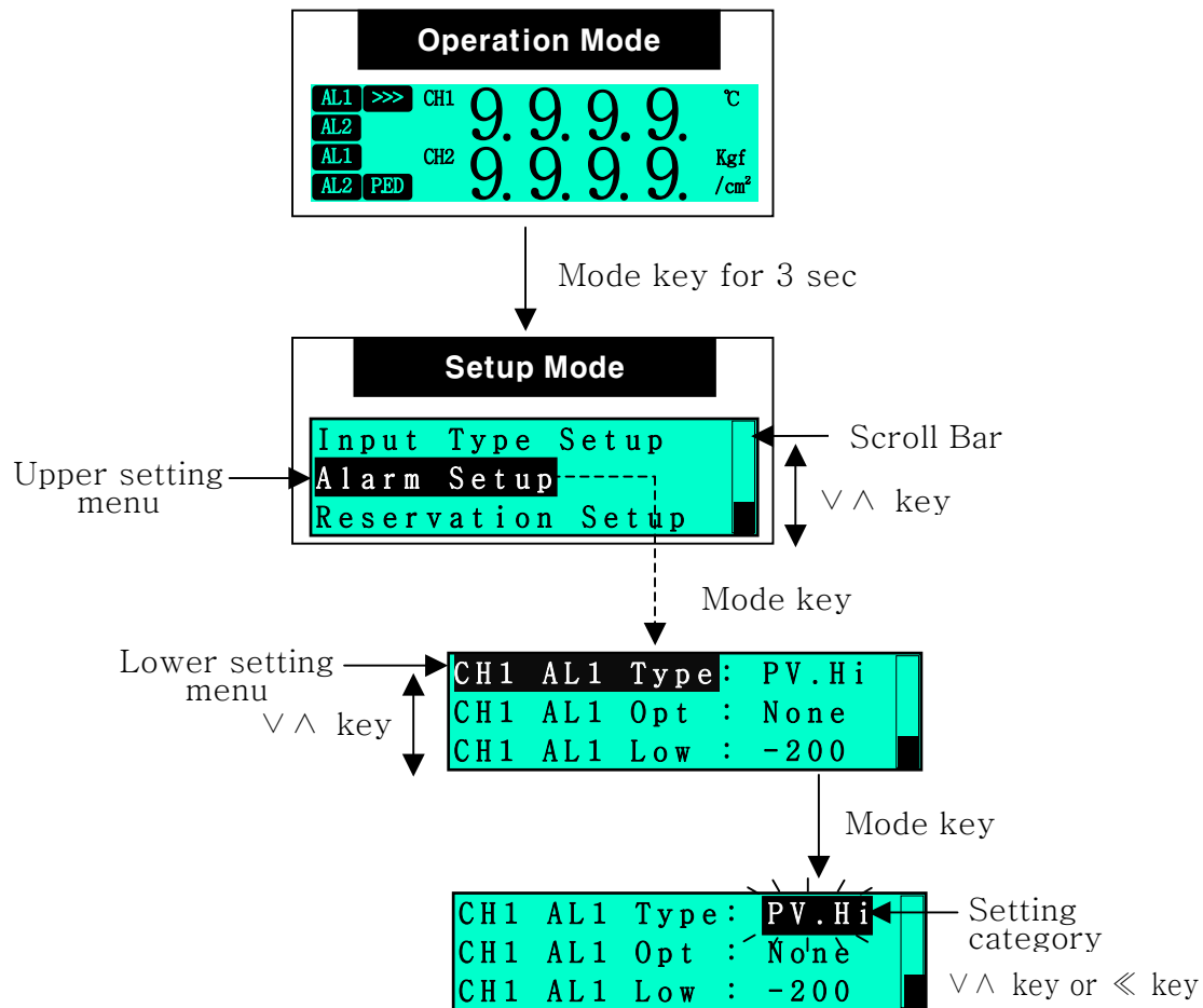
[Figure 7-2 Setting mode entrance display]
