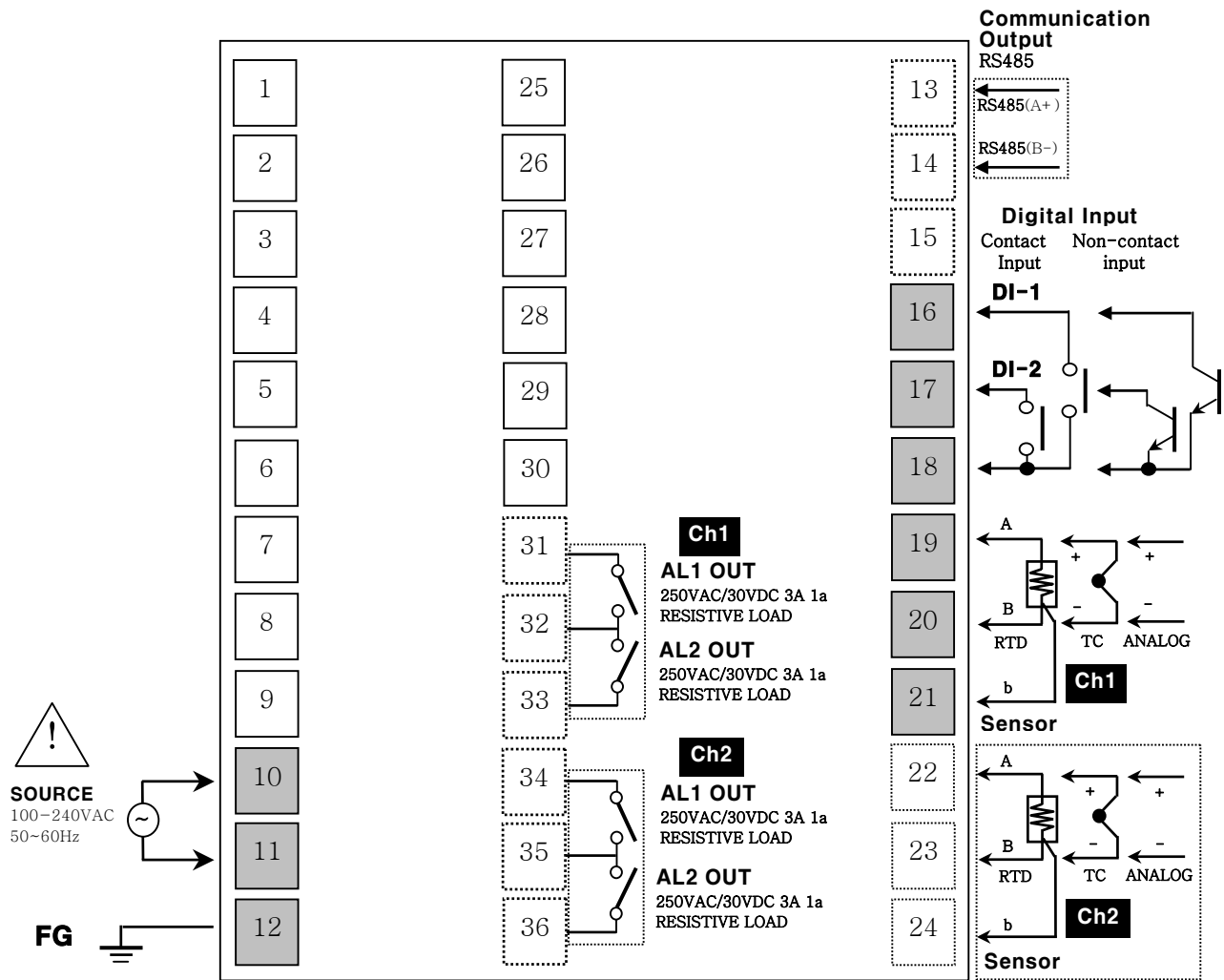
[Figure 6-3 Connections]
