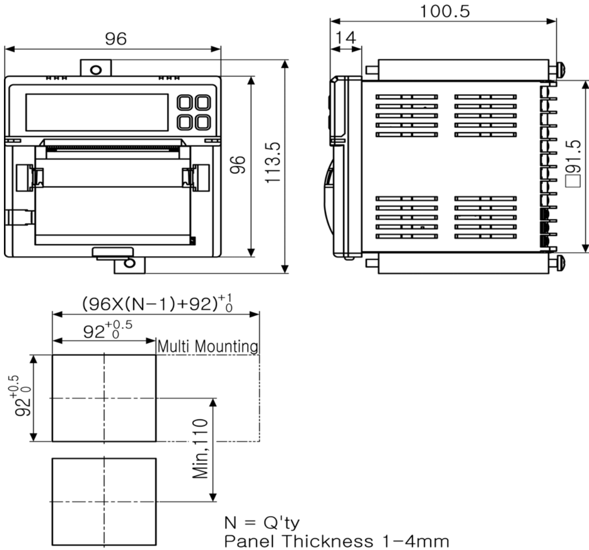
[Figure 6-2 Dimensions and panel cut-out]
