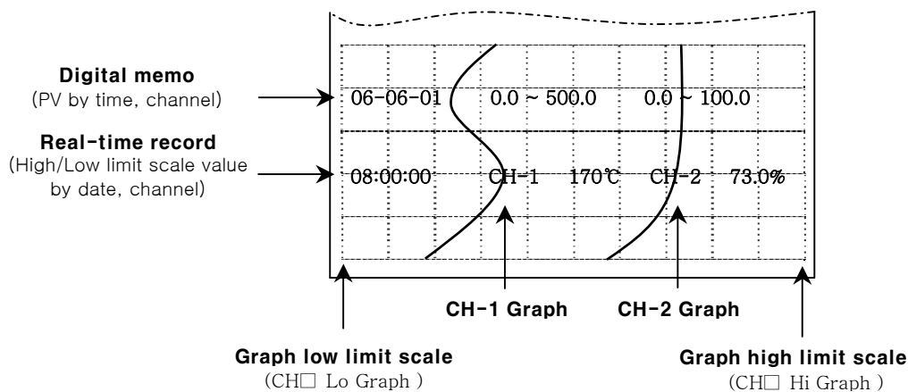
[Figure 11-1 Print on graph mode]
