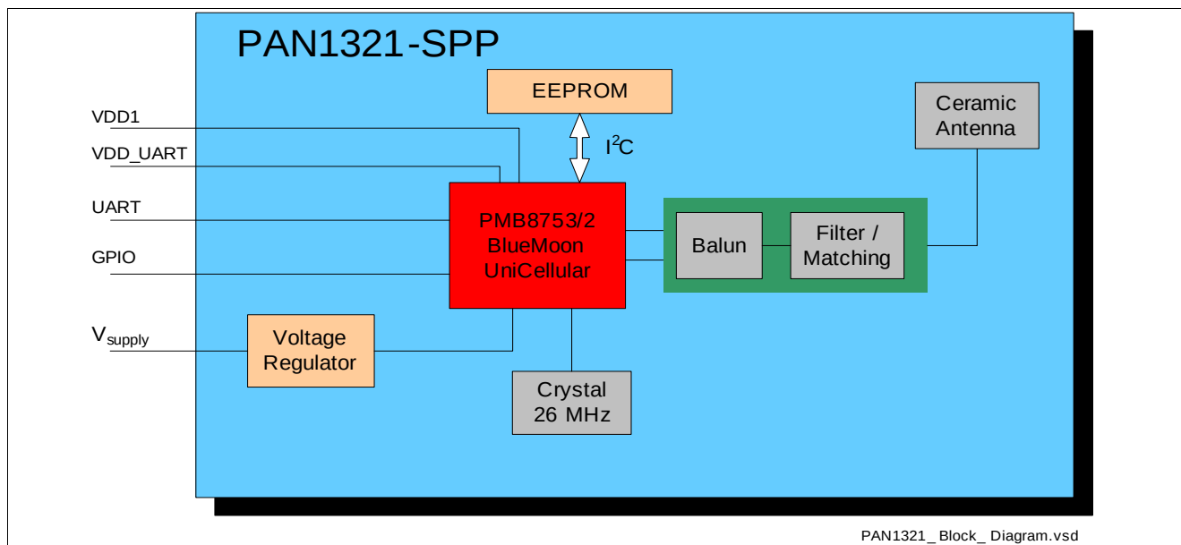
Figure 1 Simplified Block Diagram of PAN1321-SPP
