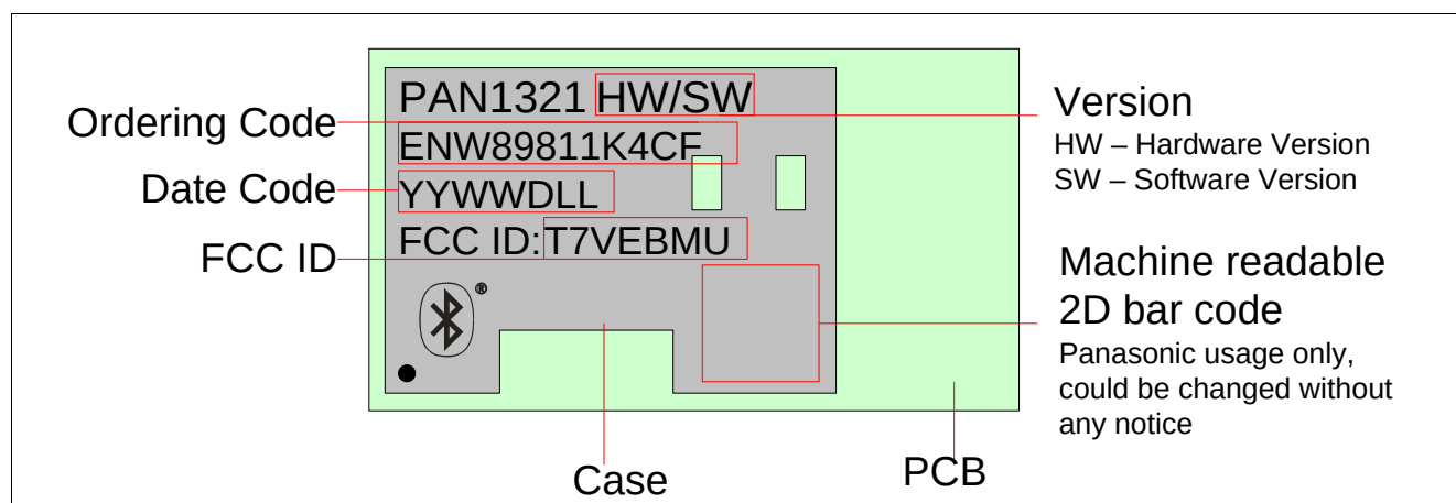
Figure 5 Package Marking
