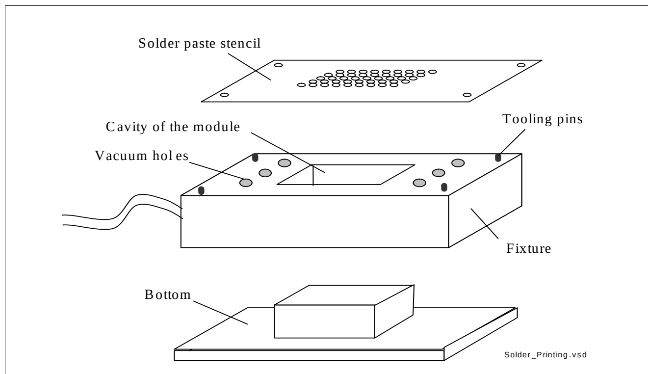
Figure 16 Solder Printing
