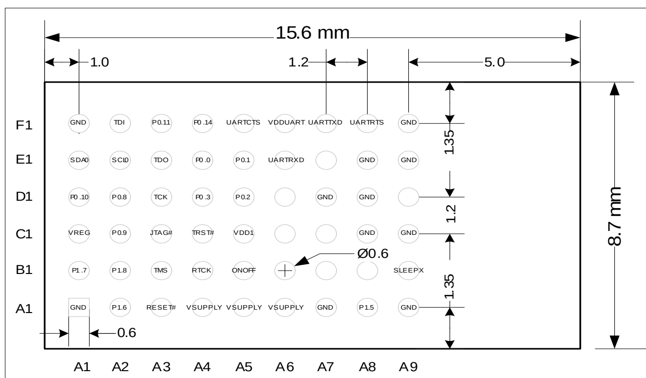
Figure 11 Pad Layout on the Module (top view)
