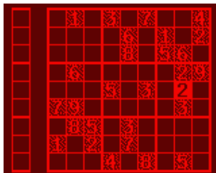
Figure 10.22: Sudoku
