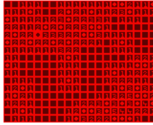
Figure 10.10: Minesweeper plugin
