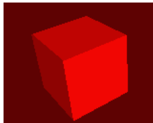
Figure 10.26: Cube
