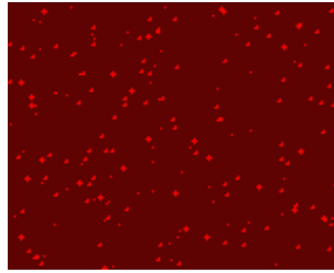
Figure 10.35: Starfield
