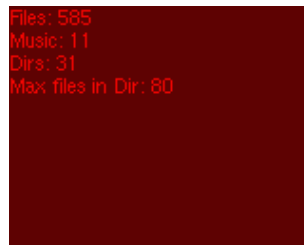
Figure 10.42: The stats-plugin
