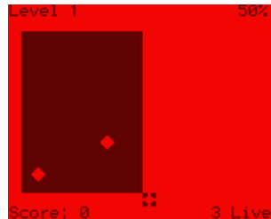
Figure 10.24: Xobox
