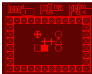
Figure 10.11: pegbox
