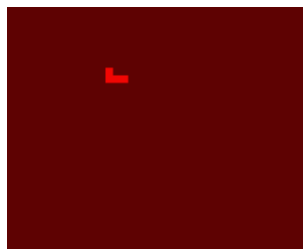
Figure 10.16: Snake
