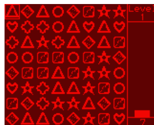
Figure 10.8: Jewels
