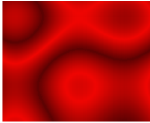
Figure 10.33: Plasma
