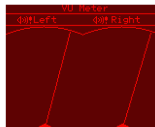
Figure 10.36: VU-Meter
