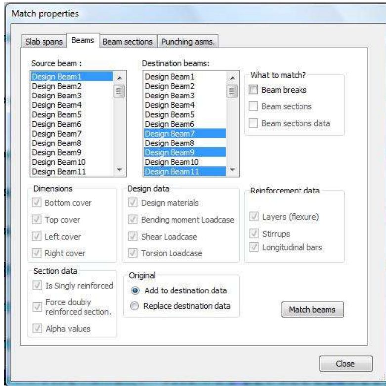
Similar beams are matched with the same reinforcement
