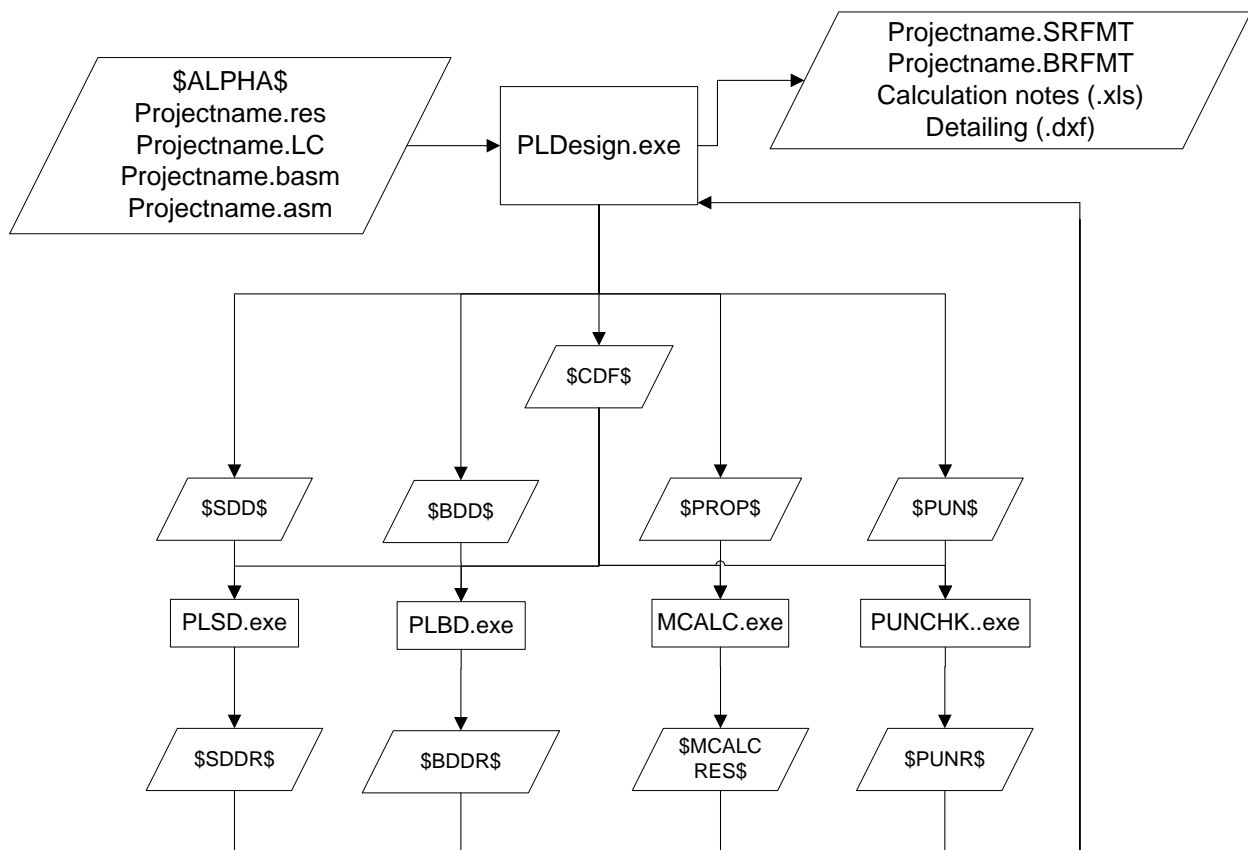
PLDesign operation diagram
