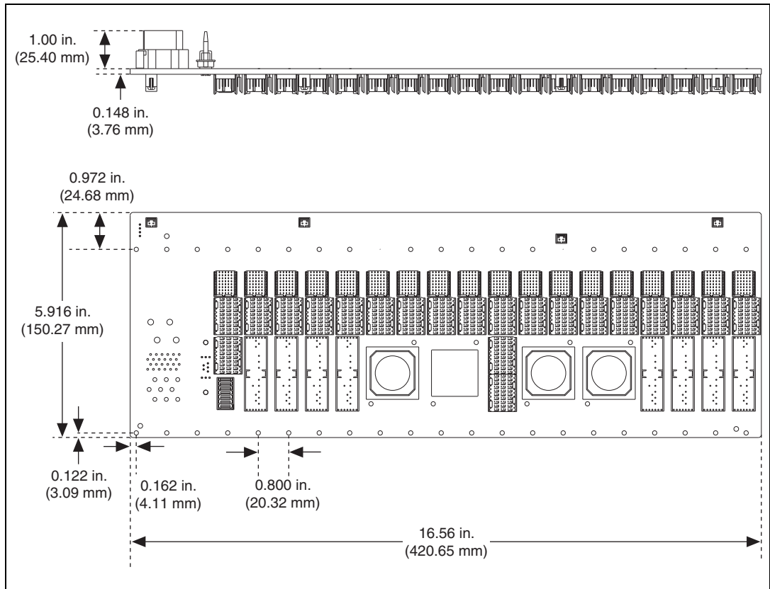
Figure 8. Dimensions
