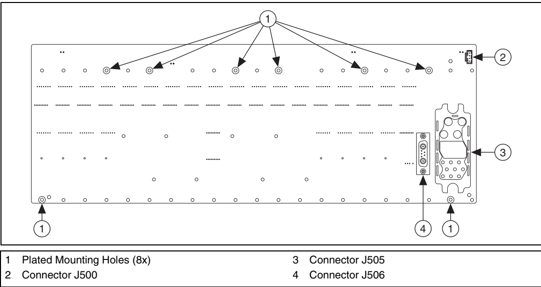
Figure 10. Backplane Power, J500, and CLK10 Connectors
