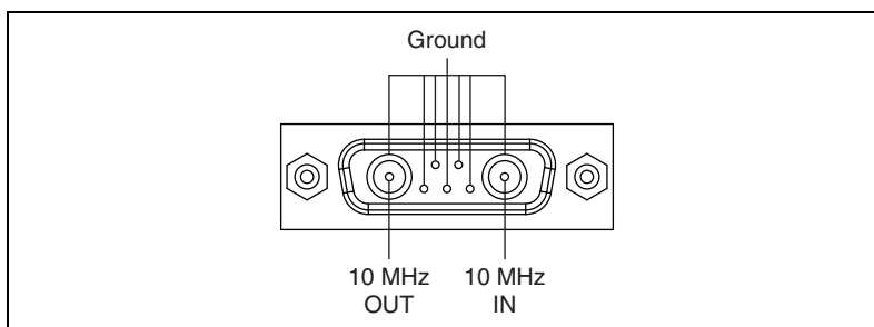
Figure 11. J506 Connector
