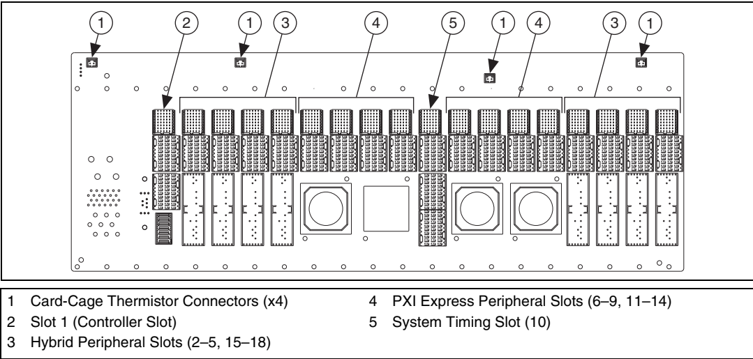
Figure 9. PXI Connectors
