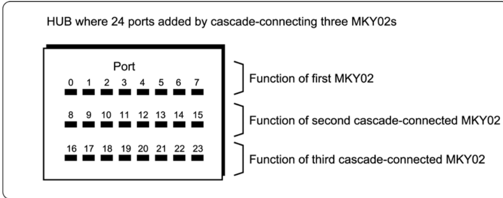
Fig. 1.9 Adding Ports by Cascading MKY02s
