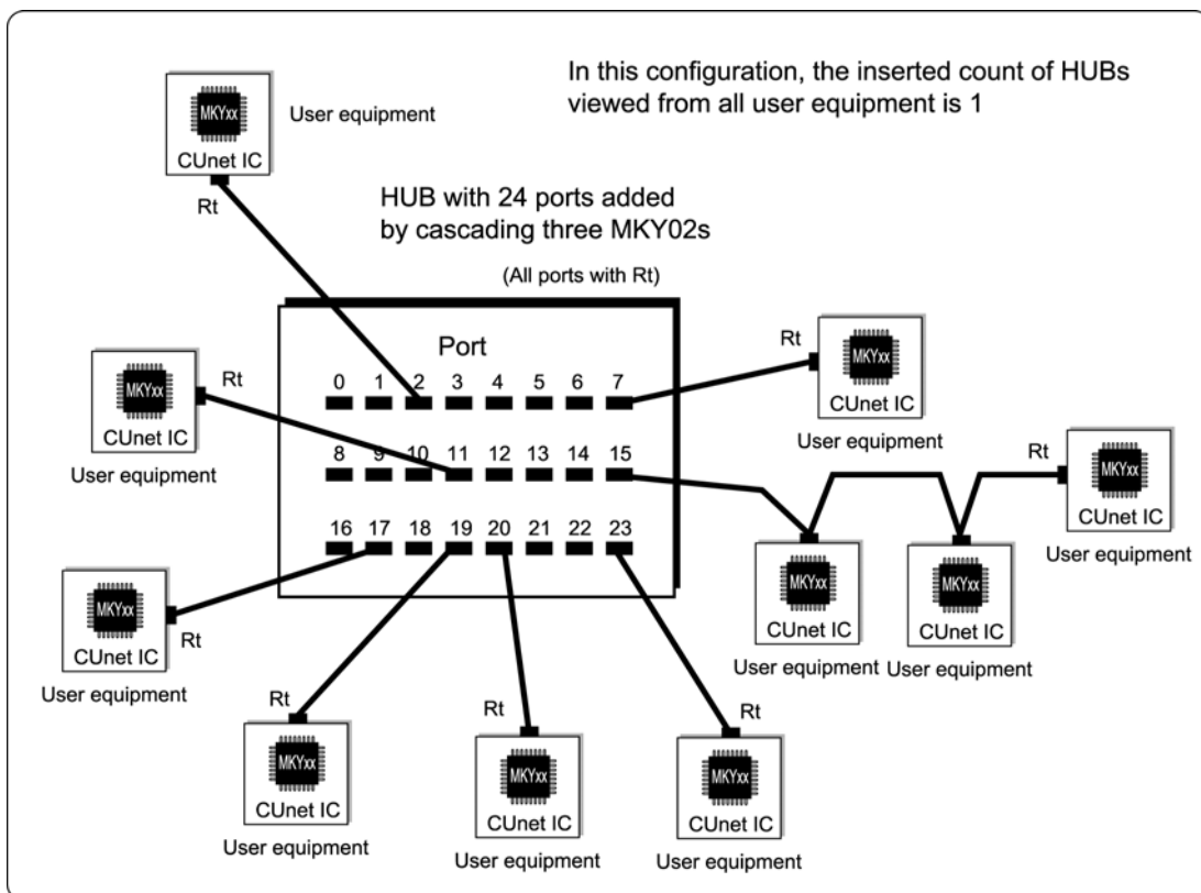
Fig. 1.10 Number of Inserted HUBs with Added Ports
