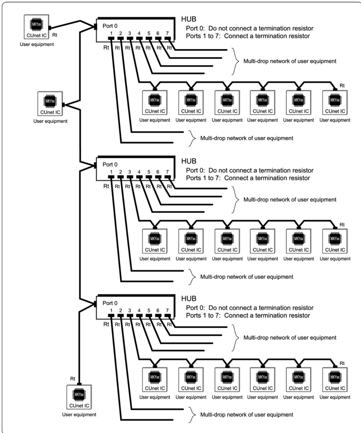
Fig. 1.8 HUB in Intermediate Position of Multi-drop Network
