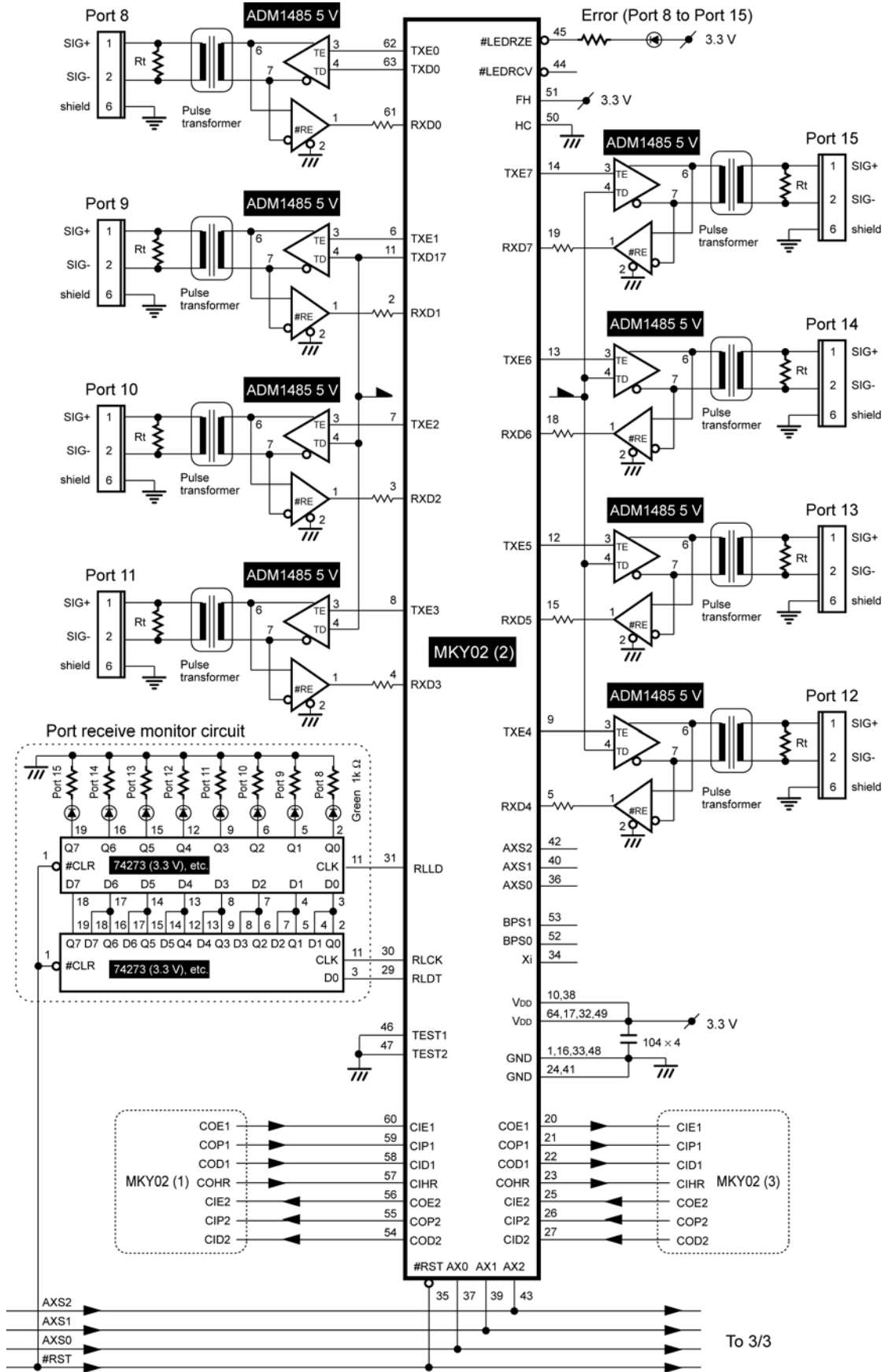
Fig. 4.10 Example Circuit for HUB with 24 Ports (2/3)
