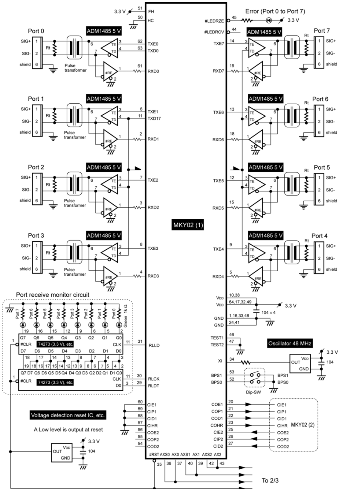
Fig. 4.10 Example Circuit for HUB with 24 Ports (1/3)
