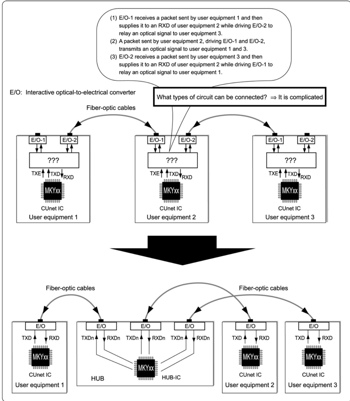
Fig. 1.6 Connection of Fiber-optic Cables
