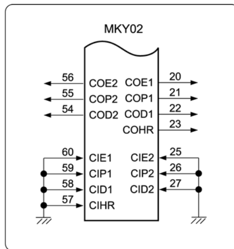
Fig. 3.15 Handling of Cascade Connection Pins
