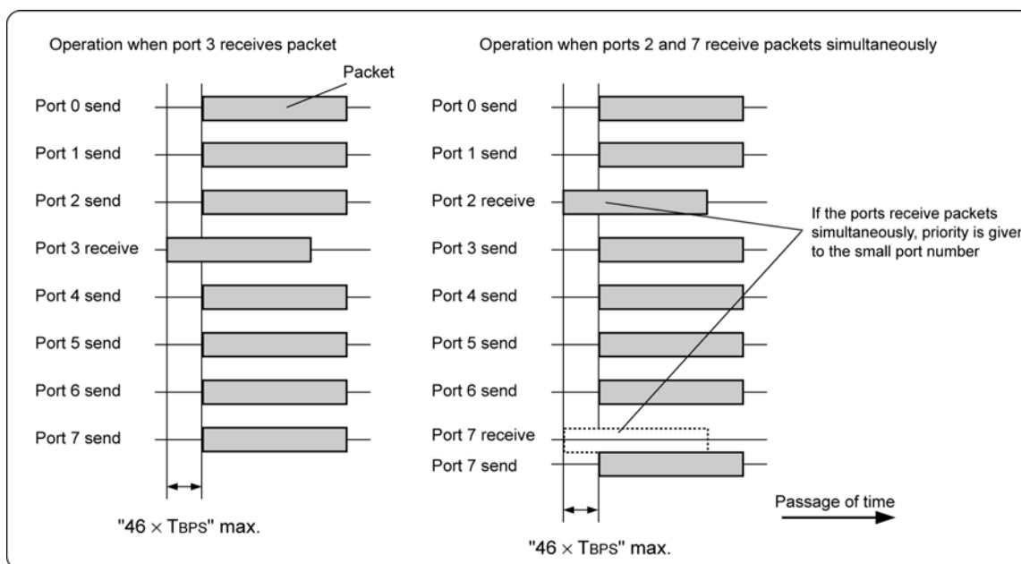
Fig. 1.11 MKY02 Operating Principles
