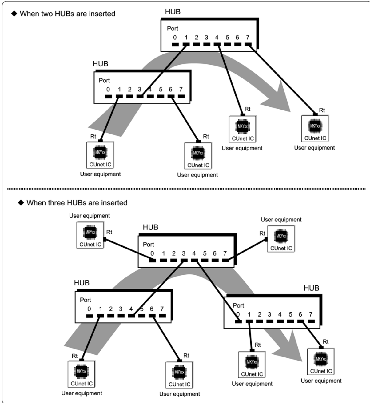
Fig. 1.7 Basic Connection and Number of Inserted HUBs
