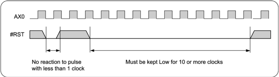
Fig. 3.4 Hardware Reset
