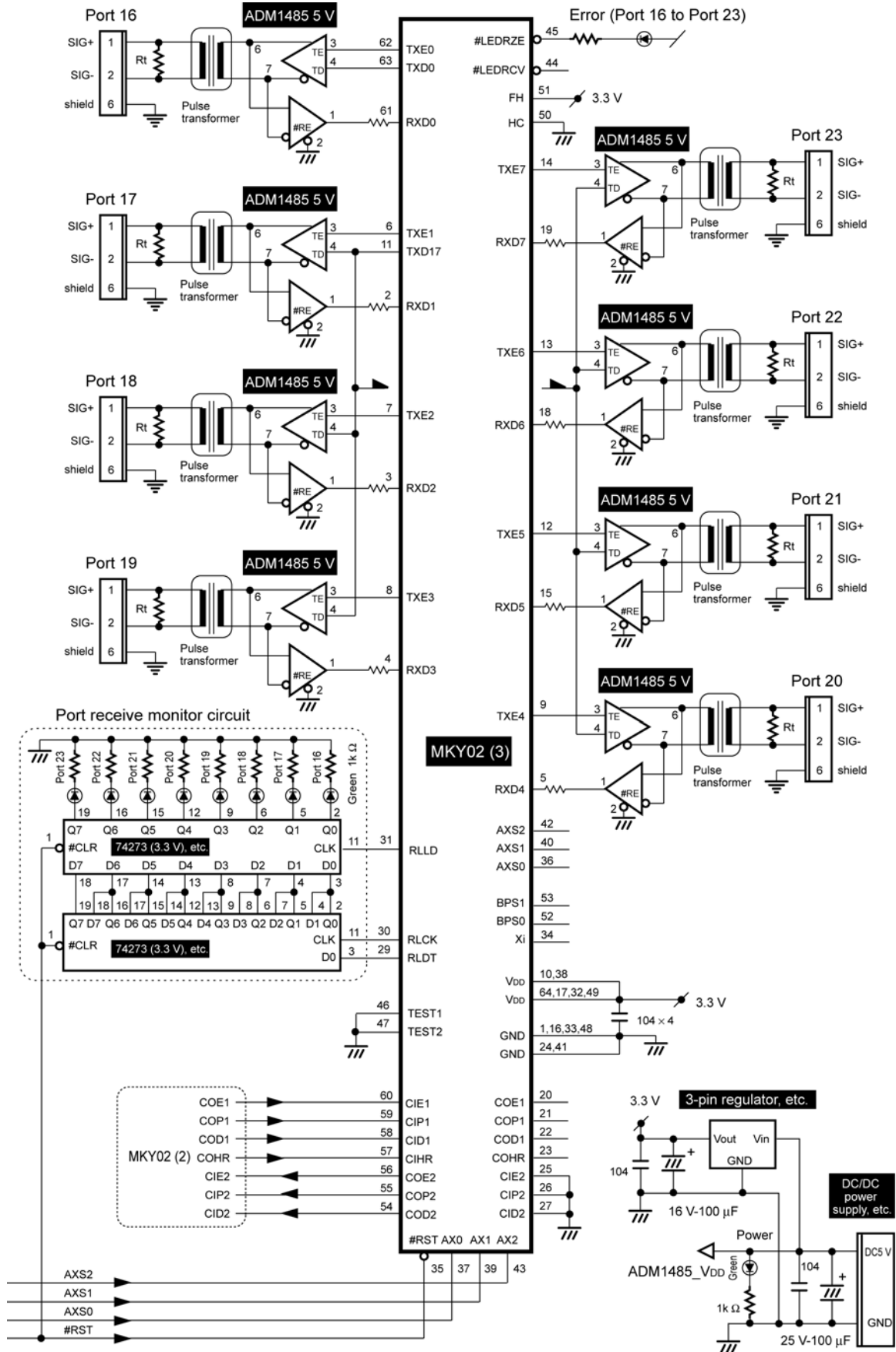
Fig. 4.10 Example Circuit for HUB with 24 Ports (3/3)
