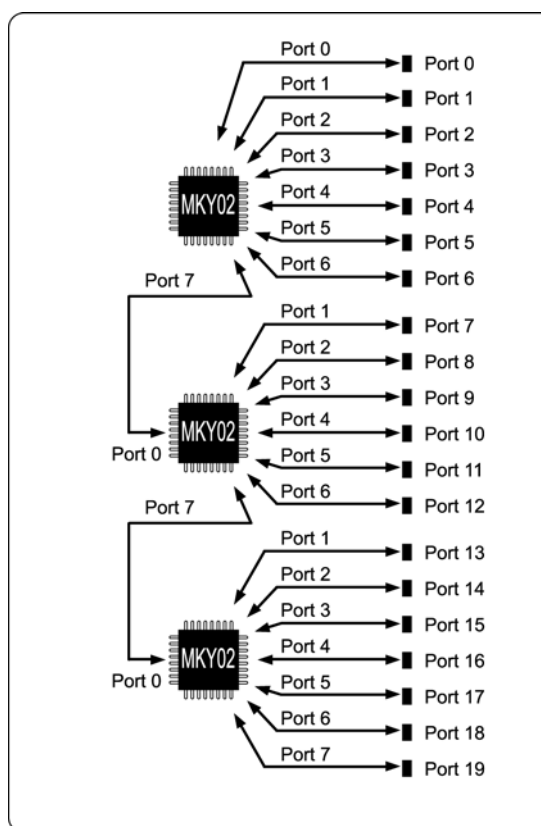
Fig. 4.1 Addition of Three-stacked Ports
