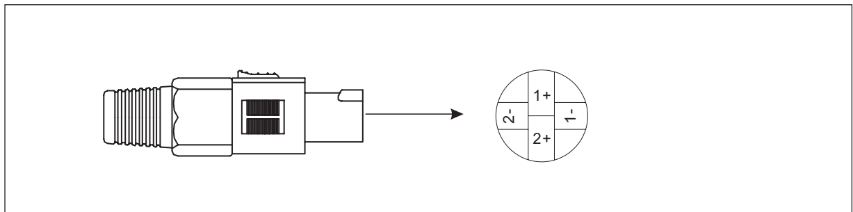
Speakon connector
