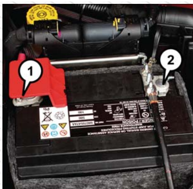
Battery Posts
