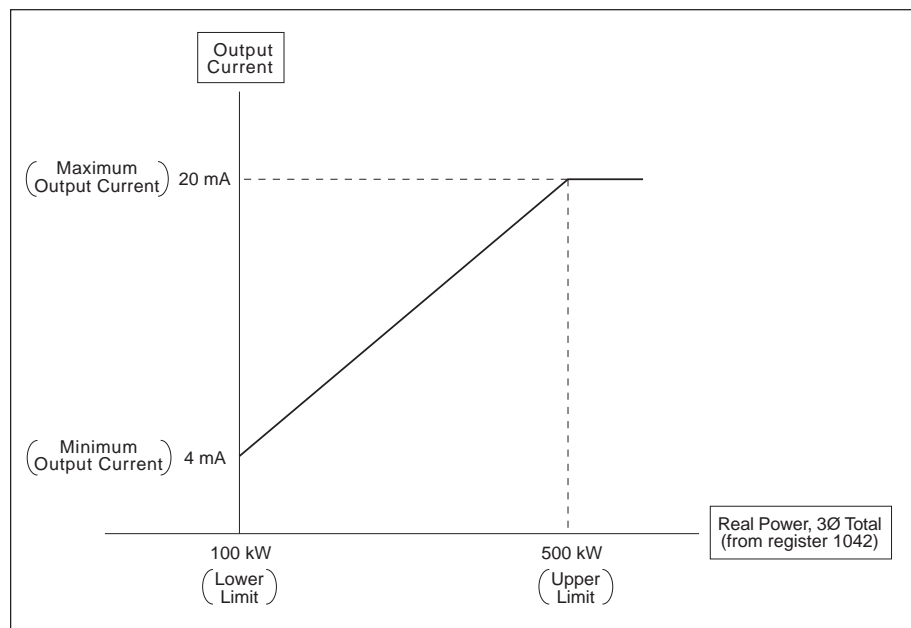
Figure 3-5: Analog output example
