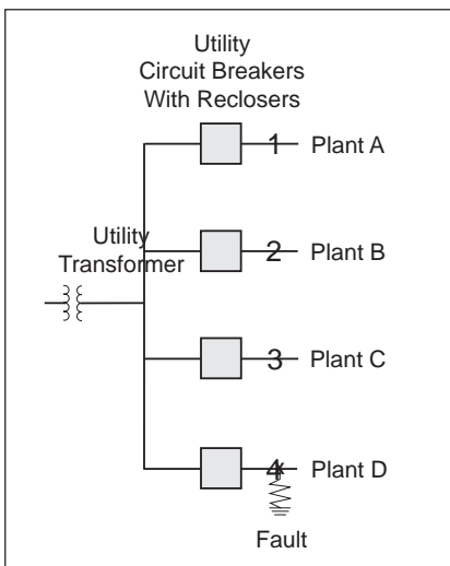
Figure 7-1: A fault near plant D that is cleared by the utility circuit breaker can still affect plants A, B, and C, resulting in a voltage sag
