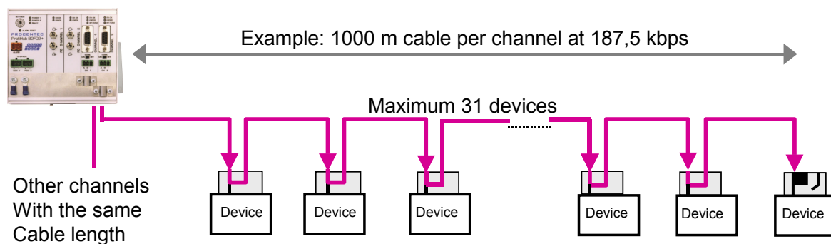
Fig. 6 - Cable lengths for PROFIBUS DP
