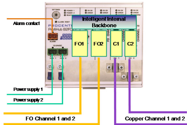
Fig. 2 - ProfiHub connections
