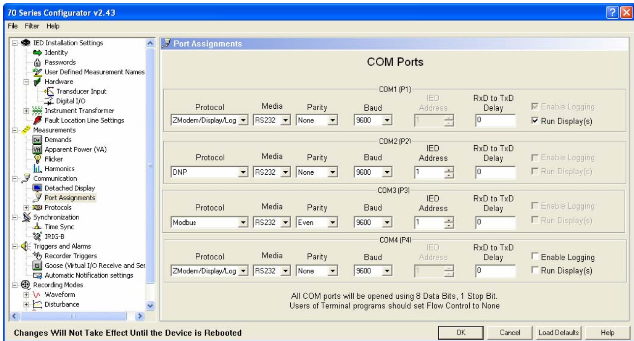
Figure 3 – Configurator Communication/Port Assignments Folder
