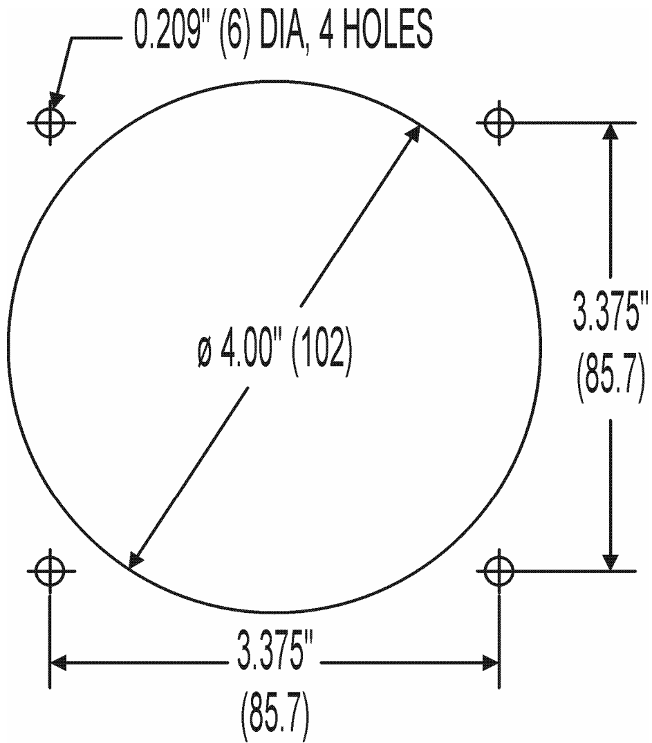
Figure 2 - Panel Cutout Dimensions
