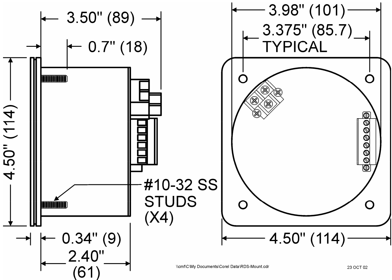
Figure 1 – Instrument Dimensions
