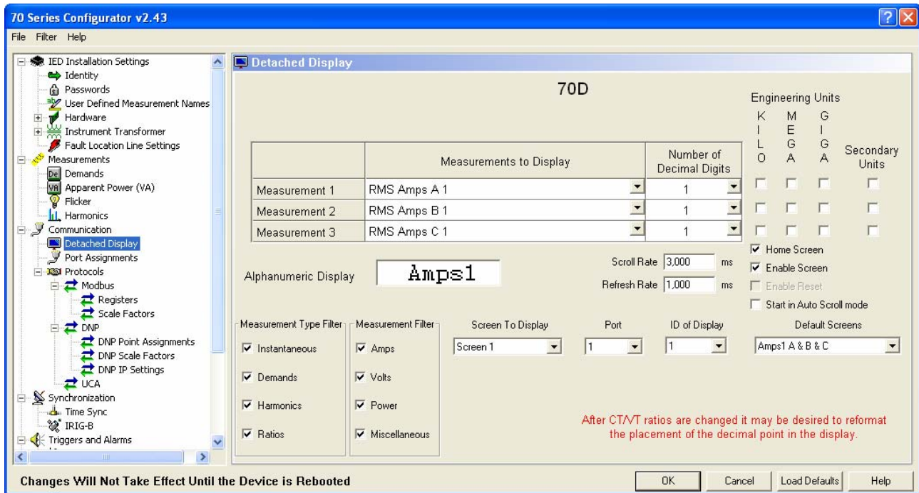
Figure 4 – Configurator Communication/Detached Display Folder
