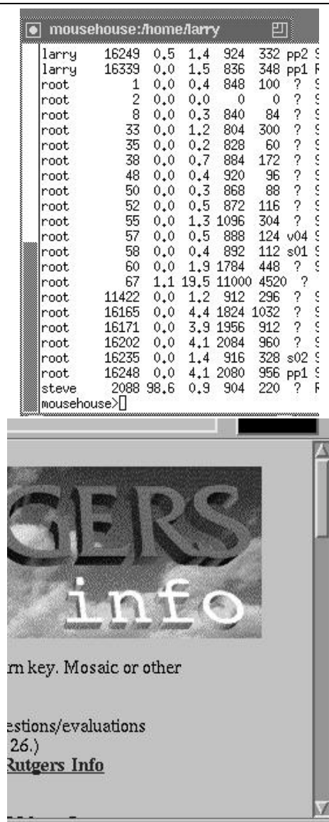
Figure 5.4 An Athena-type scroll bar is visible on the left of this xterm window. Next to it, a Motif-type scroll bar is visible on the netscape window.
