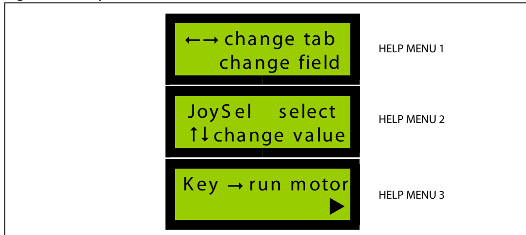
Figure 18. Help menu
